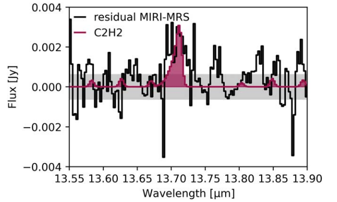
Figure 5. Residual observed emission after subtracting the continuum, H 2 O, OH, CO 2 , and HCN best-fit models (black). The best-fit model for C 2 H 2 is overlaid in magenta. Gray shading indicates the 1 \sigma rms noise level calculated for the continuum-subtracted spectrum for 14.74–14.755 \mu\text{m} . The emission attributed to C 2 H 2 is of the same order as nearby residual emission.
