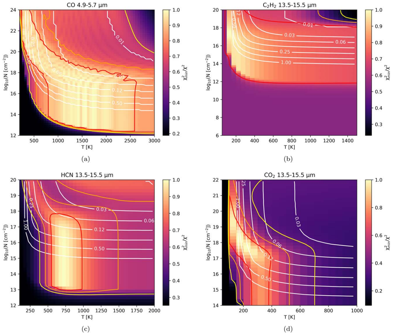
Figure 10. \chi^2 maps for the slab model fits to CO, C 2 H 2 , HCN, and CO 2 . The color map shows \chi_{\min}^2/\chi^2 such that the best fit is given a value of one. The red, orange, and yellow contours give the 1\sigma , 2\sigma , and 3\sigma uncertainty levels, respectively, for two degrees of freedom. The white contours show the best-fit emitting radius, with labels in units of au.
