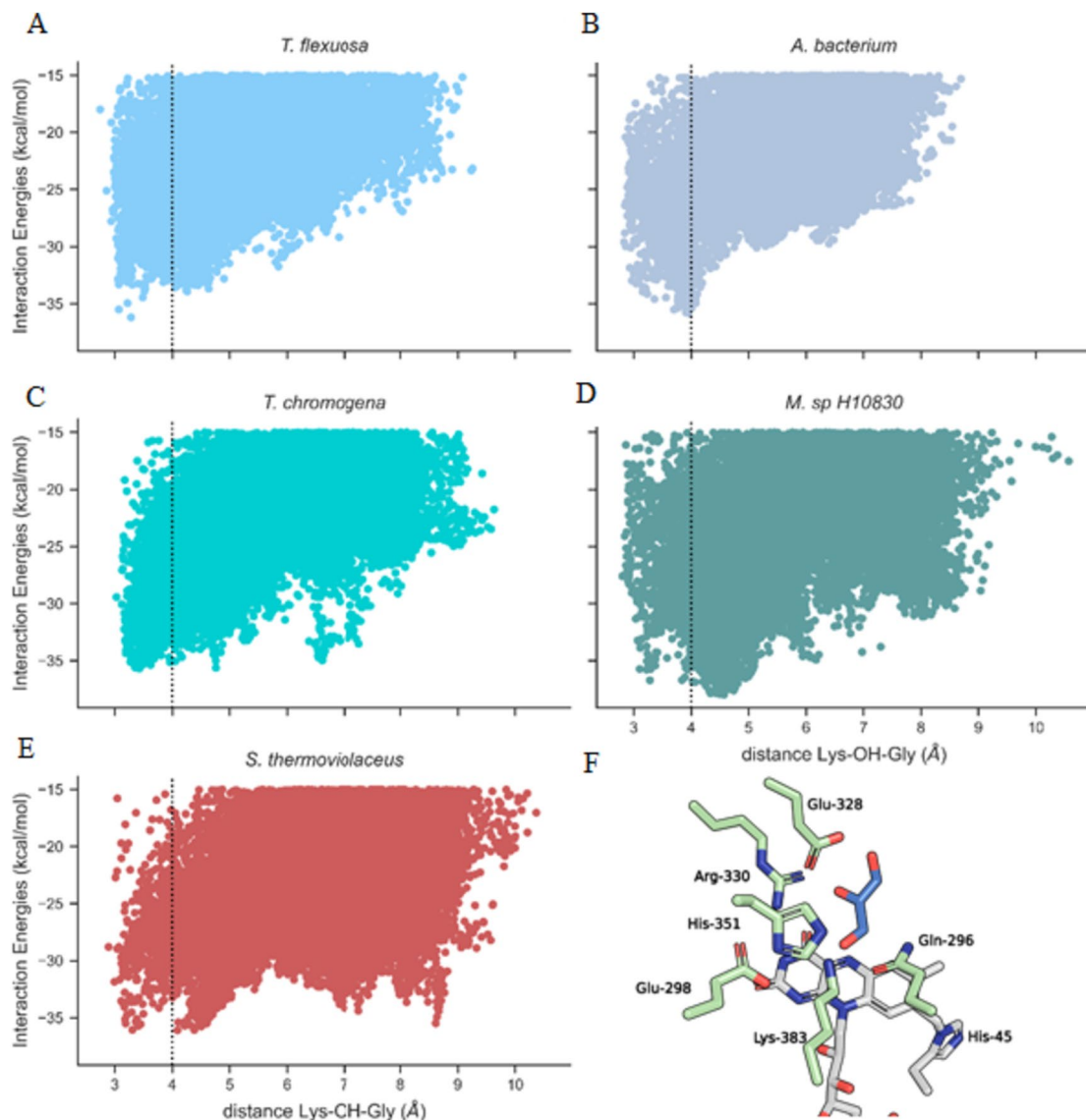
Fig. 1 PELE simulation results using glycerol as the substrate ligand. The X-axis represents the distance in angstroms ( \text{\AA} ) between the catalytic lysine residue and the hydroxyl group of the substrate. The Y-axis represents the interaction energies measured in kilocalories per mole (kcal/mol). The panels are labeled as follows: A AldO Tf
