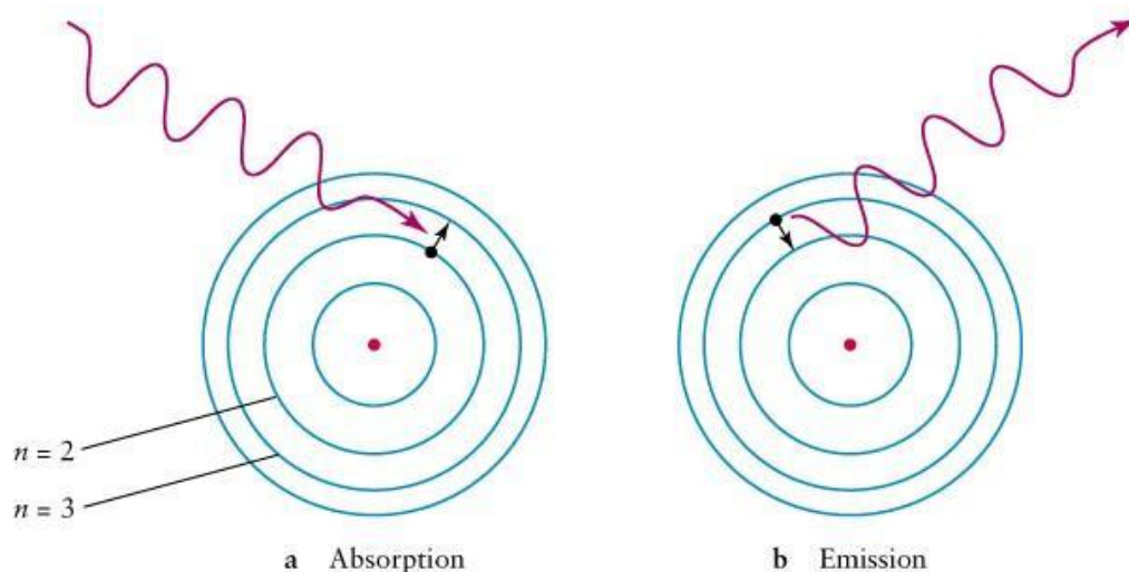
Fig.5(a,b). The graphical meaning of Bohr's postulates.
