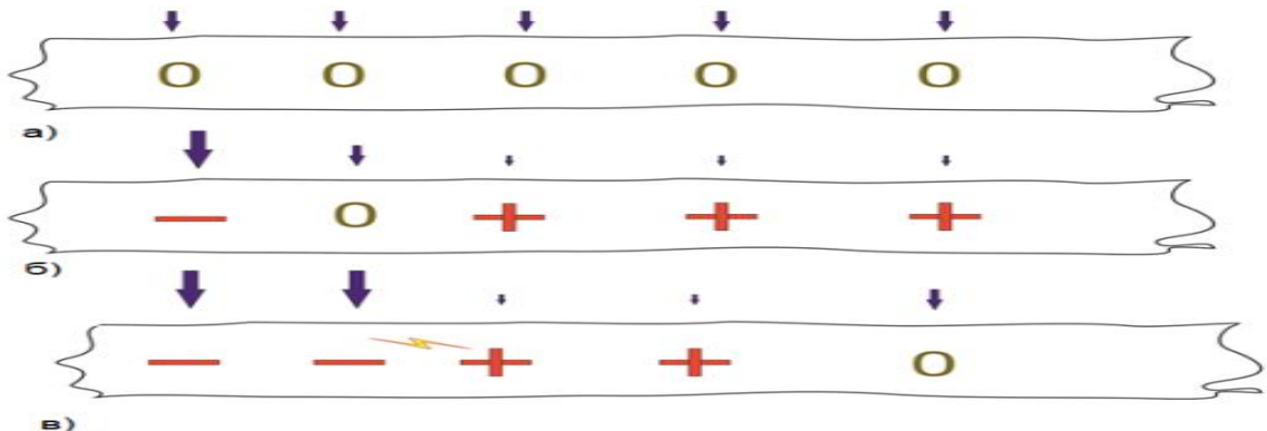
Fig.4. A change in the pressure parameter leads to the appearance of a charge and a force field.
