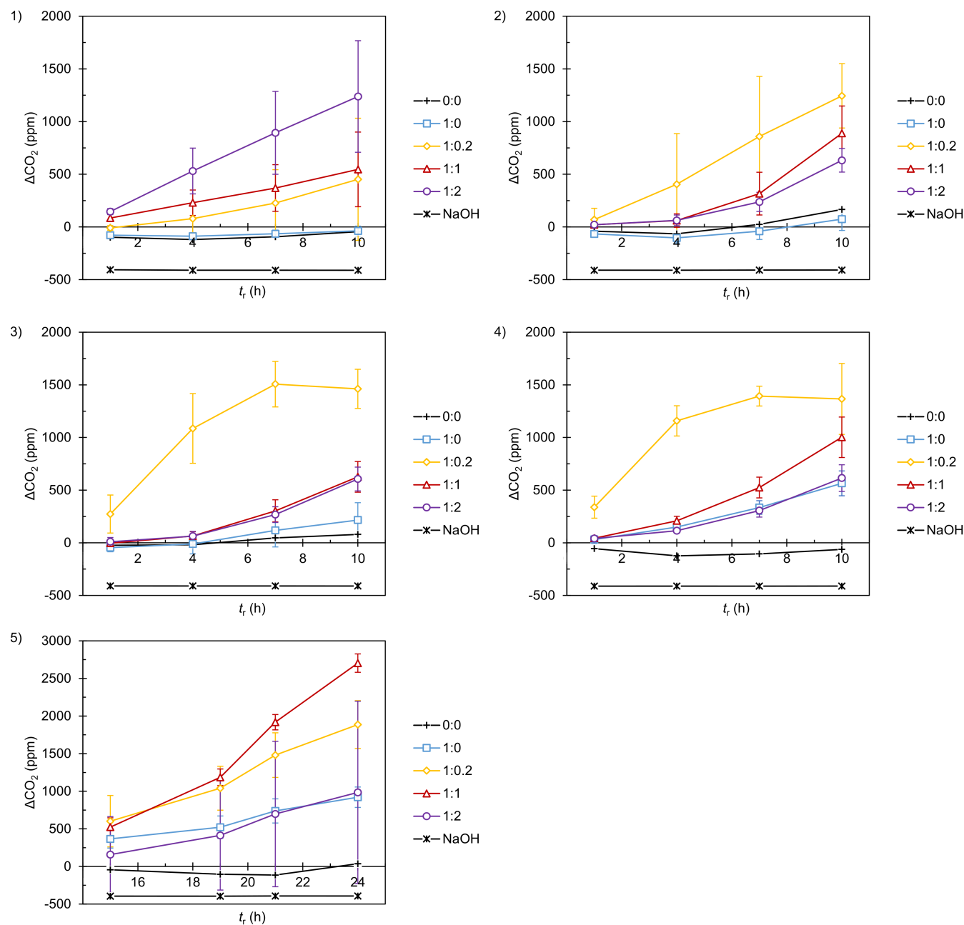
FIGURE 4 Comparison of \text{CO}_2 (ppm) evolution in vial headspace during MICP over 10 h incubation for solution treatments: distilled water (0:0); urea-to-calcium molar ratio of 1:0; 1:0.2; 1:1; 1:2; and distilled water with adjusted pH of 9.5 with NaOH (NaOH), over five incubation periods (1–5). Incubation time (1) to (4) t = 0 –10 h and of 5) t = 14 h to 24 h. Four gas measurements were performed during every 10 h incubation period at t = 1, 3, 7 and 10 h since vial closure. Gas concentrations are the difference between measured average concentrations and atmospheric concentration at t = 0 . Markers and error bars indicate the average and standard deviation of three replicate samples.
