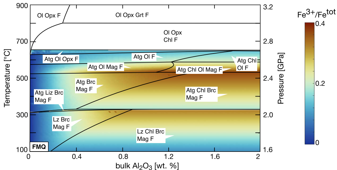
Fig. 9. Compositional diagram showing the effect of bulk \text{Al}_2\text{O}_3 on the redox potential. The bulk composition (97 wt. % lizardite + 3 wt. % magnetite, supporting information B-3) changes from 0 to 2 wt. % \text{Al}_2\text{O}_3 . The system is buffered at FMQ. Colour code shows the lizardite and antigorite \text{Fe}^{3+}/\text{Fe}^{\text{tot}} ratio.
