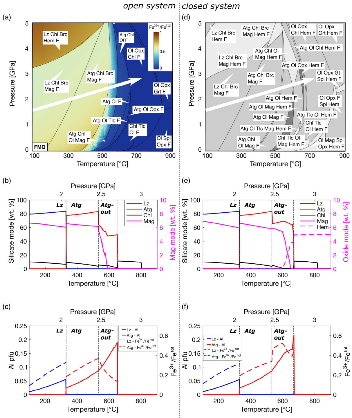
Fig. 8. (a) The lizardite to antigorite phase transformation calculated with the new solution models implemented in Perple_X for the bulk composition 97 wt. % lizardite + 3 wt. % magnetite (supporting information B-3). The P-T pseudosection is buffered at FMQ. The colour code indicates the bulk Fe^{3+}/Fe^{tot} ratio. The white arrow marks the P-T path used in b and c. (b) Phase modes of the sheet silicates lizardite, antigorite and chlorite, and oxide along the P-T path from a. Indicated are also major reactions such as the lizardite to antigorite phase transformation and the antigorite-out reaction. (c) The Al and Fe^{3+}/Fe^{tot} ratio of lizardite and antigorite along the P-T path from a. (d) to (f) The same calculation for a closed system, i.e., with a fixed O_2 content of 0.5 wt. %, giving rise to a bulk Fe^{3+}/Fe^{tot} content of 0.55.
