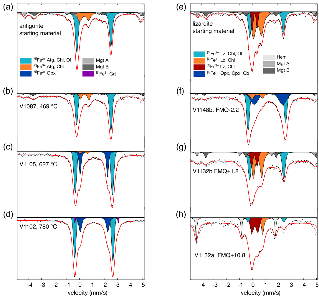
Fig. 5. Room temperature Mössbauer absorption spectra of representative samples. (a) The antigorite serpentinite starting material has ferric Fe only on the octahedral site. (b to d) With increasing temperature, magnetite and serpentine disappear. Increasing proportions of olivine, orthopyroxene and garnet are observed. (e) The lizardite serpentinite starting material also contains tetrahedral ferric Fe. (f to h) With increasing f(\text{O}_2) , the \text{Fe}^{3+}/\text{Fe}^{\text{tot}} ratio of lizardite increases. Note the broad peaks in experiment V1148b most probably indicating a poorly crystallised carbonate and olivine–pyroxene intergrowth.
