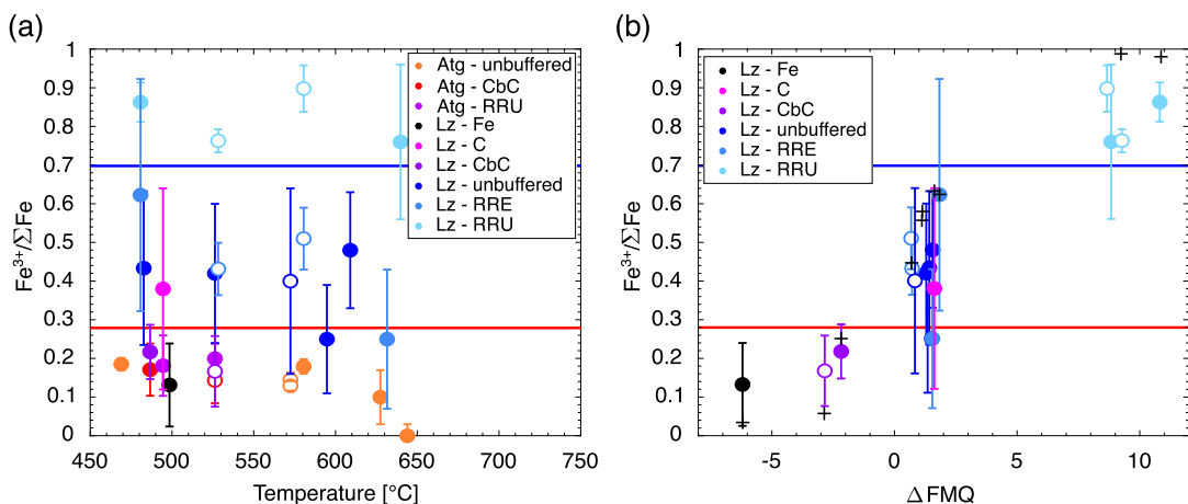
Fig. 6. \text{Fe}^{3+}/\text{Fe}^{\text{tot}} ratio of serpentinite in experimental run products. (a) The \text{Fe}^{3+}/\text{Fe}^{\text{tot}} ratio in antigorite decreases only above 600 °C and is independent of the pressure and the buffer component added. Lizardite shows a decrease with increasing temperature at a fixed f(\text{O}_2) over the entire experimental temperature range. (b) The \text{Fe}^{3+}/\text{Fe}^{\text{tot}} ratio of lizardite is also strongly dependent on the f(\text{O}_2) . Note that the experiment at \Delta\text{FMQ} < -5 was buffered with Fe metal and probably did not fully equilibrate. The \text{Fe}^{3+}/\text{Fe}^{\text{tot}} ratio in this experiment might thus be even lower. The black crosses represent values obtained with the new solid solution models of this study for the experimental conditions.
