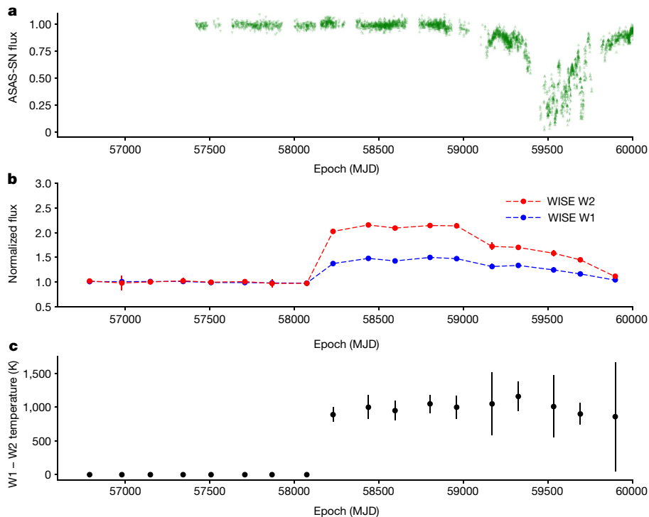
Fig. 1 | Optical and infrared photometry of ASASSN-21qj. a , Normalized optical photometry from ASAS-SN in the V-band and the g'-band. b , Fractional flux increase in brightness of ASASSN-21qj in both the W1 and W2 bands, for which a value of 1.0 represents the stellar contribution alone. c , Calculated
