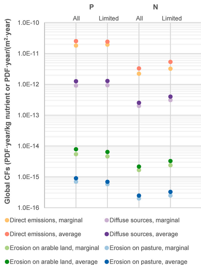
Fig. 3. Globally aggregated characterization factors (CFs) for P and N impacts on global species richness. The unit of CFs for direct and diffuse emissions is PDF-year/kg nutrient, where the nutrient represents P or N, while the unit of CFs for erosion is PDF-year/(m 2 -year). CFs consider either all regions (All) or only regions limited by the respective nutrient (Limited).
