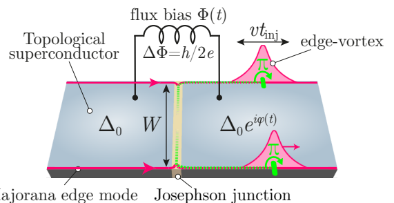
FIG. 1. Edge-vortex injector [10], consisting of a Josephson junction in a topological superconductor with copropagating chiral edge modes. An h/2e flux increment injects a pair of edge vortices on opposite edges with a protected fermion parity. The corresponding phase domain wall is represented by green lines. The adiabatic description of the injection process assumes that the injection time t_{\text{inj}} = (2\pi\xi_J/W)(d\varphi/dt)^{-1} is long compared to the propagation time W/v along the junction. In this work we relax that assumption to simulate a device (Fig. 2) in which these dynamically injected edge vortices are braided with Abrikosov bulk vortices.
