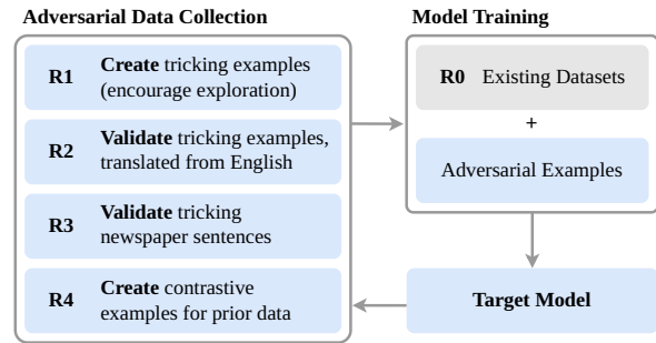
Figure 1: We use four rounds of dynamic adversarial data collection (Kiela et al., 2021) to improve a German hate speech classifier. We start with a target model trained on existing datasets. Then, in each round (R1-R4), annotators try to trick the target model using a different method. After each round, we train a new target model including the new adversarial examples.
