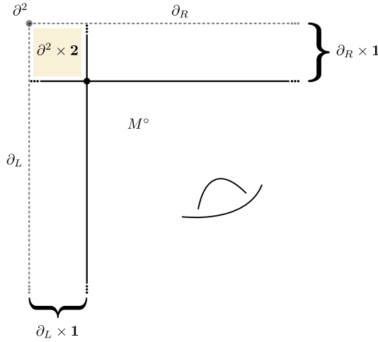
Figure 7.4: Construction of \overline{\mathfrak{M}} \rightarrow \mathfrak{M}^! induced by M with connected boundary \partial = \partial_L \cup \partial^2 \cup \partial_R , with \partial^2 denoting the corner.
