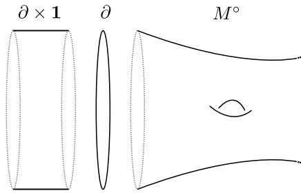
Figure 7.3: The three strata of the linked collar of a manifold with connected boundary.
