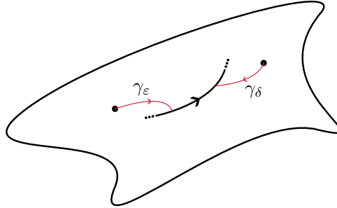
Figure 7.1: A general closed linked path as in (7.1.9).
