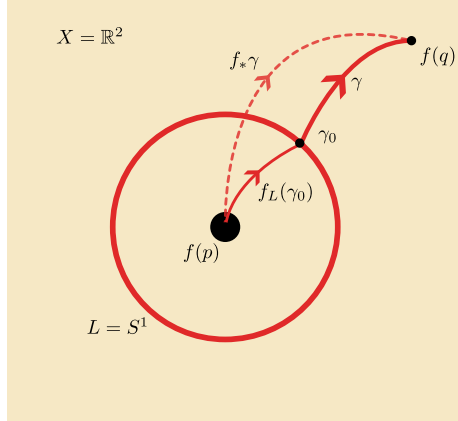
Figure 7.2: The proof of Proposition 7.1.10 for (M \rightarrow \mathfrak{P}) = (\{0\} \leftarrow S^1 \hookrightarrow \mathbf{R}^2 \setminus \{0\}) and N = X = \mathbf{R}^2 , with f ‘the identity’; cf. Remark 7.1.12.
