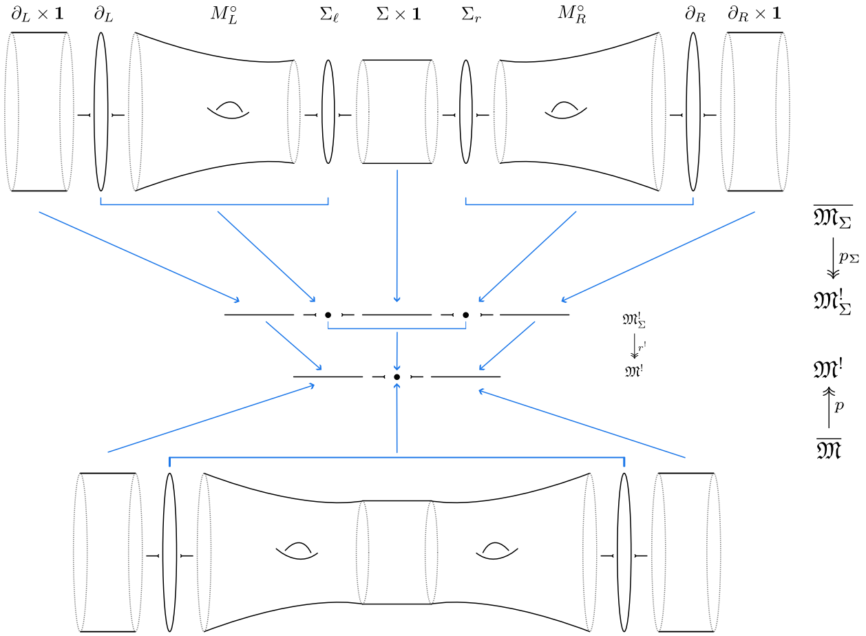
Figure 7.6: The cutting-and-gluing square (7.5.6) using Notation 7.2.16; \bar{r}: \overline{\mathfrak{M}}_\Sigma \rightarrow \overline{\mathfrak{M}} omitted.
