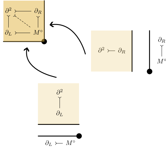
Figure 7.5: The assembly of a corner: \mathfrak{M}^1 from depth-1 data.
