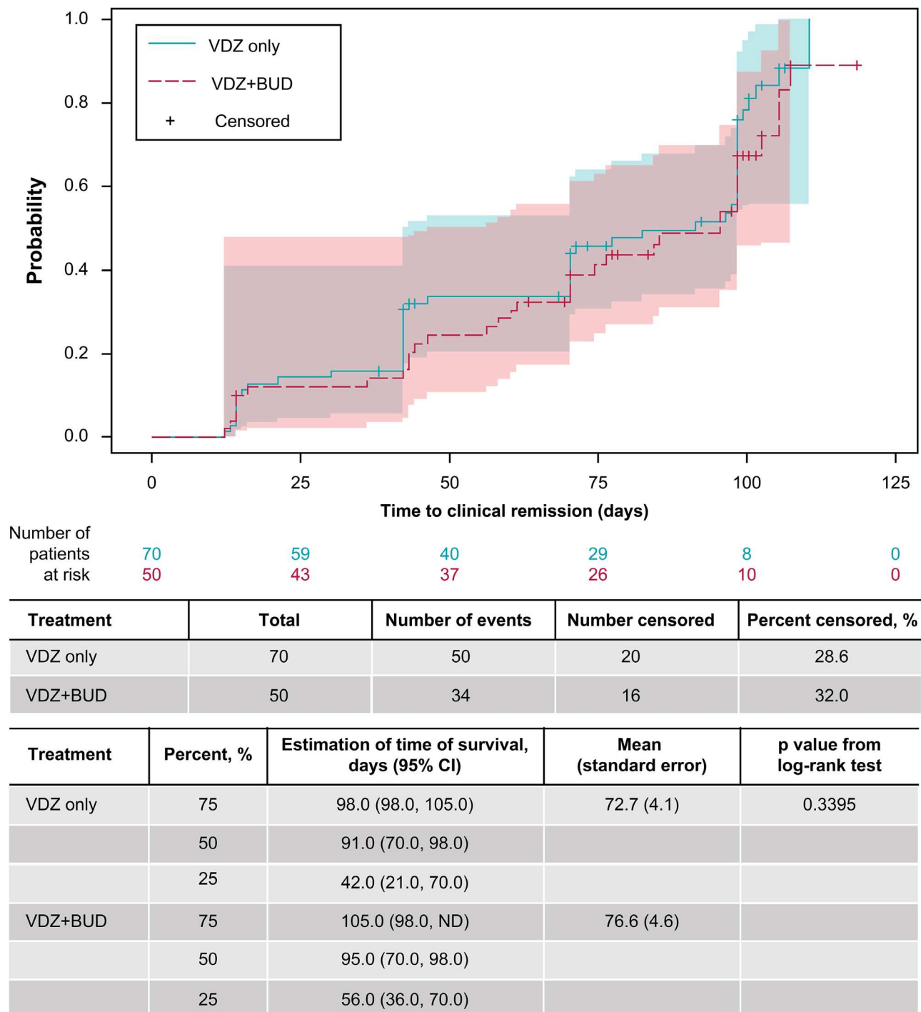
Fig. 4 Time to clinical remission (days) according to patient-reported symptoms: APS ( \leq 1 ) and LSF ( \leq 3 ). PRO-2 is estimated as a sum of the weighted averages of APS and LSF. APS=abdominal pain score; BUD=budesonide; CI=confidence interval; LSF=loose stool frequency; VDZ=vedolizumab
