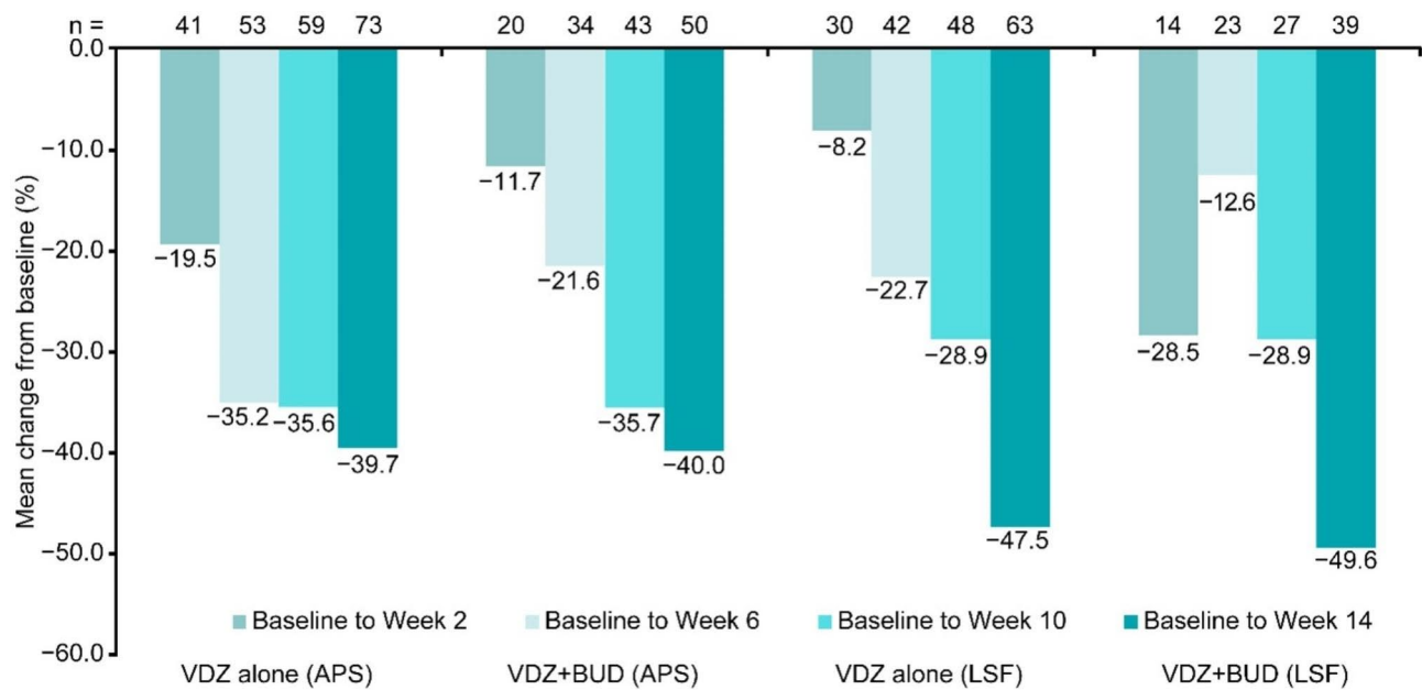
Fig. 3 Mean percentage change in APS and LSF from baseline. APS=abdominal pain score; BUD=budesonide; LSF=loose stool frequency; VDZ=vedolizumab
