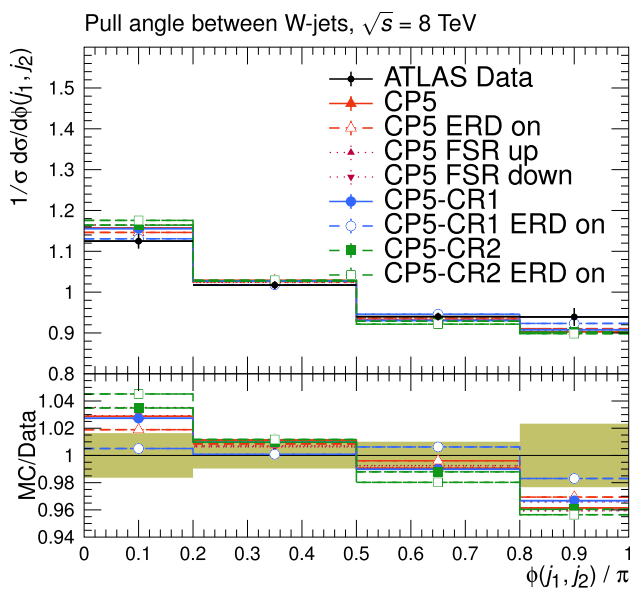
Fig. 20 Normalised \bar{t} differential cross section for the pull angle between jets from the W boson in top quark decays, calculated from the charged constituents of the jets, measured by the ATLAS experiment using \sqrt{s} = 8 TeV data [58] to investigate colour flow. The coloured band and error bars on the data points represent the total experimental uncertainty in the data
