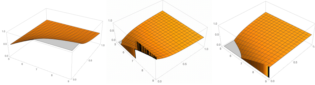
Figure 4: The probability (vertical axis) of the seller keeping the good as a function of c \in [5, 9] and \gamma \in (0, 1) for v = 5 (left), v = 7 (center), and v = 9 (right).
