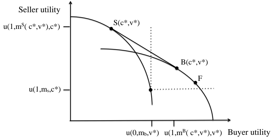
Figure 2: Individually Rational Part of the Pareto Frontier. The Case of Trade at Fixed Price.
