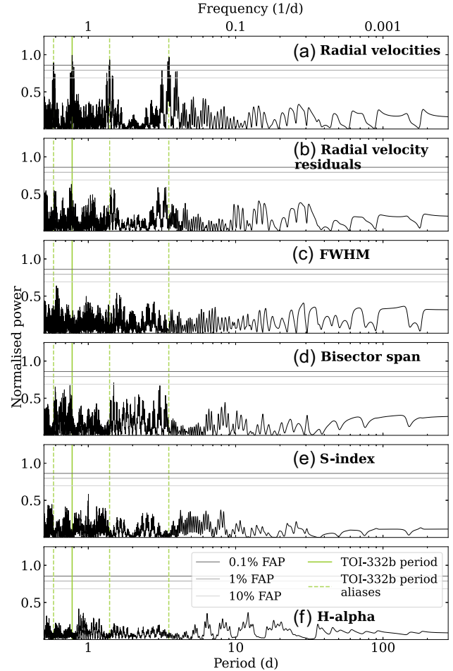
Figure 5. Periodograms for the HARPS data. The expected period of TOI-332 b is denoted by a solid vertical line, with the aliases of this period given as dashed lines. The 0.1, 1, and 10 per cent False Alarm Probabilities (FAPs) are shown as solid horizontal lines. The FAPs are calculated using the approximation from Baluev (2008). From top to bottom: (a) the periodogram for the raw radial velocities with a peak above the 0.1 per cent FAP at the expected planetary period; (b) the periodogram for the RV residuals after the best fit model has been removed, showing no further significant peaks; (c–f) the periodograms for the stellar activity indicators FWHM (c), bisector span (d), s-index (e), and h-alpha (f), with no significant periodicity shown.
