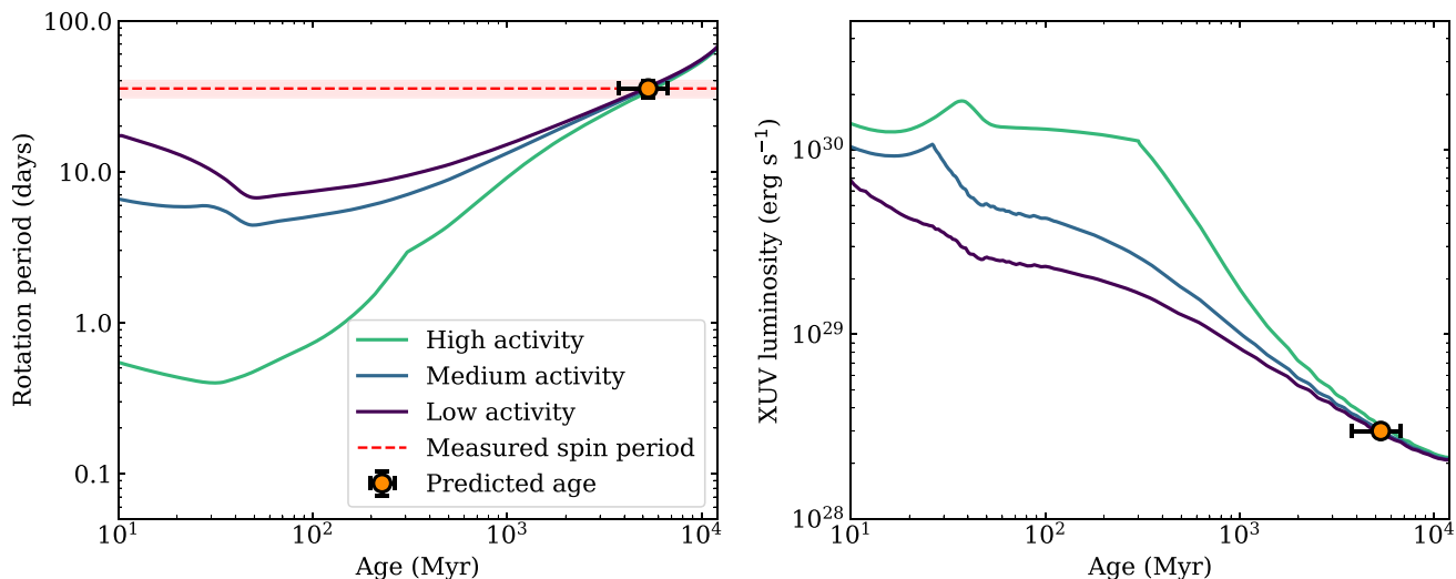
Figure 8. Left panel: plot of rotation period against age showing rotational evolution models by Johnstone, Bartel & Güdel (2021), with high, medium, and low activity tracks for a 0.9 M_{\odot} star. Its measured rotation period is shown as a dashed red line, with the uncertainty as a shaded region. The age estimated with gyrochronology is plotted as an orange circle. Right panel: plot of XUV luminosity against age showing the corresponding XUV evolution tracks to the models on the left panel, as well as the predicted XUV luminosity based on its rotation period. The models were calculated using the methods described in Section 5.3.
