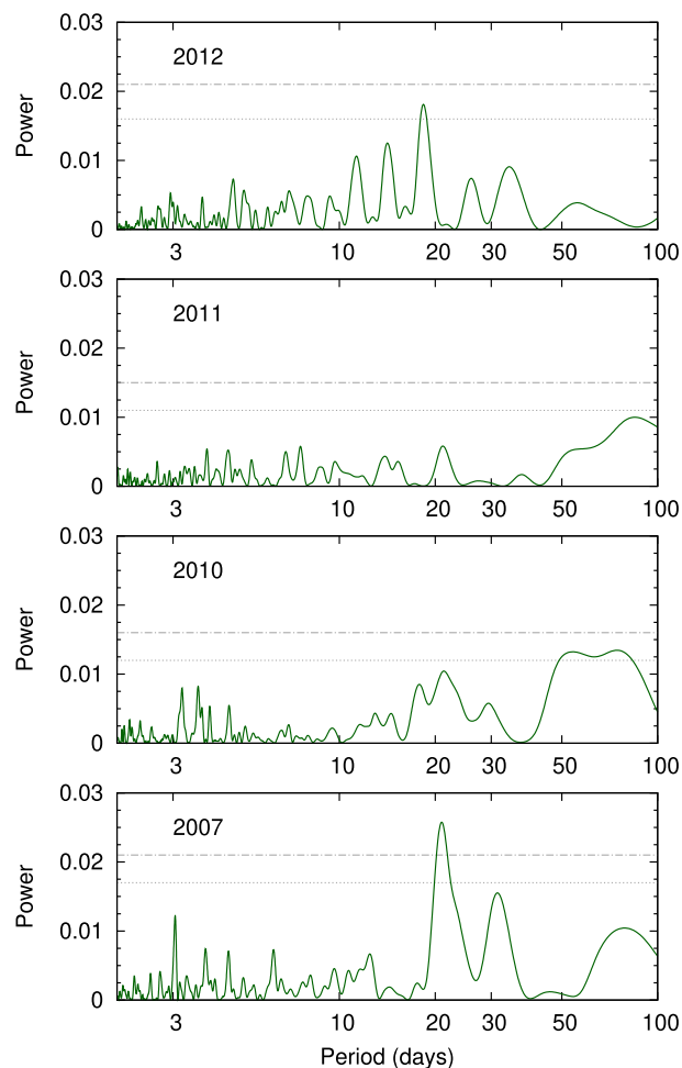
Figure A4. Periodograms of the WASP-South data for TOI-332 from four different years of data. The horizontal lines mark the estimated 10 percent- and 1 percent-likelihood false-alarm levels. A significant periodicity at 20.9 \pm 1.0 d was seen in 2007.
