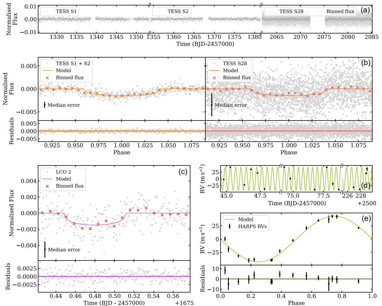
Figure 3. Joint fit model to the TESS , LCO, and HARPS data. (a) TESS PDCSAP light curve for Sectors 1, 2, and 28 (circles), with time given as Barycentric Julian Date (BJD). Sectors 1 and 2 are 30 min cadence data, Sector 28 is 2 min cadence, hence the higher levels of noise in the latter. The Sector 28 data binned to 30 min has been overplotted in dark grey. (b) Phase folded TESS 30 min cadence data (grey circles) from Sectors 1 and 2 (left), and 2 min cadence data from Sector 28 (right). Binned flux (red crosses) and the best fit model (solid line) are overplotted, and the median error on the flux is displayed (one standard deviation, black error bar, bottom left). Residuals when the model is subtracted are shown in the bottom panels. (c) An example of the phase folded LCO data, using the second transit obtained (chronologically) by LCO (the model is fit to all of the LCO transits and the full data can be seen in Appendix Fig. A1). Symbols and model are as in (b), with residuals in the bottom panel. (d–e) The HARPS data (black circles), shown as a time series in (d), and the phase folded data in (e). The model is plotted as in (b), with residuals in the bottom panel.
