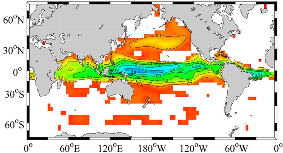
Fig. 7. Pointwise correlation of zonal wind stress between two connected AGCMs. Areas with insignificant correlation are blank. Approximate synchronization was found over the tropical Pacific. There is no significant correlation between the unconnected AGCMs (not shown) (Shen et al. 2016, supporting information).
