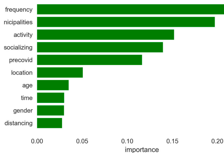
Figure 5. Variable importance of the Xgboost model (author: Jovanka Lili Matić).
