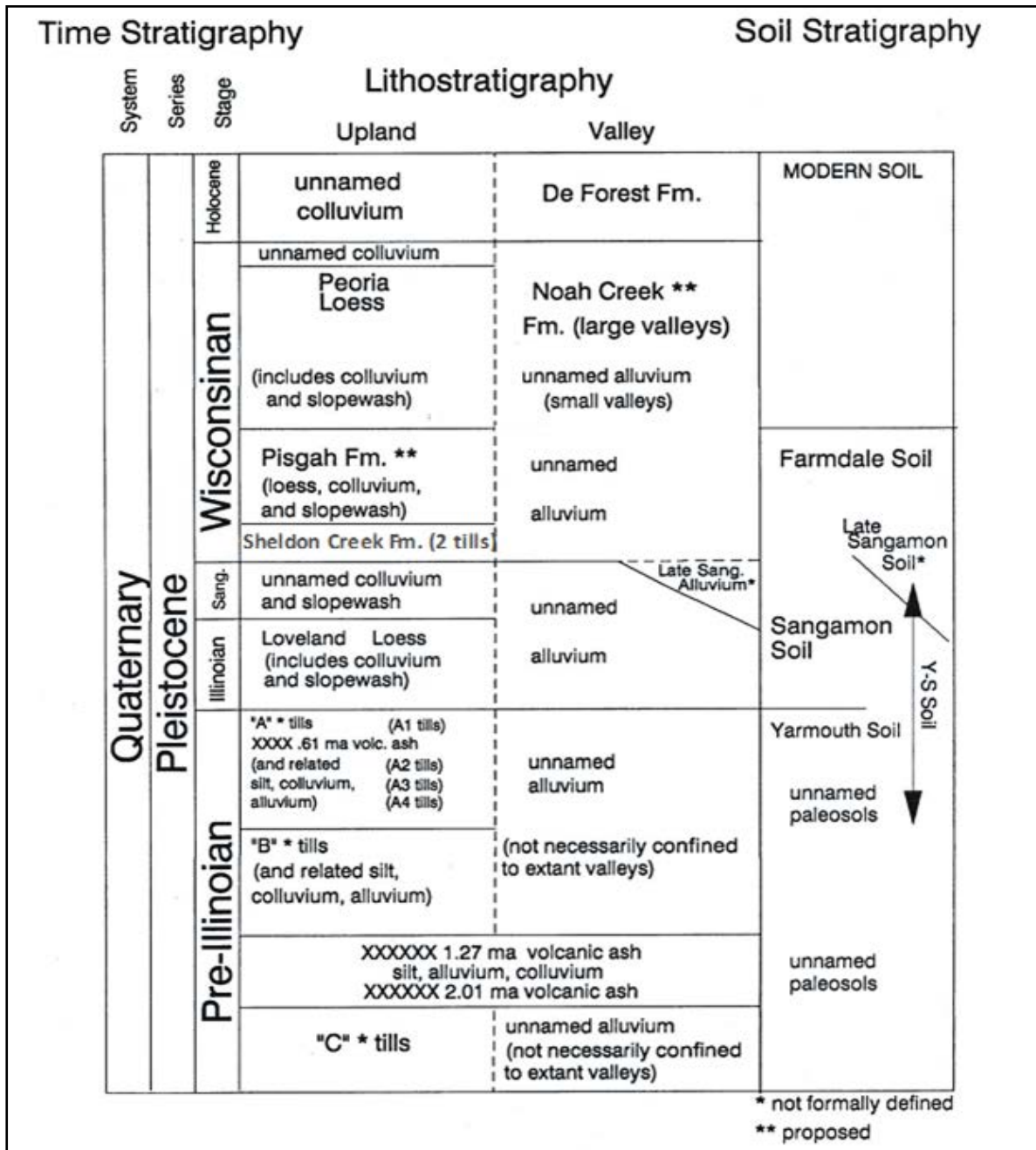
Figure 9. Generalized Pleistocene stratigraphic framework for western Iowa (modified to include north-west Iowa, from Bettis, 1990).
