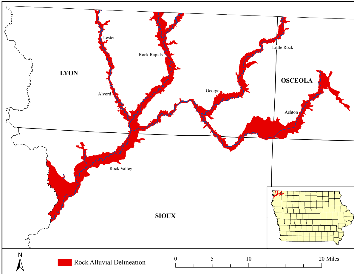
Figure 1. Extent of the Rock River alluvial aquifer study area.
