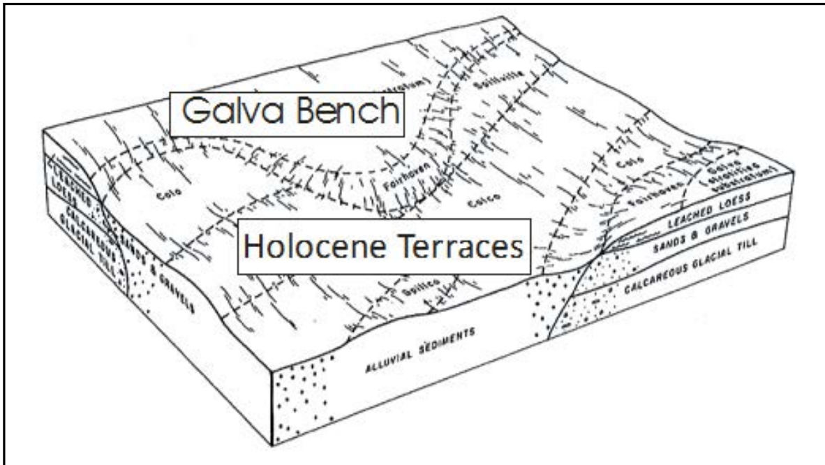
Figure 8. Block diagram representation of soil-geomorphic relationships of Wisconsin-age loess mantled terraces (Galva Bench) to the adjacent uplands in northwest Iowa (modified from Soil Survey of O'Brien County, 1981).
