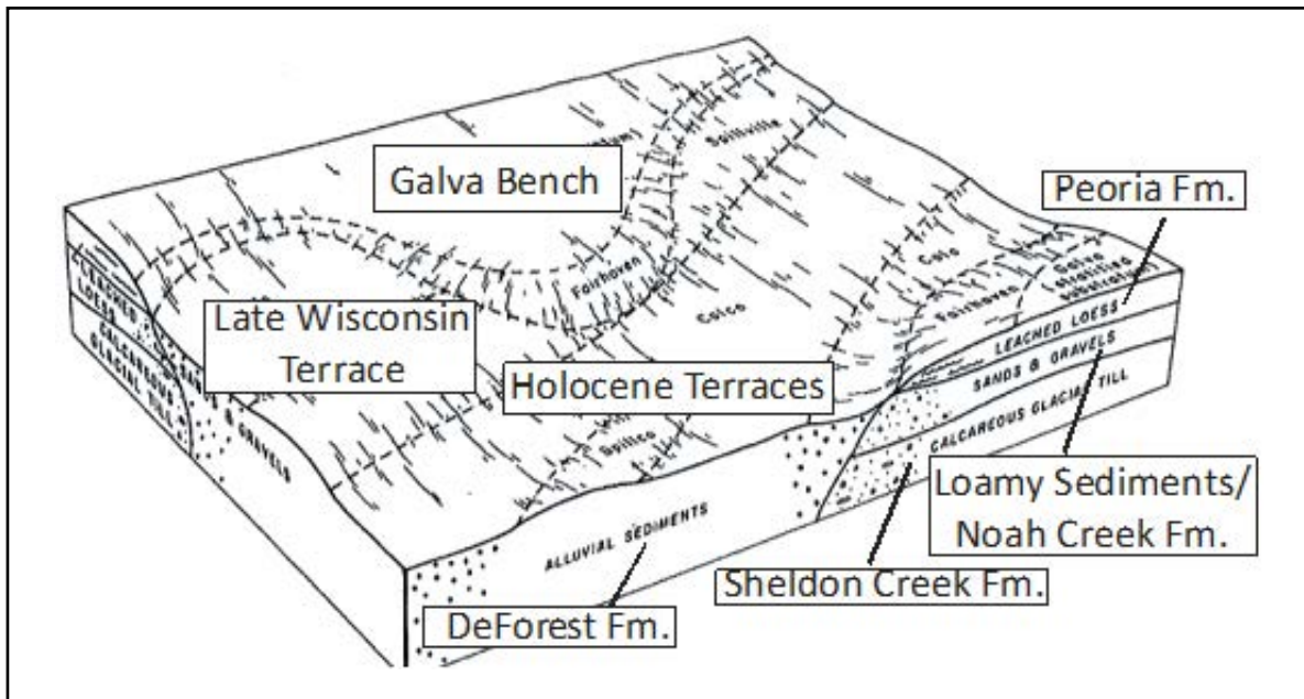
Figure 10. Block diagram representation of soil-geomorphic and underlying stratigraphic relationships of Holocene and Wisconsin- age terraces to the adjacent uplands in Northwest Iowa (modified from Soil Survey of O'Brien County, 1981).
