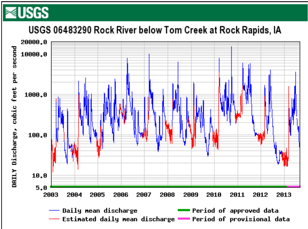
Figure 2. Daily average streamflow at USGS Rock Rapids gage (2003 to 2013).
