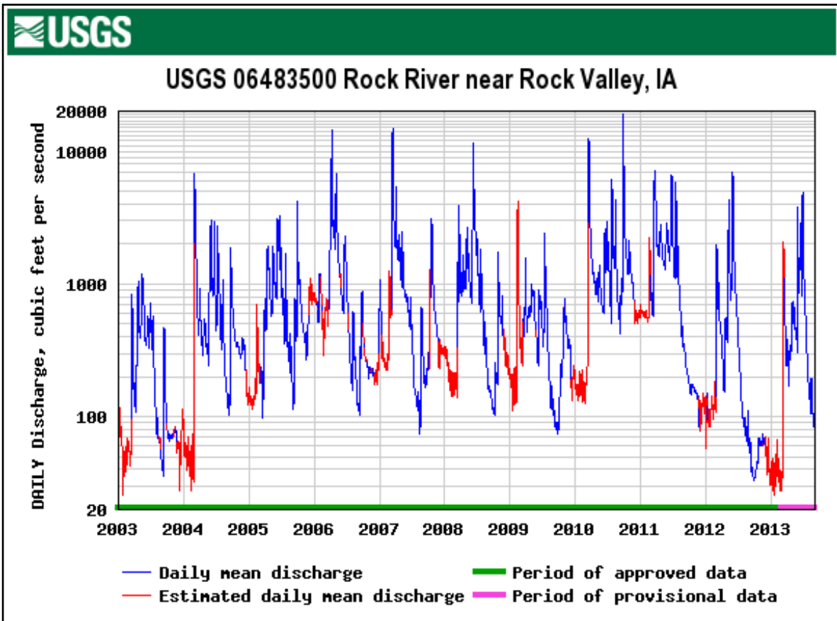
Figure 3. Daily average streamflow at USGS Rock Valley gage (2003 to 2013).
