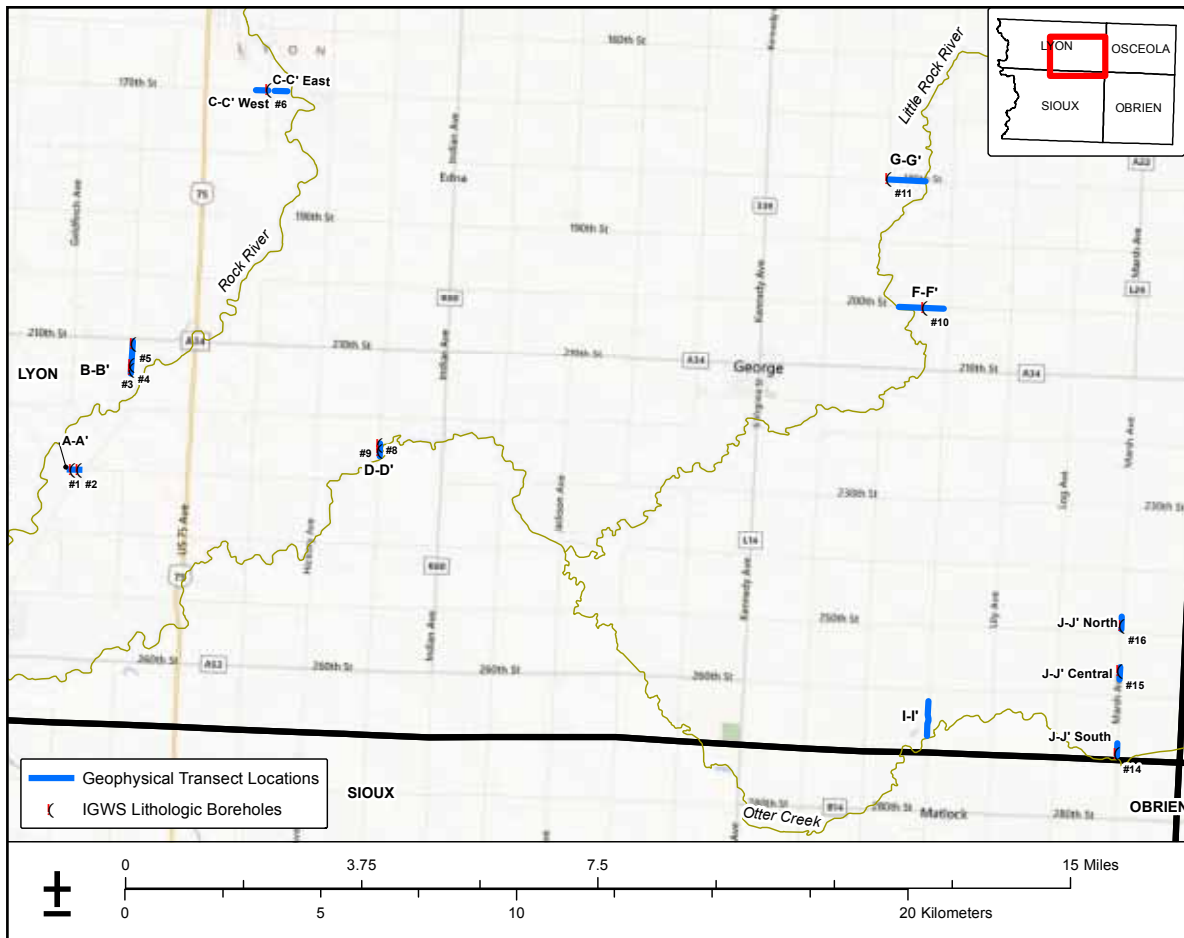
Figure 5. Locations of geophysical surveys and lithologic boreholes.
