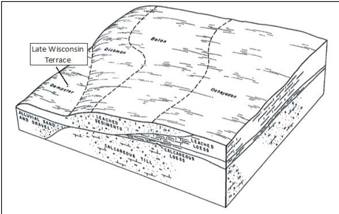
Figure 7. Block diagram representation of soil-geomorphic relationship of Late Wisconsin-age terraces to the adjacent uplands in northwest Iowa (modified from Soil Survey of Lyon County, 1978).
