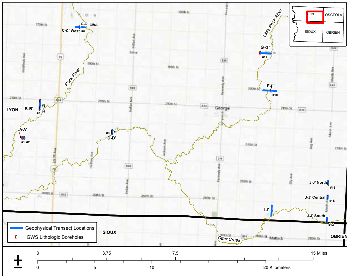
Rock River alluvial aquifer geophysical models
