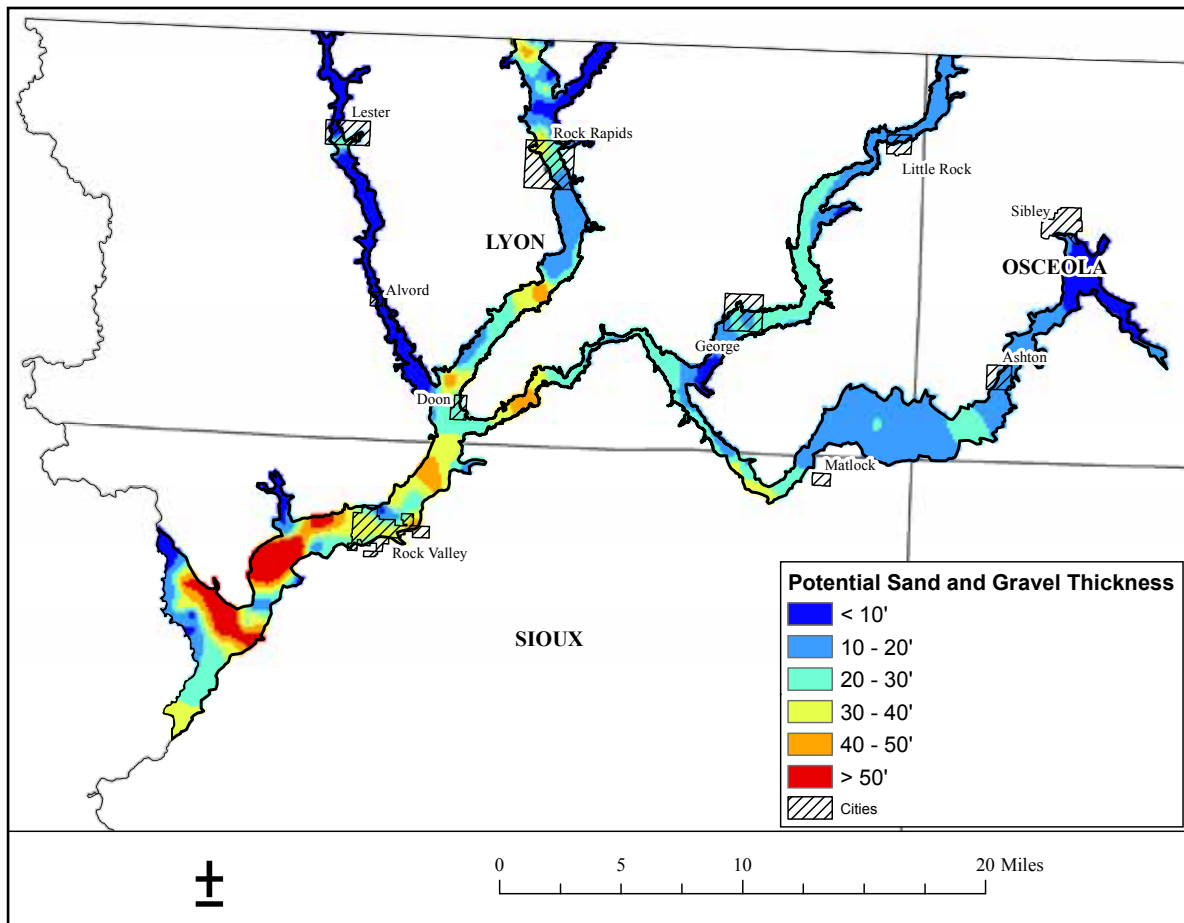
Figure 11. Potential sand and gravel thickness in the Rock River alluvial aquifer.
