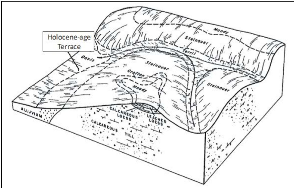
Figure 6. Block diagram representation of soil-geomorphic relationship of Holocene-age terraces to the adjacent uplands in northwest Iowa (modified from Soil Survey of O'Brien County, 1981).
