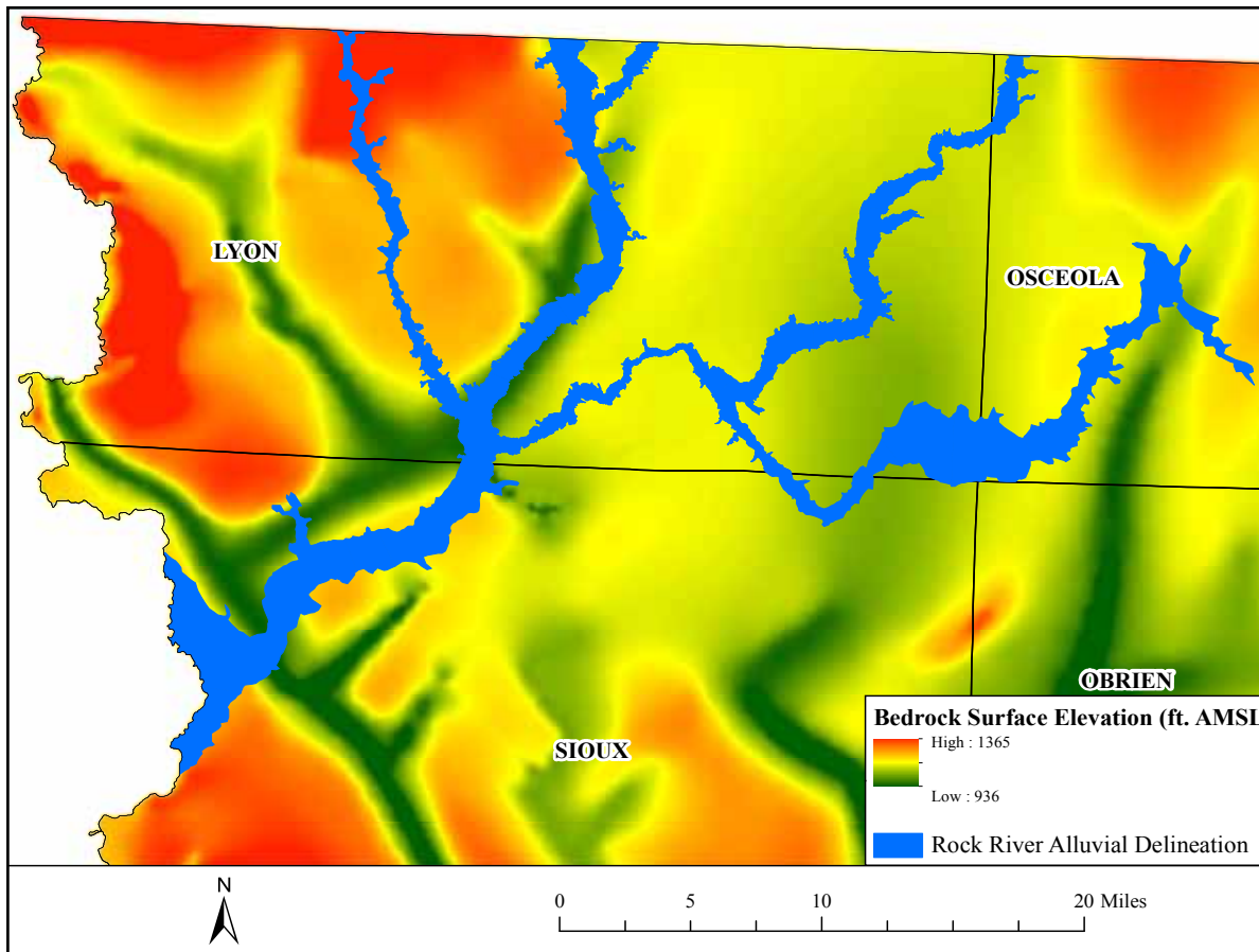
Figure 4. Bedrock surface elevation map showing bedrock highs (reds) and lows (greens).
