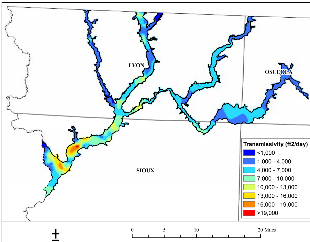
Figure 14. Transmissivity distribution within the Rock River aquifer based on data found in Table 4.
