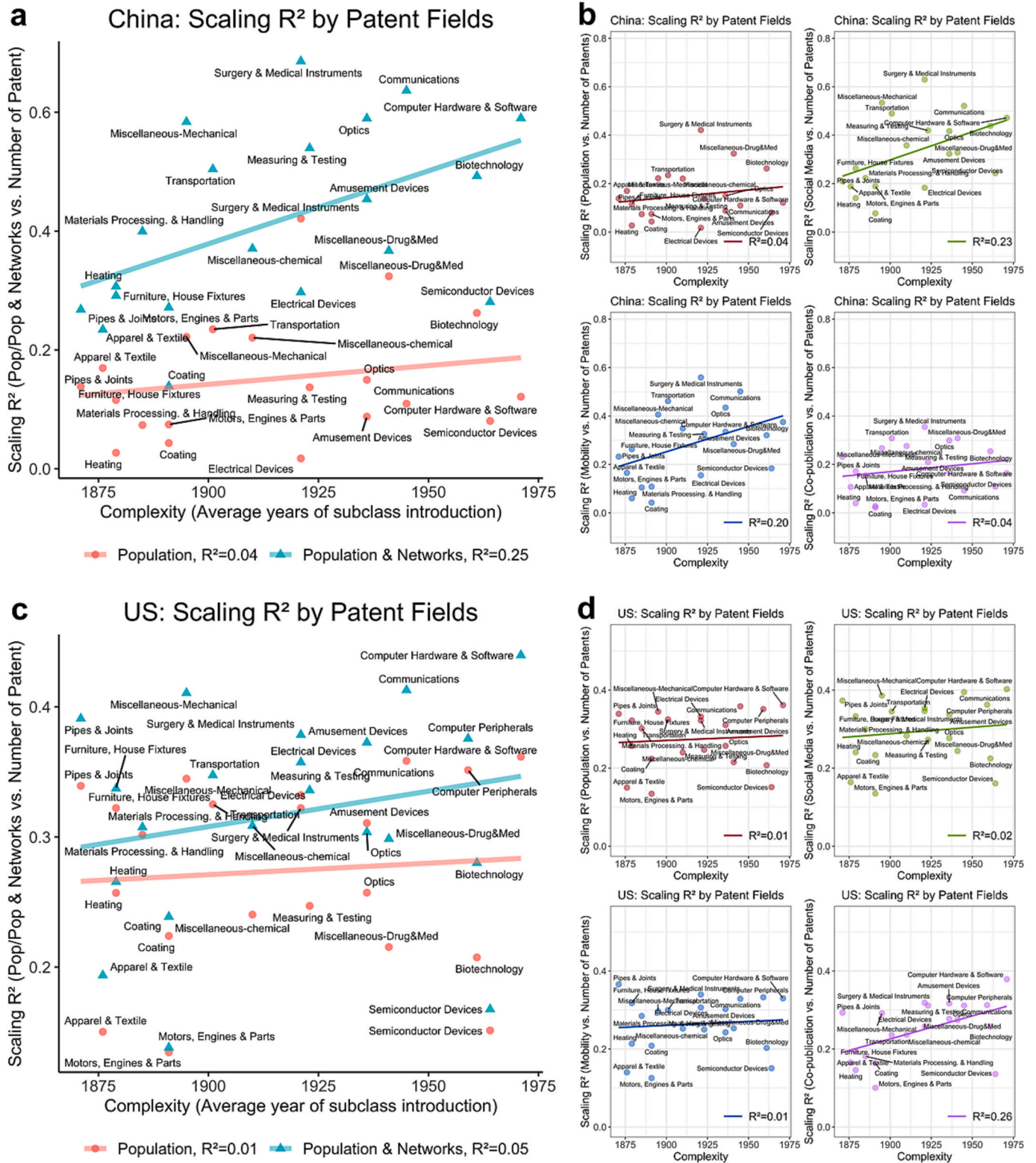
Fig. 4. Comparing Scaling R^2 of model_{pop} and model_{pop+networks} by patent fields. a, China c, U.S. The Scaling R^2 is further broken down using each independent variable in the model to examine each of its contribution in China (b) and U.S. (d). Small-to-medium size cities whose economy depends on tourism are removed.
