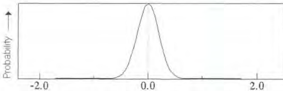
Figure 14 – A Gaussian probability distribution curve with a standard deviation of 0.2 and a mean of 0.0
