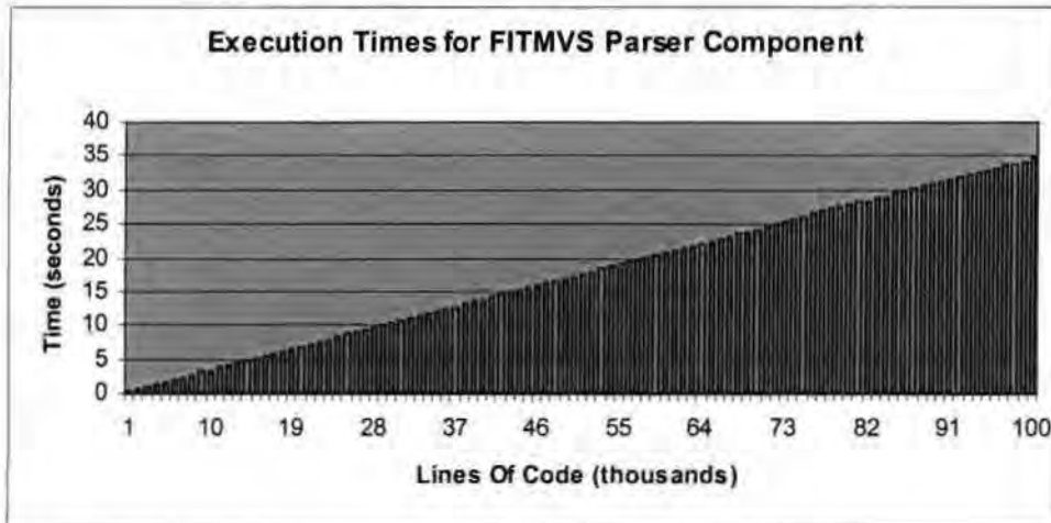
Figure 18 - Parse Times for different sized programs
