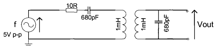
Figure 7-16 Resonant Frequency Test Circuit
