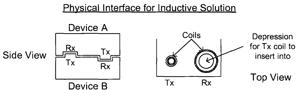
Figure 7-13 Physical Interface For Inductive Solution
