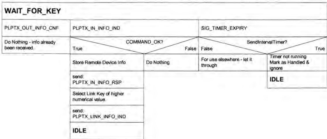
Figure 5-13 Nassi-Schneiderman Diagram of WAIT_FOR_KEY state.
