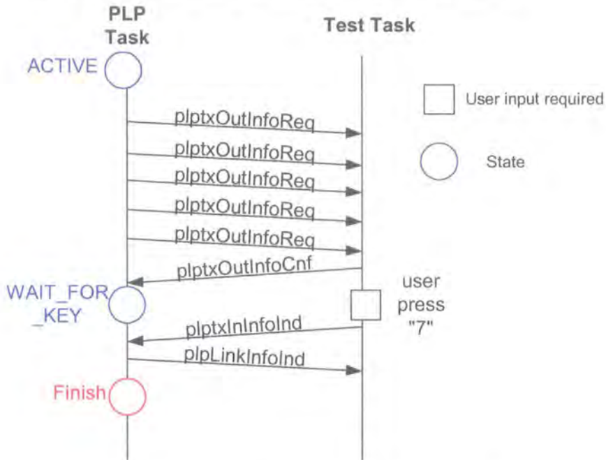
Figure 5-15 Signal Flow between PLP Task and Test Task
