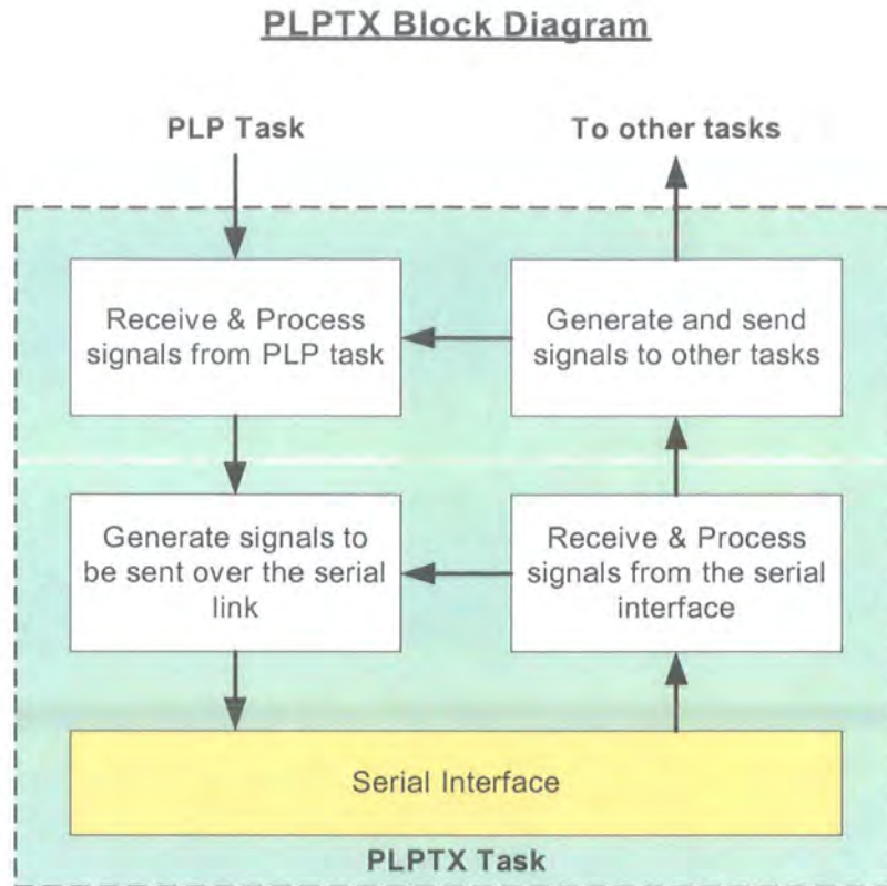
Figure 6-2 PLPTX Block Diagram
