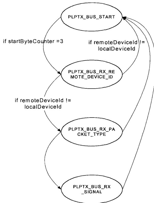
Figure 7-6 RxState Diagram 2
