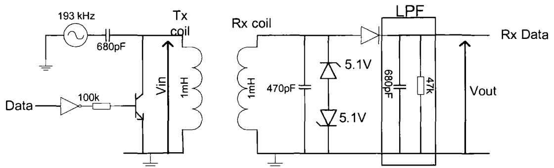
Figure 7-17 Inductive Solution Development Circuit Diagram
