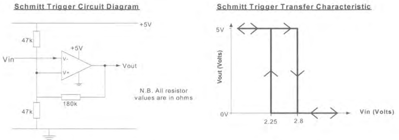
Figure 7-2 Schmitt Circuit Diagram and Transfer Characteristic
