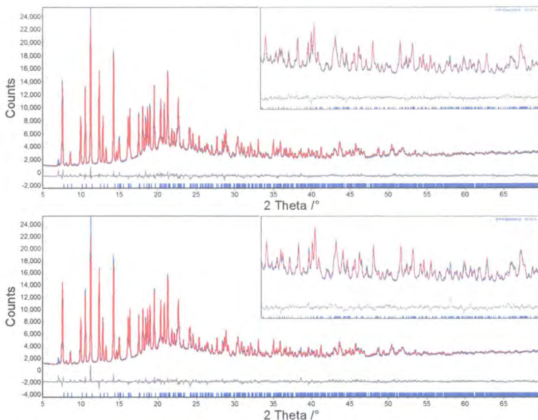
Figure 3.7 Rietveld refinements of (PPh_4)_2Ni(WS_4)_2 with (top) and without (bottom) a preferred orientation correction. The inset shows zooms of the region between 25 and 45 ° 2\theta . Observed data are shown in blue, calculated in red and difference in grey.
