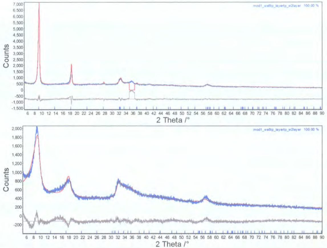
Figure 6.8 Rietveld fits for the iron containing material (top) and for the cobalt containing material (bottom) using structure number 1. Observed data are shown in blue, calculated in red and difference in grey.
