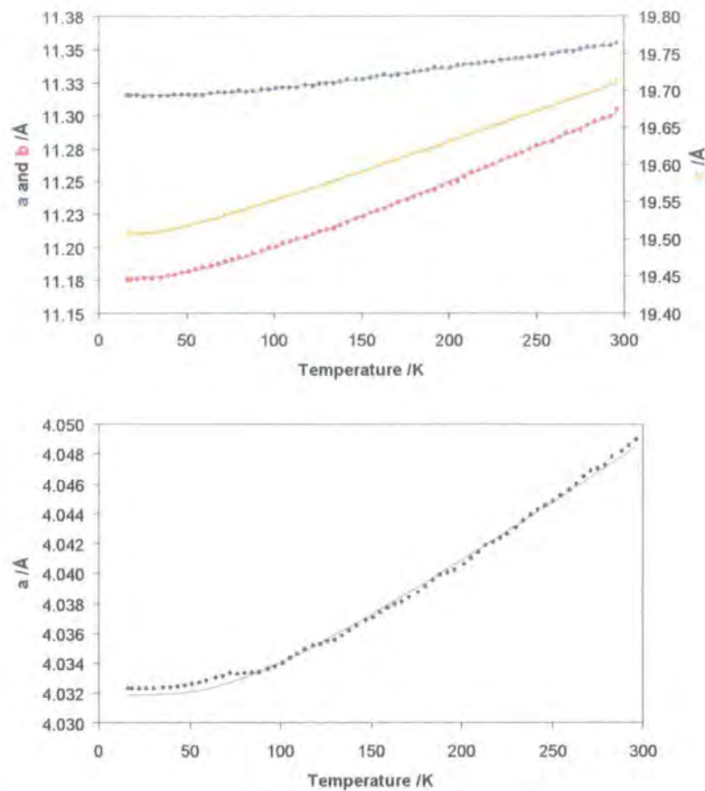
Figure 4.30 The variation of cell parameters for \text{PPh}_4\text{CuWSe}_4 (top) and Al (bottom) with varying temperature. The a cell parameter is shown in blue, b in red and c in yellow, the Al cell parameter is shown in black. Grey lines show values calculated from the Reeber equation.
