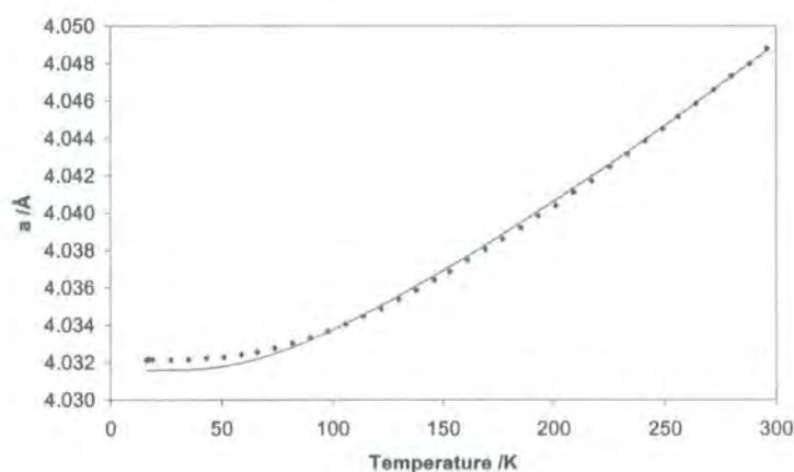
Figure 4.8 The variation in the cell parameter of the aluminium cell parameter during the PheniX experiment. Observed data are shown in black values calculated from the Reeber equation in grey.
