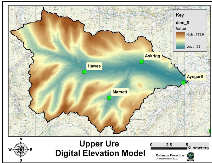
Figure 3.13: An elevation map of the upper Ure catchment.
