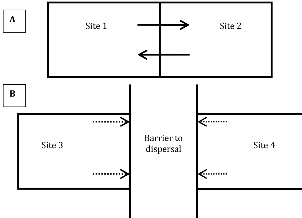
Fig. 2.6: Showing how a fragmented landscape can reduce a population's ability to disperse. With good connections dispersal is a two way process between habitats (A) whereas with fragmented landscapes (B) dispersal is hindered or not possible. In terms of rivers waterfalls, manmade structures including weirs and pollution hotspots can all fragment ecosystems and become barriers to dispersal.
