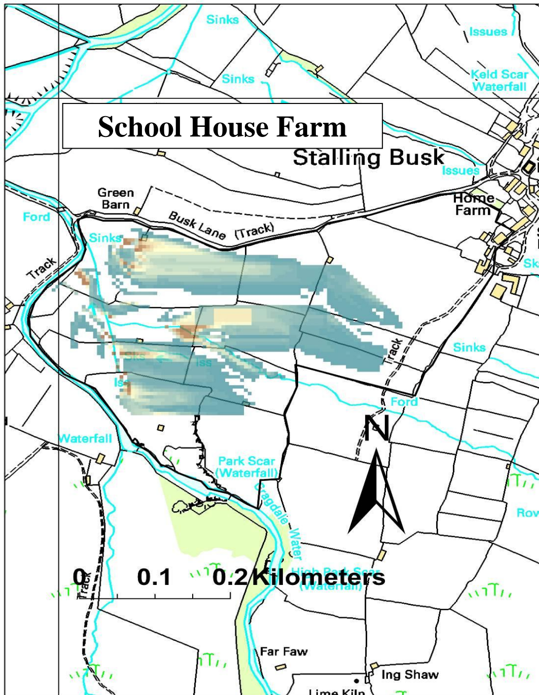
Figure 5.7: SCIMAP results for School House Farm. The outputs are based on the same scale and form as with figure 5.3.
