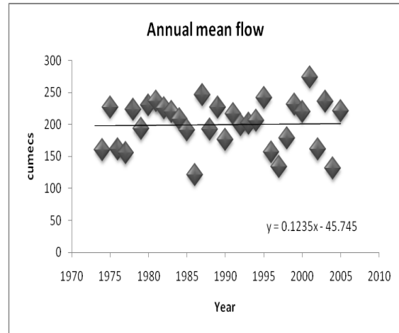
Figure 3.25: The annual mean flow at Snaizeholme displays a static trend. However winter mean flow is increasing in contrast to autumn mean flows which are decreasing slightly.
