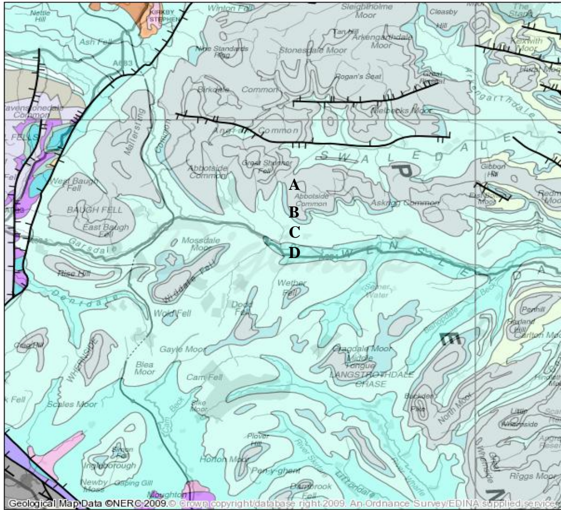
Figure 3.15: The geology of the catchment.
