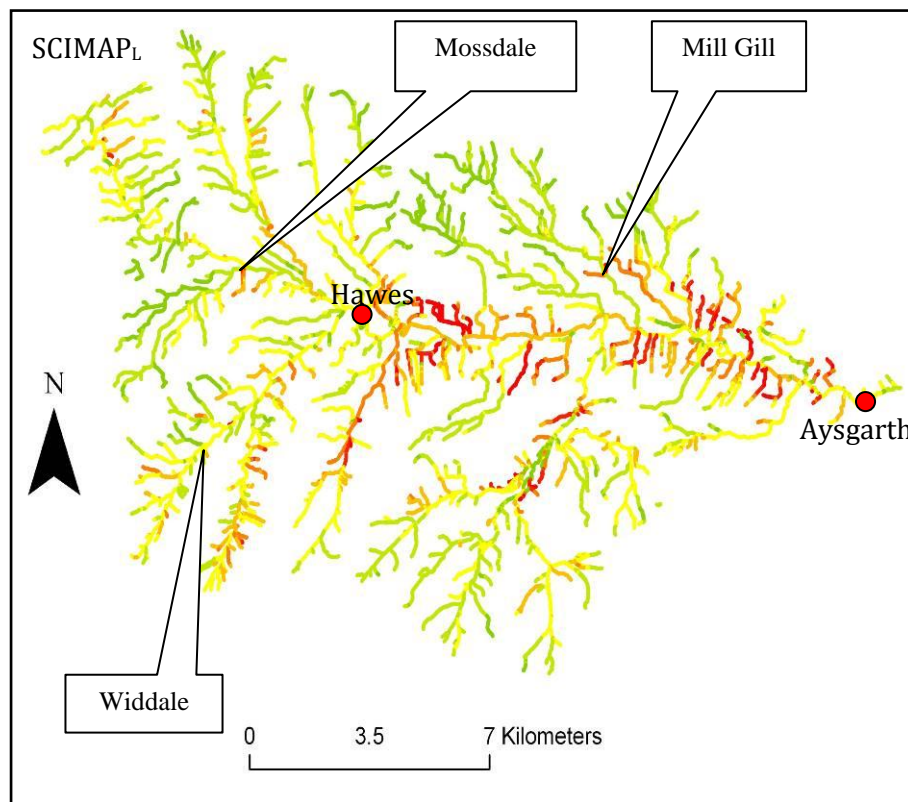
Figure 6.3: Locations where differences in the SCIMAP risk categories between SCIMAP_U , SCIMAP_L and SCIMAP_G are clear.
