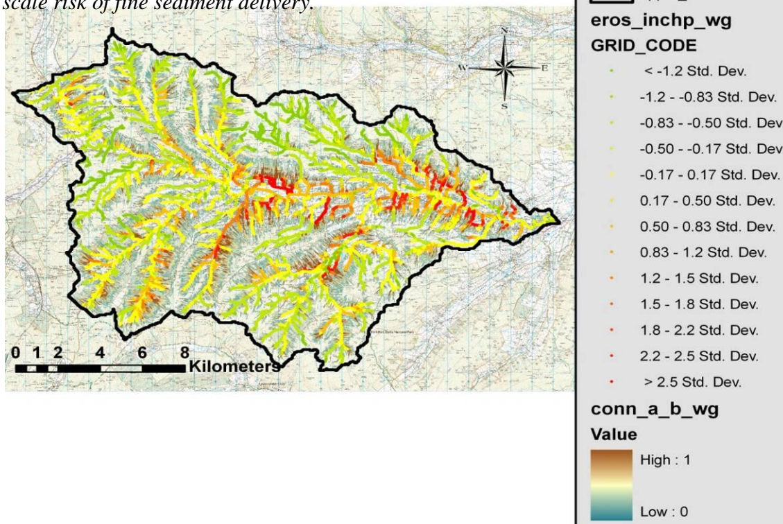
Figure 5.12: catchment-scale SCIMAP results for the upper Ure case study. The outputs show the in-stream risk and field scale risk of fine sediment delivery.
