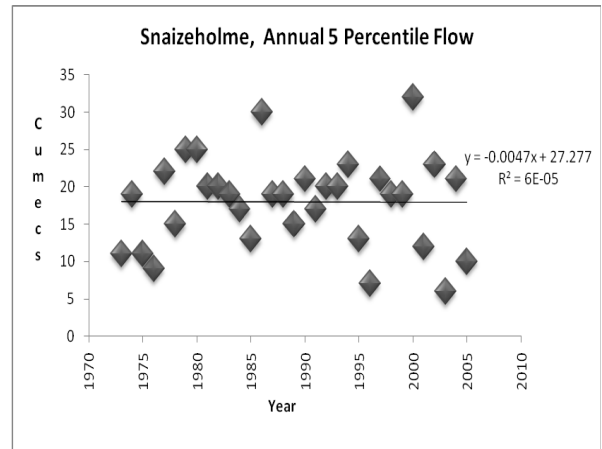
Figure 3.26: Again the annual 5 percentile flow remains static but there are clear trends with the seasonal 5 percentile flows. Summer and autumn show decreasing trend whilst winter 5 percentile flows reveal an upward trend.
