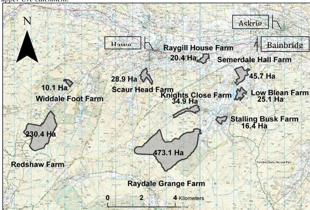
Figure 4.17: The land holdings for running SCIMAP at the farm scale are shown in the map below. They hectarage arnged from 10.1 Ha to 473.1 Ha and covered the typical land cover types of the upper Ure catchment.
