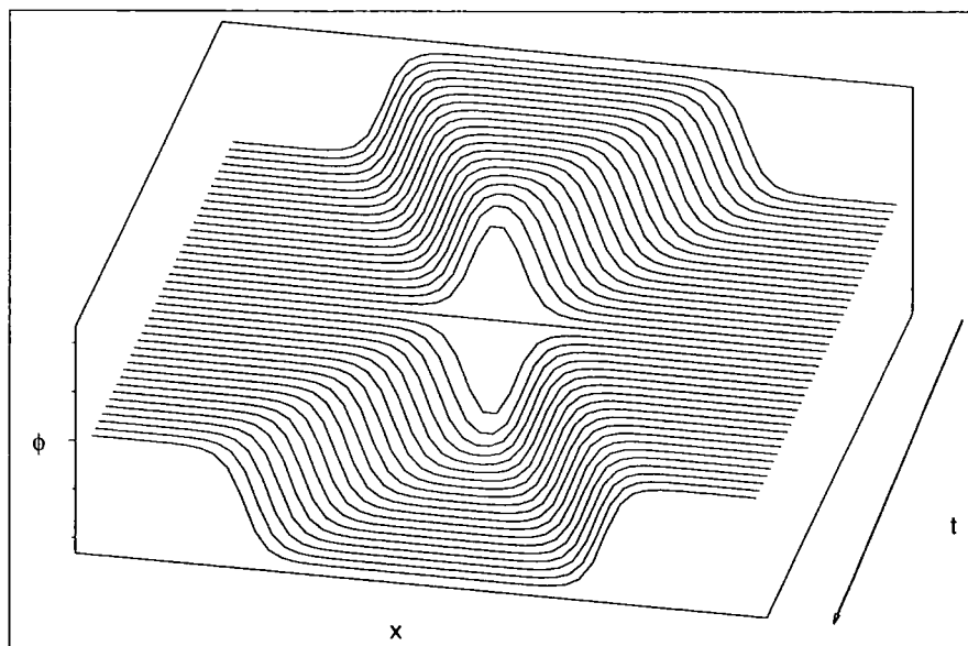
Figure 1.3: Kink-Antikink collision
