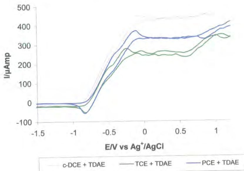
Figure 2.7. Voltammograms showing the catalytic reaction of TDAE with the chlorinated ethenes PCE, TCE, and c-DCE. Scan rate 20\text{mV s}^{-1} .
