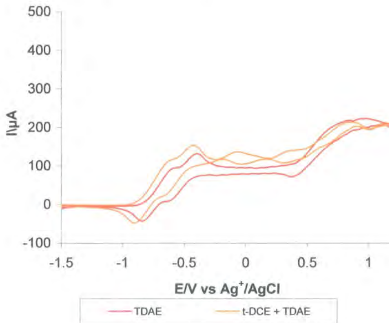
Figure 2.9. trans -Dichloroethene produces virtually no deviance from the voltammogram of TDAE. Scan rate 20mV s -1 .
