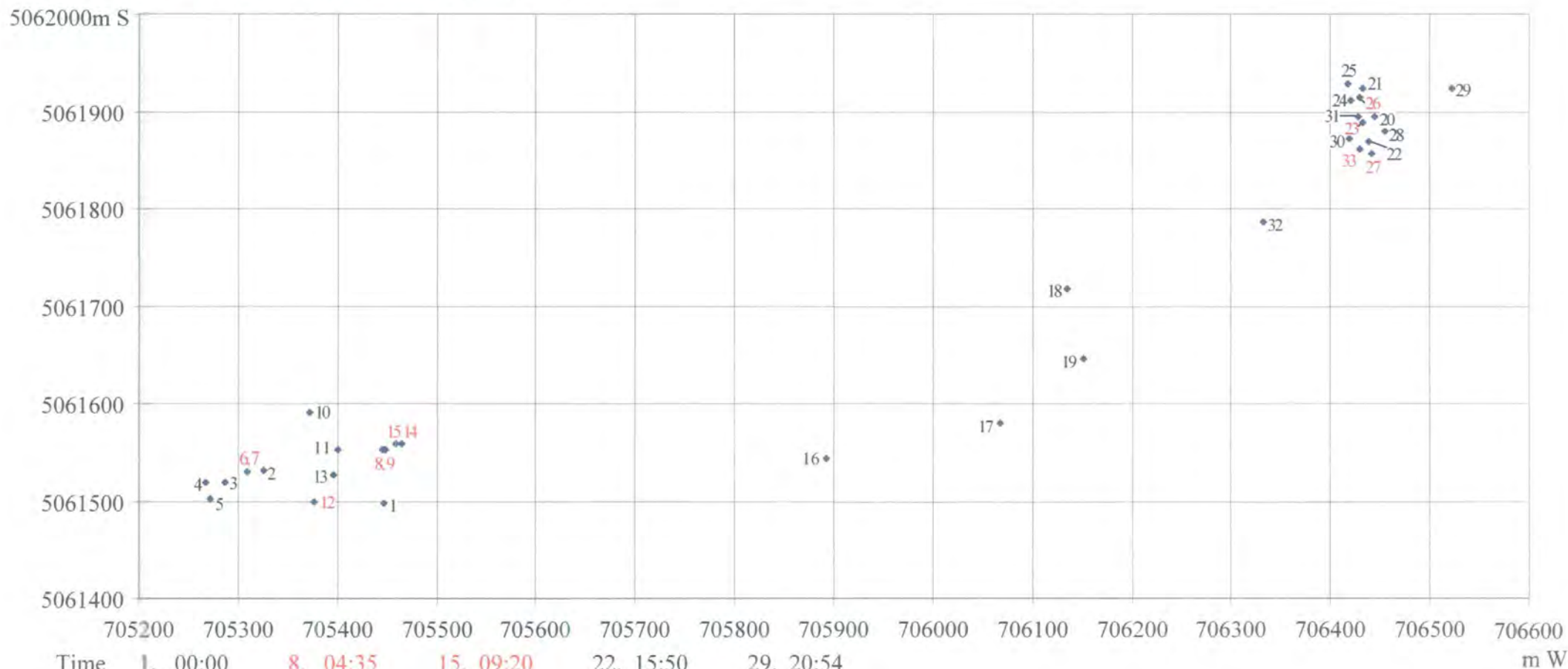
Fig. 5.3.1 Movement distances and times for animal QAM1 as described by continuous radio-telemetry data recorded on 10 th February 2000. Static location fixes are highlighted in red.
