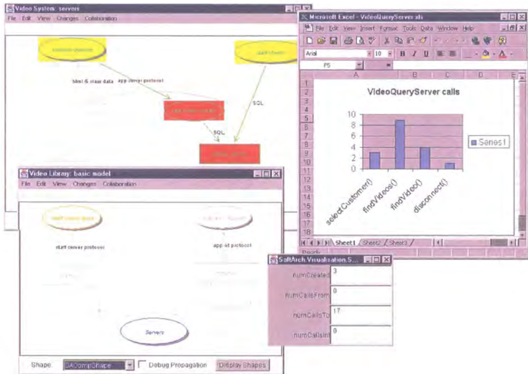
Figure 4-4 SoftArch dynamic view
