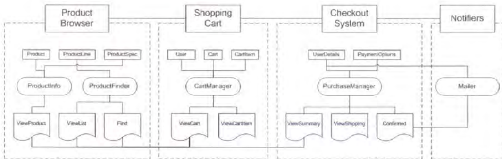
Figure 5-24 Detailed view of shopping cart system
