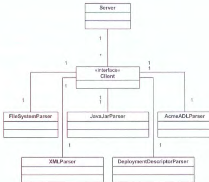
Figure 5-6 Data Extractors in ArchVis
