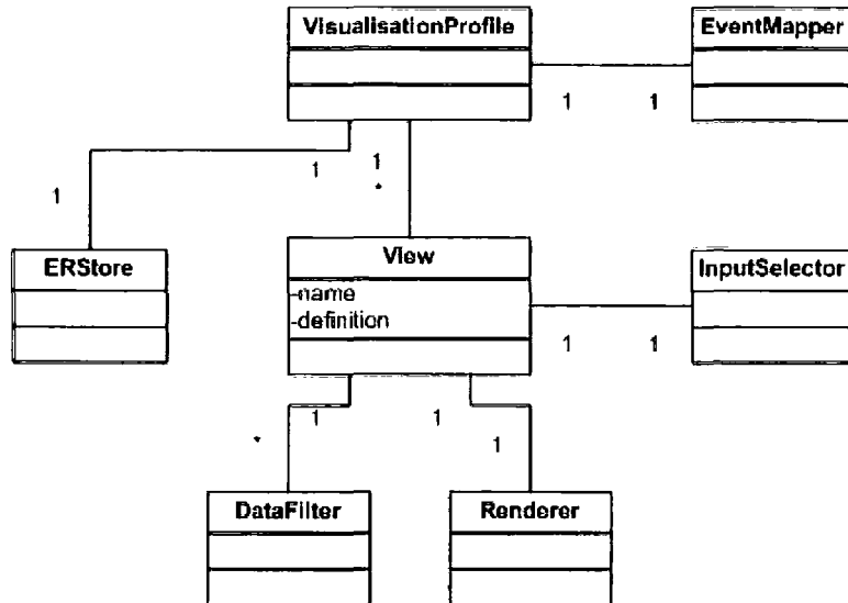
Figure 5-16 ArchVis view model
