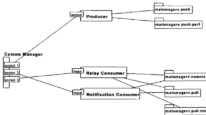
Figure 5-25 Component and connector view with ports, roles and packages
