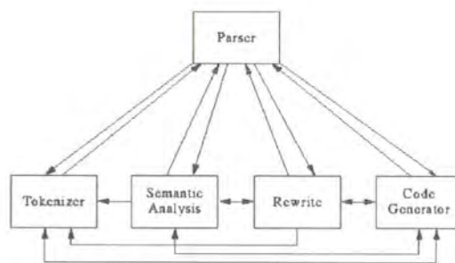
Figure 4-6 System structure redrawn by system designer
