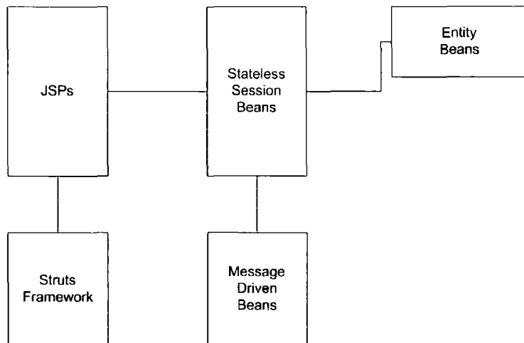
Figure 5-29 Framework and Technology View
