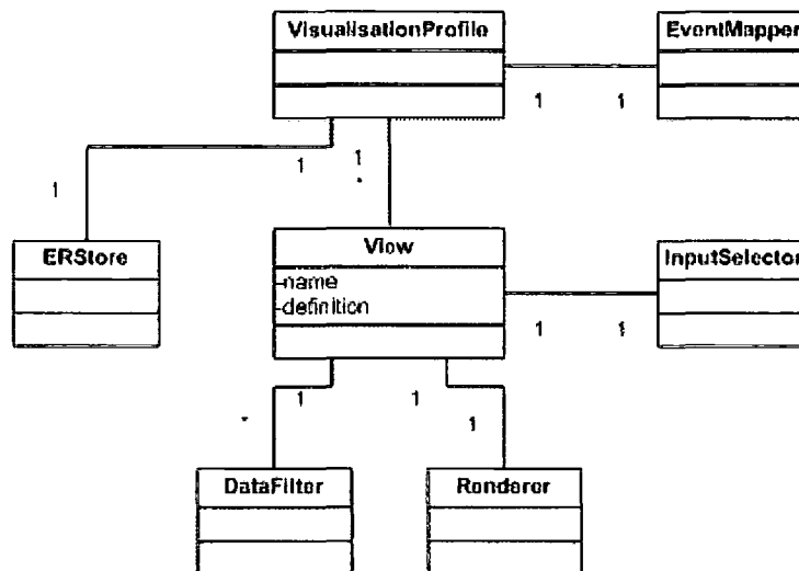
Figure 8-1 ArchVis view model
