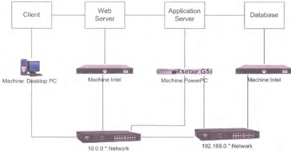
Figure 5-28 A physical deployment view
