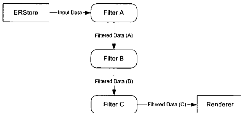
Figure 5-17 ArchVis static data filters
