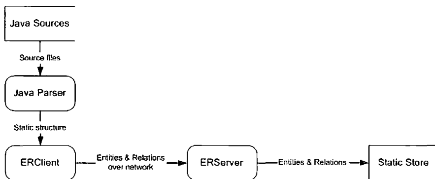
Figure 5-8 Data flow diagram of source code parsing
