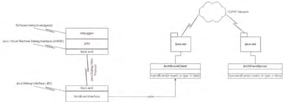
Figure 5-13 ArchVis and the Java debugger interface
