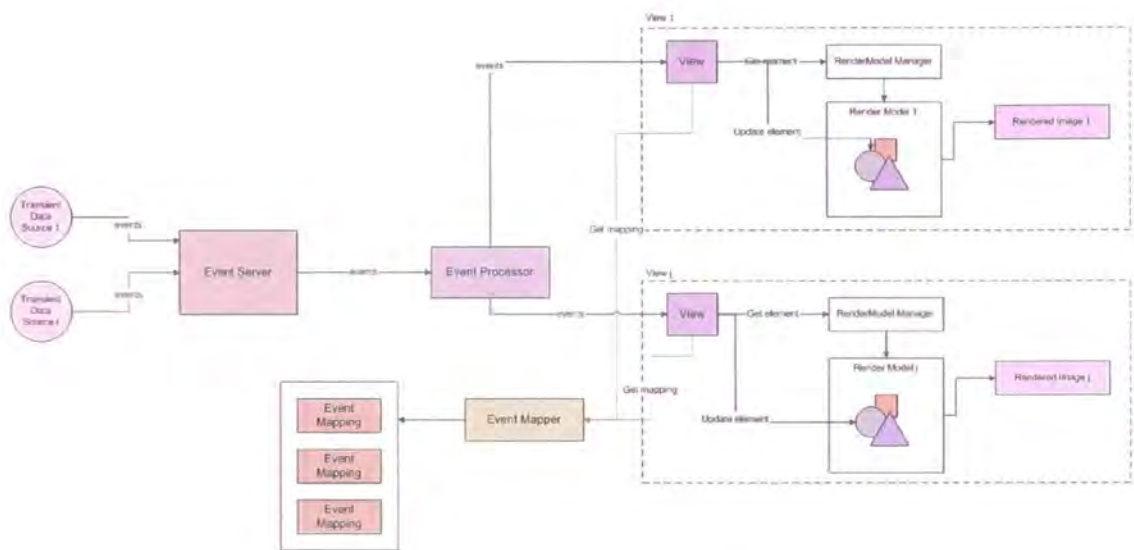
Figure 5-19 Transient data extraction
