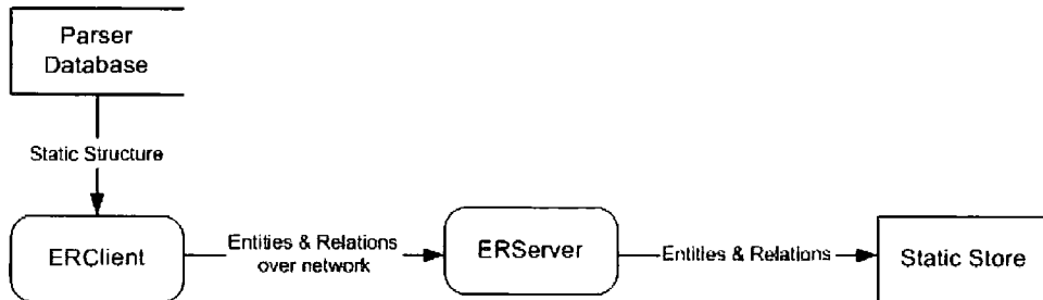
Figure 5-9 Data flow diagram of parser database extraction
