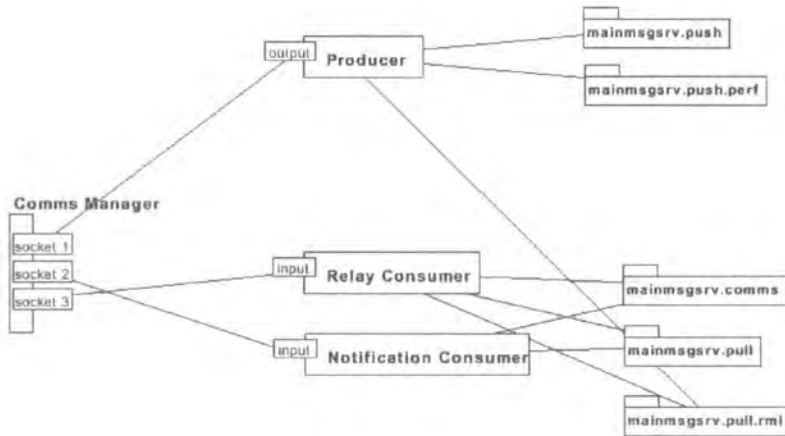
Figure 8-11 As implemented package assignment to architectural components
