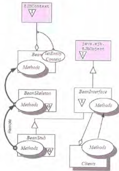
Figure 4-10 LePUS diagram of the Enterprise JavaBeans framework
