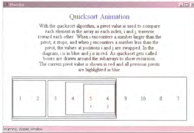
Figure 3-7 Quicksort algorithm animation in SAMBA
