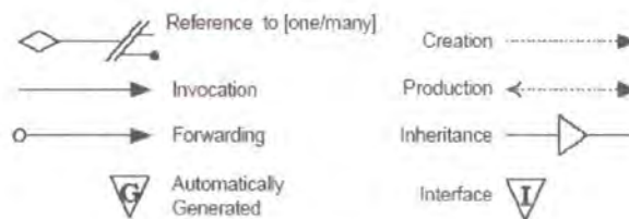
Figure 4-9 Additional LePUS symbols
