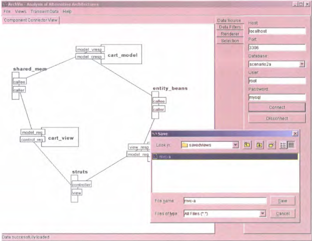
Figure 8-6 Saving a component-connector view
