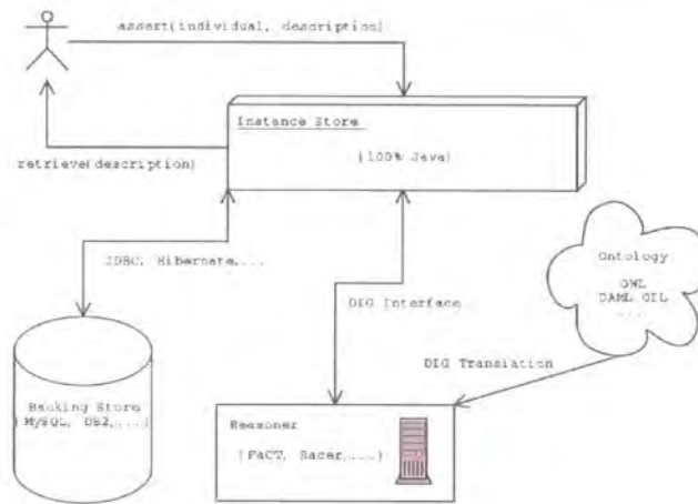
Figure 2-4 Instance Store API Architecture Overview
