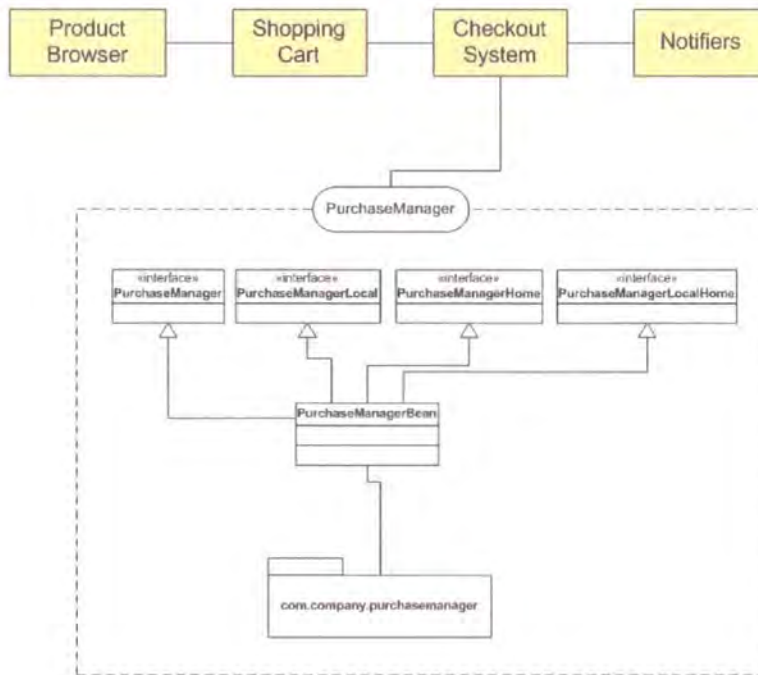
Figure 5-26 UML static model of an architectural component
