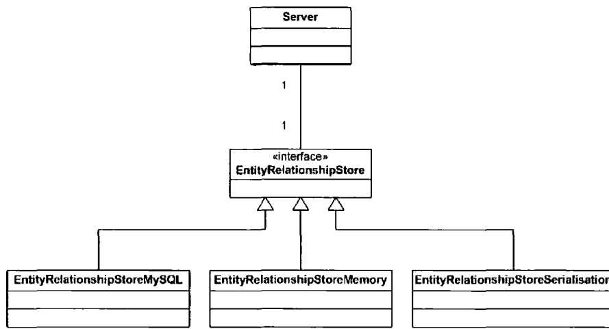
Figure 5-5 EntityRelationshipStore static UML diagram
