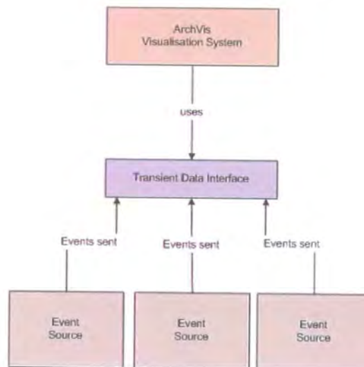
Figure 5-11 ArchVis transient data interface
