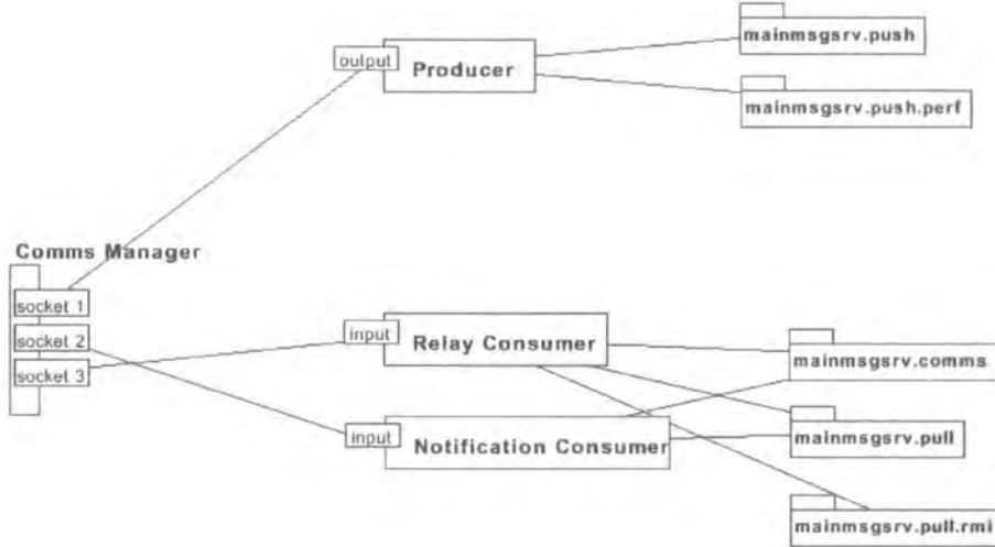
Figure 8-10 As designed package assignment to architectural components
