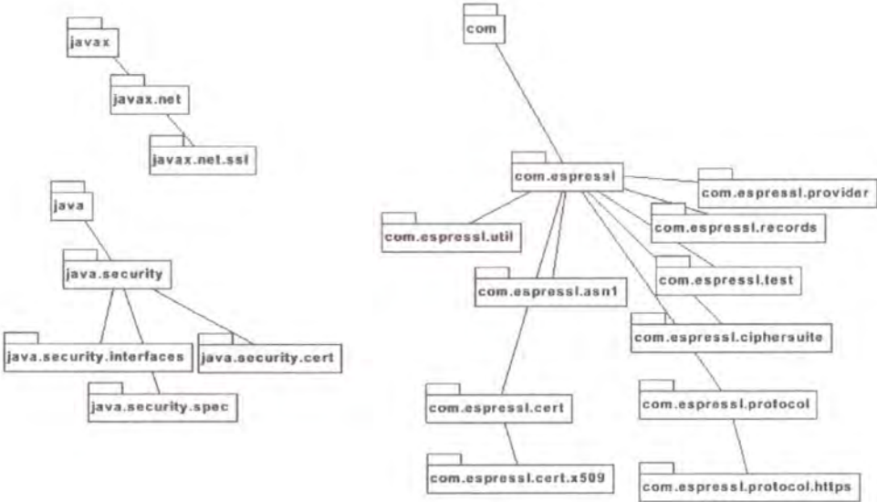
Figure 8-2 Package Structure view
