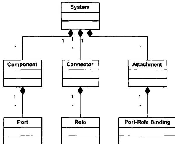
Figure 5-7 Acme ADL language structure
