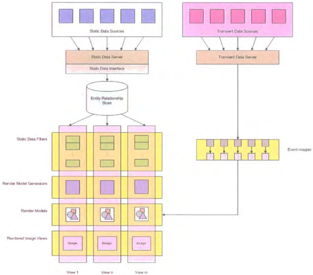
Figure 5-20 ArchVis logical architecture
