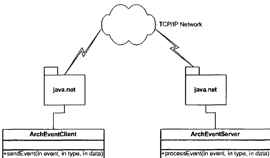
Figure 5-12 ArchVis client-server communication for transient data
