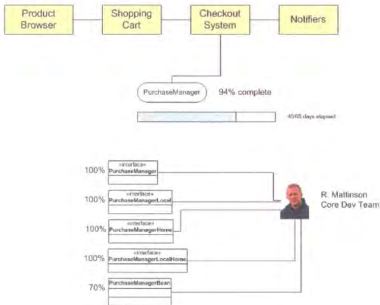
Figure 5-27 Development assignment to classes and interfaces of a component
