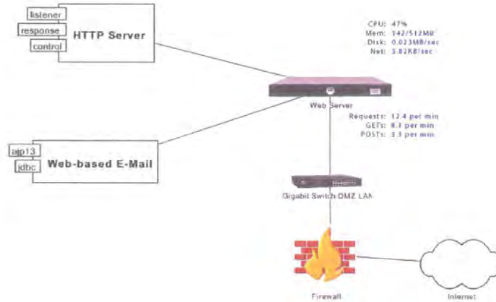
Figure 8-12 Real-time deployment information
