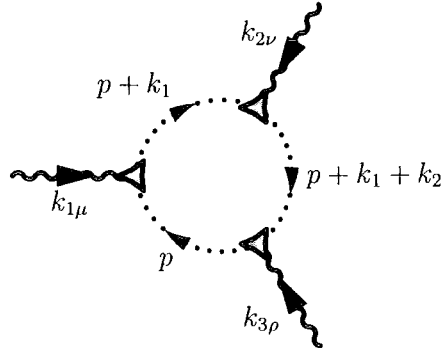
Figure 3.4: This diagram contains three insertions of the triangle J -vertex.
