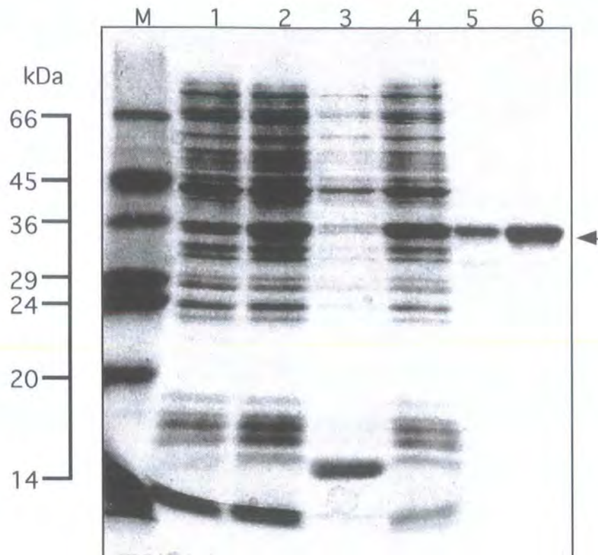
Figure 4.13(a). SDS-PAGE analysis of recombinant DHR protein expressed in BL21 (DE3) STAR (Invitrogen) and purification under denaturing conditions. Protein samples were prepared for SDS-PAGE analysis and resolved on a 12% polyacrylamide gel, proteins were visualised by staining with Coomassie blue. Uninduced cells were grown to an OD \lambda 600 nm (lane 1) and induced with IPTG (0.1 mM). Following induction cells were grown for a further 3 hours (lane 2). A sample of induced cells was split into soluble (lane 3) and insoluble (lane 4) fractions. Recombinant DHR receptor binding domain was purified under denaturing conditions, as described in section 2.8.6 (lane 5) and refolded by dialysis into 10 mM Tris-HCl (pH 7.5) and finally water (lane 6). SDS-7 marker (lane M) was run along with protein samples to estimate protein molecular weight, each band corresponds to approximately 3 \mu g protein. The molecular weight of purified recombinant protein was confirmed by SELDI-TOF mass spectrometry (Fig. 4.13b).
