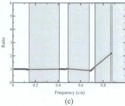
Figure 5.16: TM anisotropy ratios for the rod radii with the highest peak values. The ratios have been plotted as a function of frequency (a, c) and the peak value dispersion surfaces are shown (b, d).
