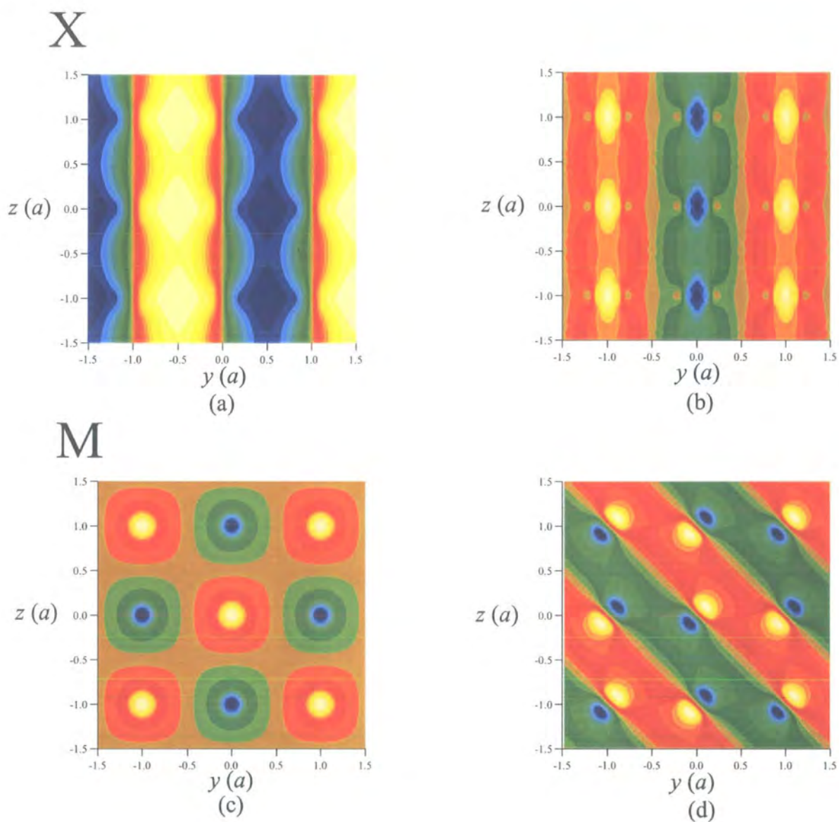
Figure 5.8: Magnetic field profiles for first (left column) and second (right column) bands for the TE modes at the high symmetry points in the Brillouin zone. For key see Fig 5.6.
