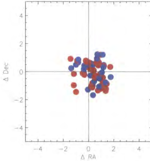
Figure 3.6: Offsets between Chandra and WFI positions for the same sixty-seven objects from table 3.4, in arcsecond units.
