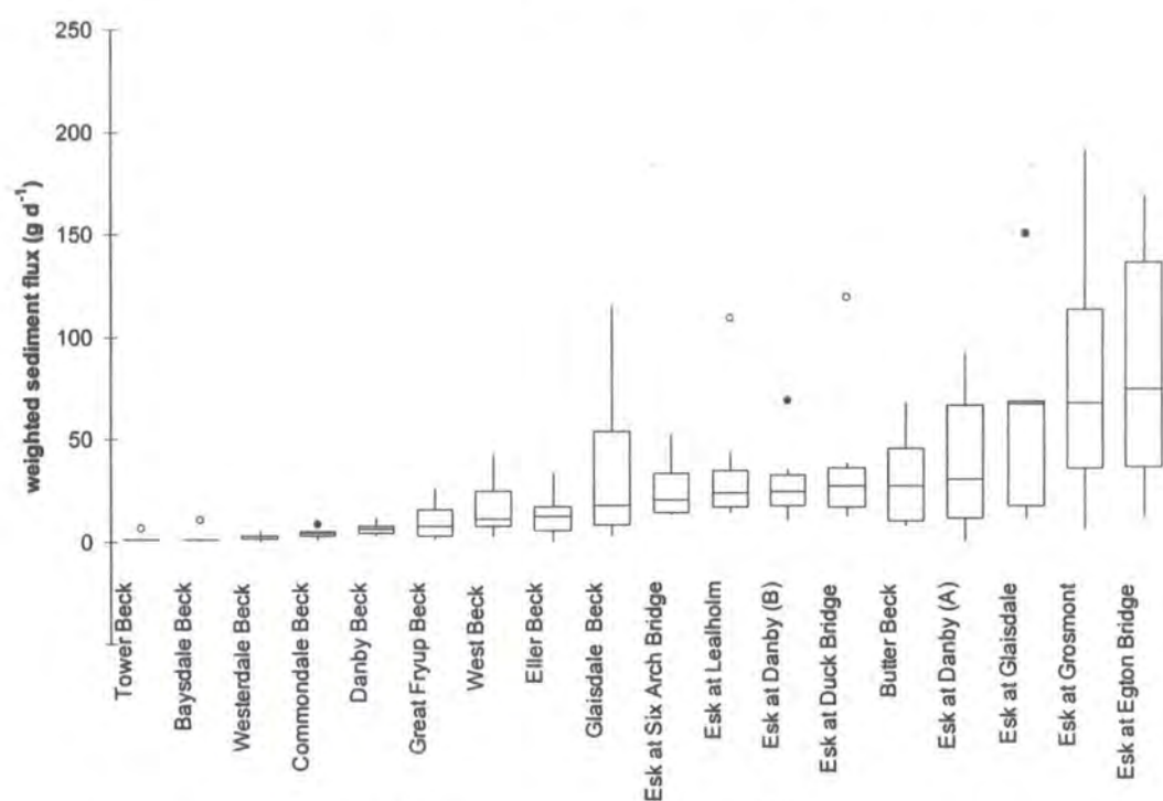
Figure 5.4: Box plots of weighted sediment fluxes ( \text{g d}^{-1} ) from mass flux samplers ordered by median sediment flux
