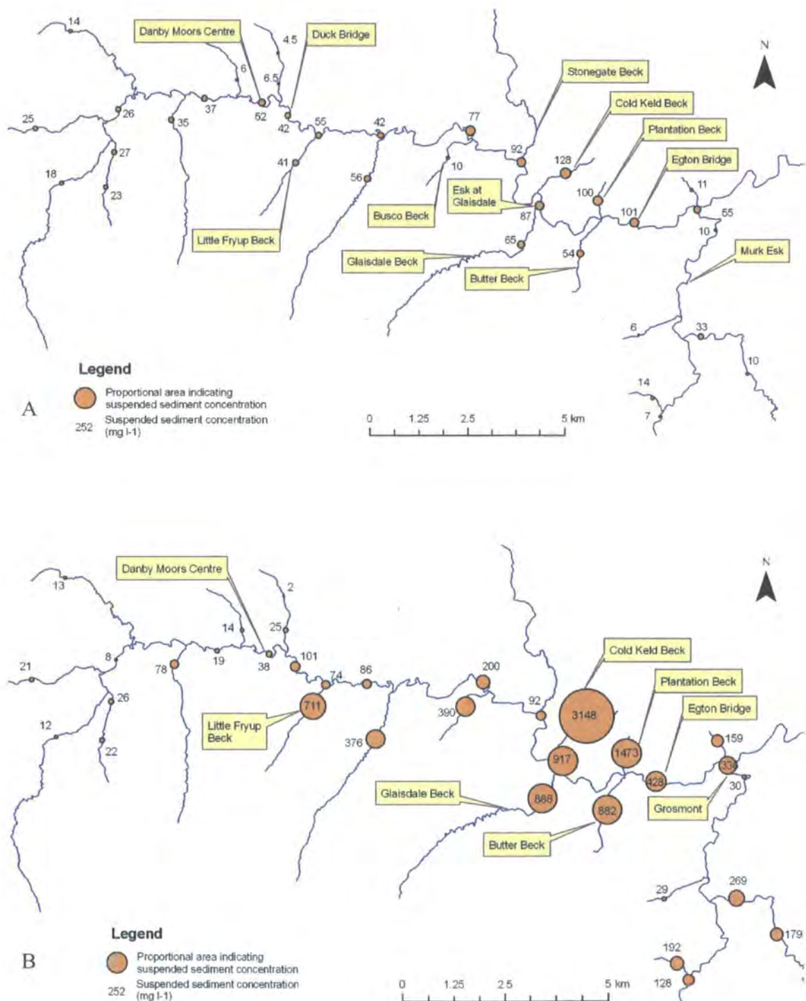
Figure 5.9: Mean suspended sediment concentrations (mg l -1 ) collected from storm ‘gulf’ samples during high flows storm events: (A) 9/11/06; (B) 20/05/06
