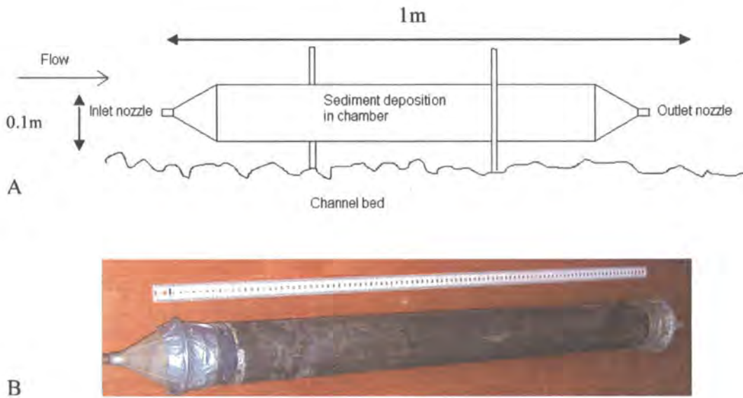
Figure 4.2: A) Diagram and B) Photo of a TIMS (Phillips et al. , 2000)
