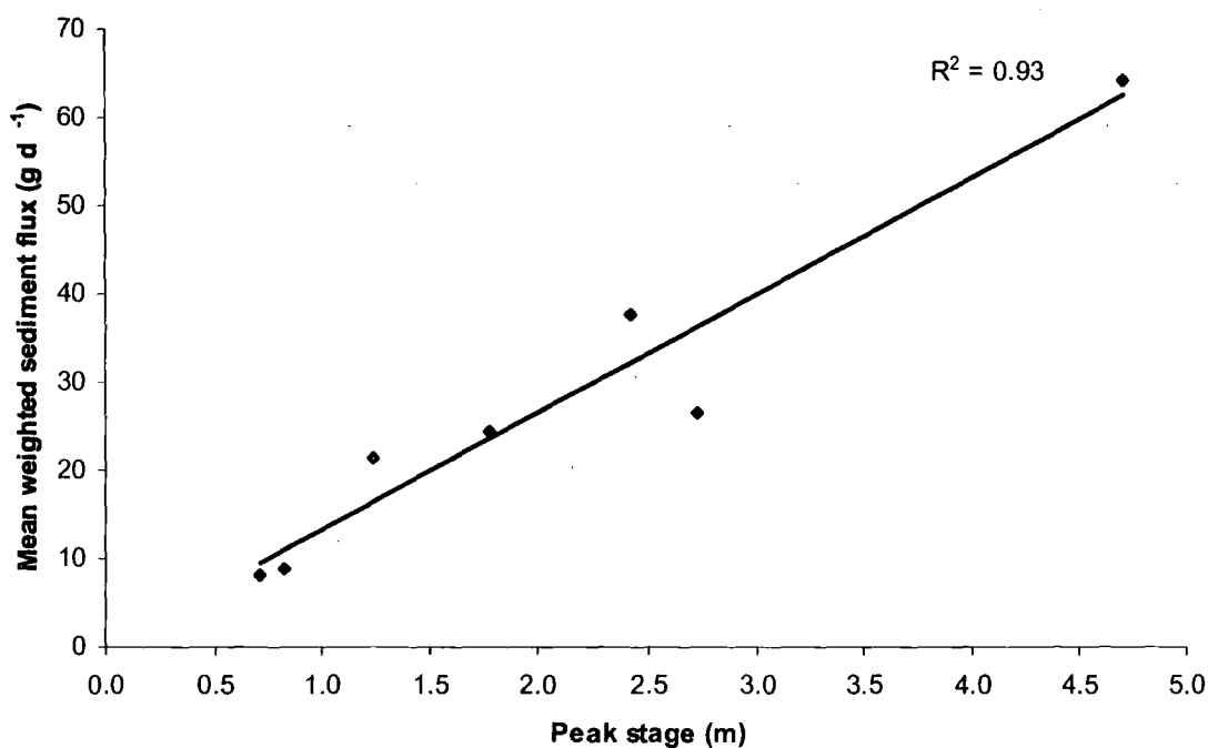
Figure 5.13: Comparison of peak stage records (m) and mean weighted sediment flux ( \text{g d}^{-1} )
