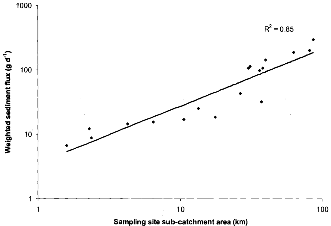
Figure 5.6: Comparison of mean weighted sediment flux ( \text{g d}^{-1} ) and sub-catchment areas of each TIMS sampling site ( R^2 = 0.85 )
