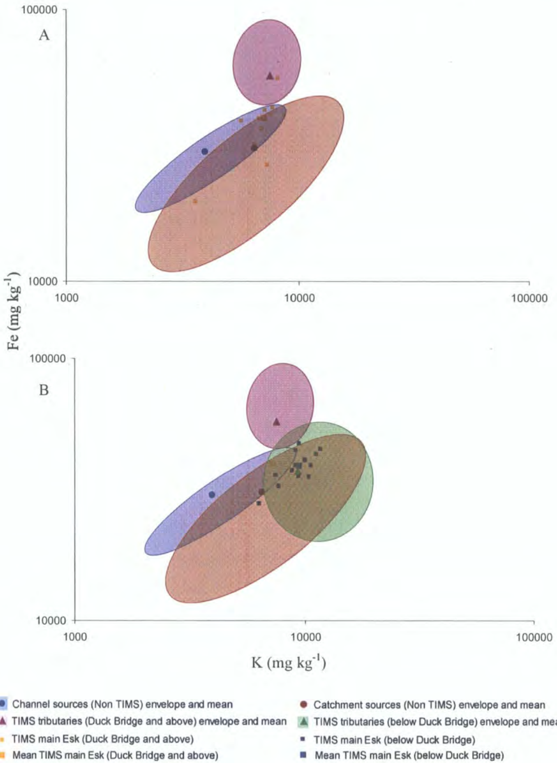
Figure 7.10: Comparison of K and Fe concentrations for: A) TMS main Esk samples above Duck Bridge; and B) TMS below Duck Bridge, with mean K and Fe concentrations for TMS tributaries (above and below Duck Bridge) and channel and catchment (Non-TMS) samples
