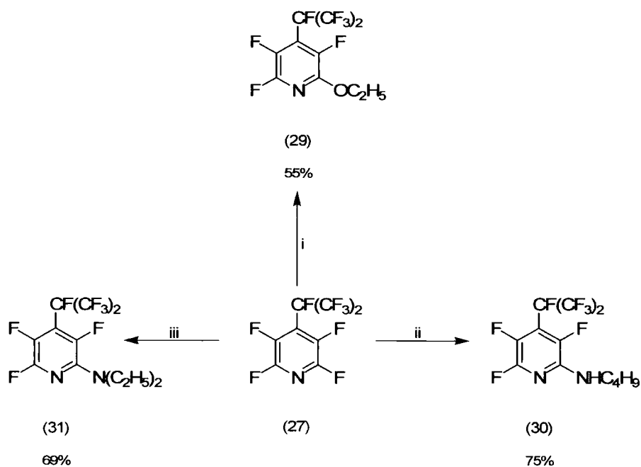
Figure 4.14. Reagents and Conditions: i, NaOC 2 H 5 (1.2 equiv), C 2 H 5 OH, reflux; ii, H 2 NC 4 H 9 (2.2 equiv), THF, reflux; iii, HN(C 2 H 5 ) 2 (2.2 equiv.), THF, reflux.
