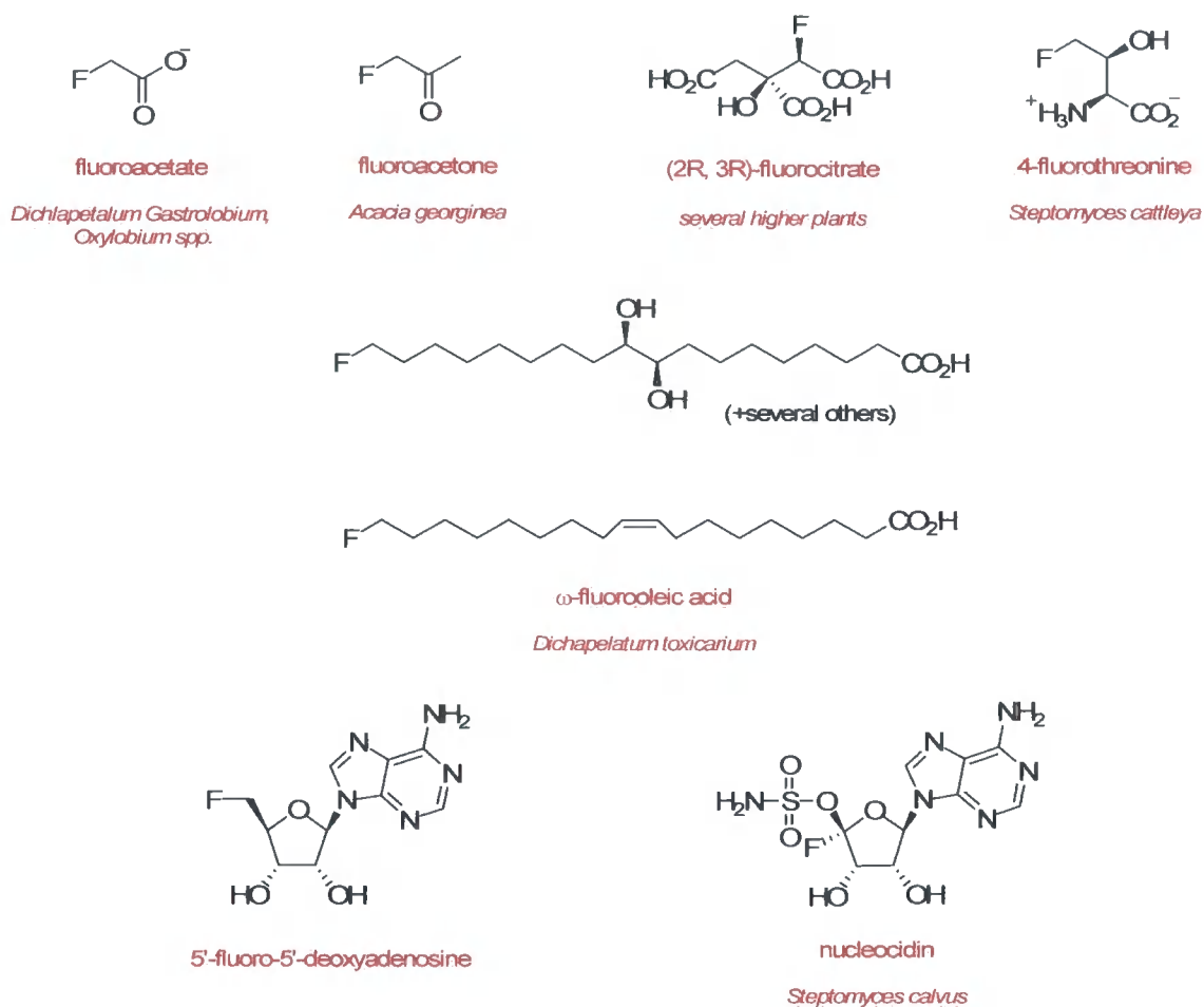
Figure 1.2. Naturally occurring fluorinated compounds.
