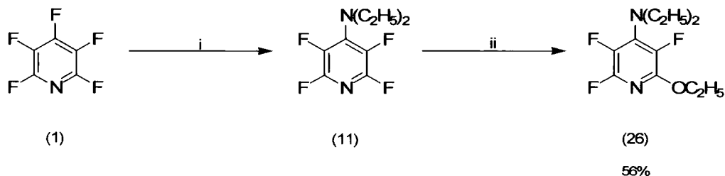
Figure 4.15. Reagents and Conditions: i, HN(C 2 H 5 ) 2 (1 equiv.), NaHCO 3 (2 equiv.), THF, reflux; ii, C 2 H 5 ONa (1 equiv.), THF, reflux.
