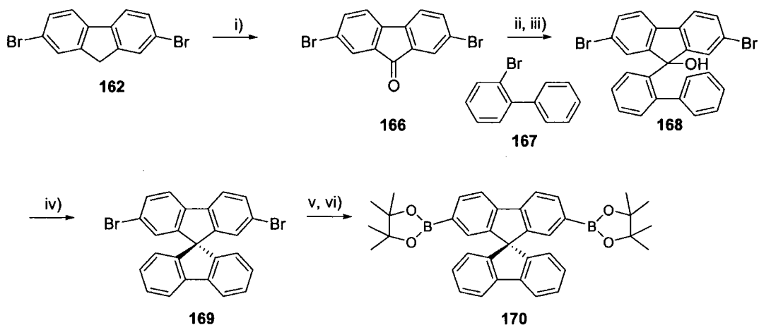
Scheme 72: Synthetic route to 2,7-di(4,4,5,5-tetramethyl-1,3,2-dioxaborolan-2-yl)spirobifluorene 170 : (i) \text{CrO}_3 , AcOH, \Delta ; (ii) 2-bromobiphenyl 167 , t -BuLi, THF, -78^\circ\text{C} ; (iii) 166 , -78^\circ\text{C} \rightarrow 20^\circ\text{C} ; (iv) HCl, AcOH, \Delta ; (v) n -BuLi, THF, -78^\circ\text{C} ; (vi) 2-isopropoxy-4,4,5,5-tetramethyl-[1,3,2]-dioxaborolane -78^\circ\text{C} \rightarrow 20^\circ\text{C} .
