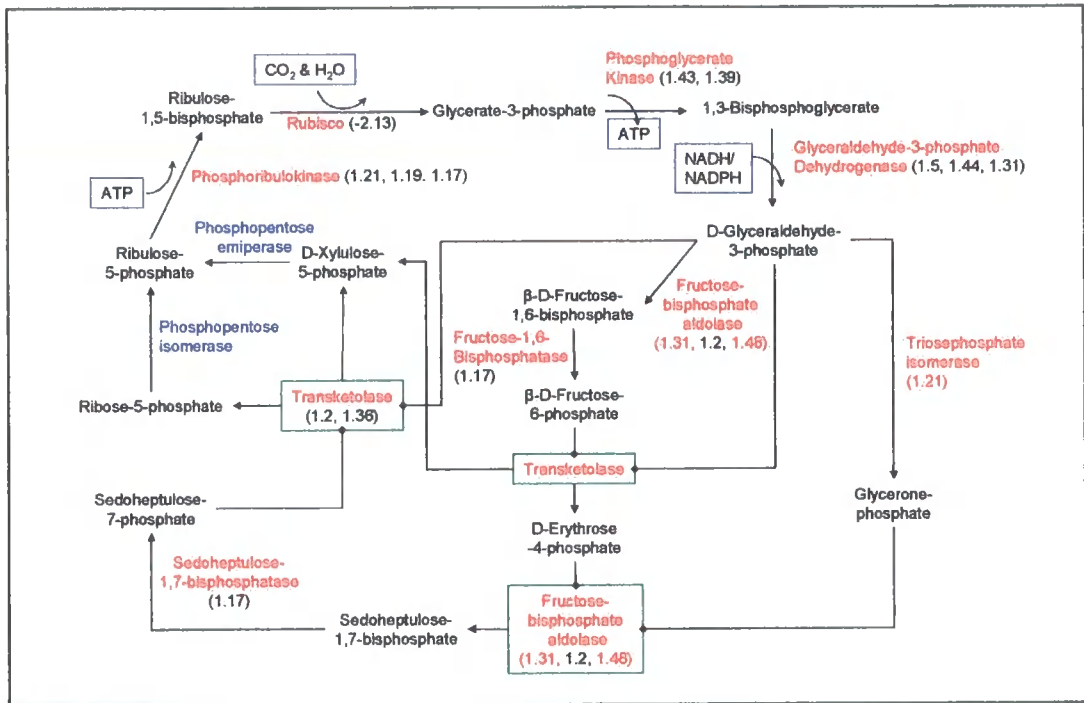
Figure 4.24. Proteins involved in the Calvin cycle which display a heat shock induced change in abundance.
