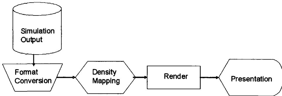
Figure 7.3: Dark Matter Simulation Pipeline
