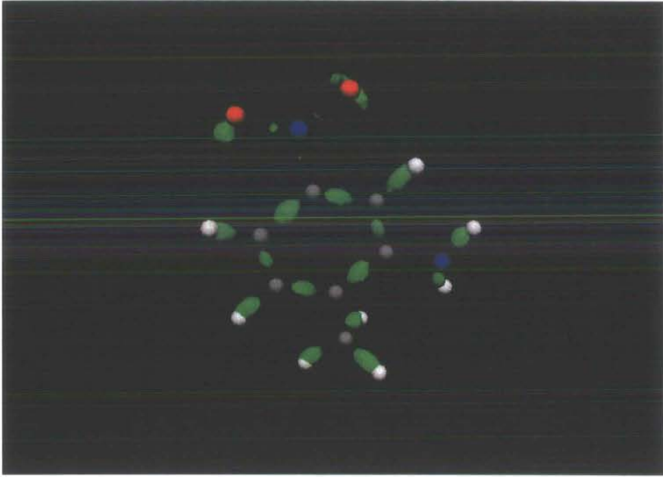
Figure 9.2: X-Ray Crystallography Scenario Result
