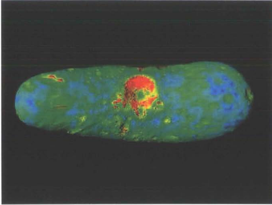
Figure 2.4: Gravity Slope on the asteroid Eros [NASA Goddard Space Flight Center]
