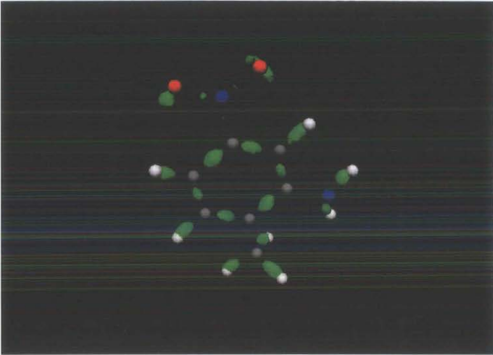
Figure 7.2: X-Ray Crystallography Results
