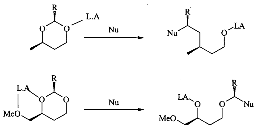
Scheme 4.13
