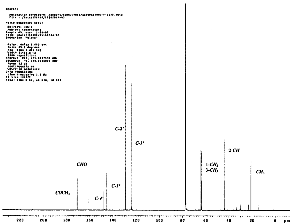
13 C NMR spectrum of 3-formyl-2-(4'-nitro)-propyl acetate (62)
