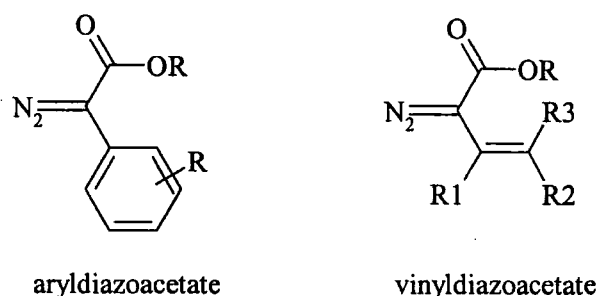
Scheme 1.19
