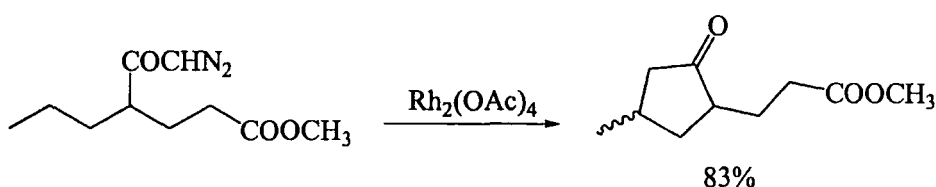
Scheme 1.69
