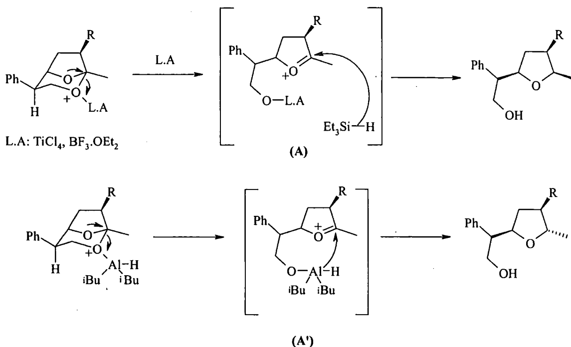
Scheme 4.22
