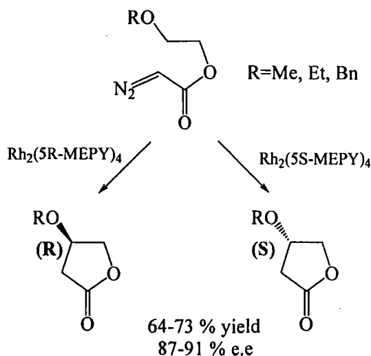
Scheme 1.92
