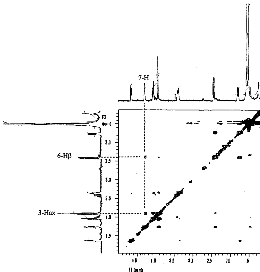
Scheme 4.38
