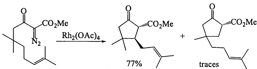
Scheme 1.66
