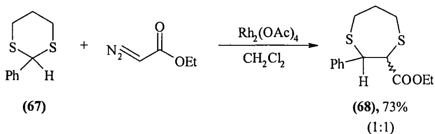
Scheme 1.40
