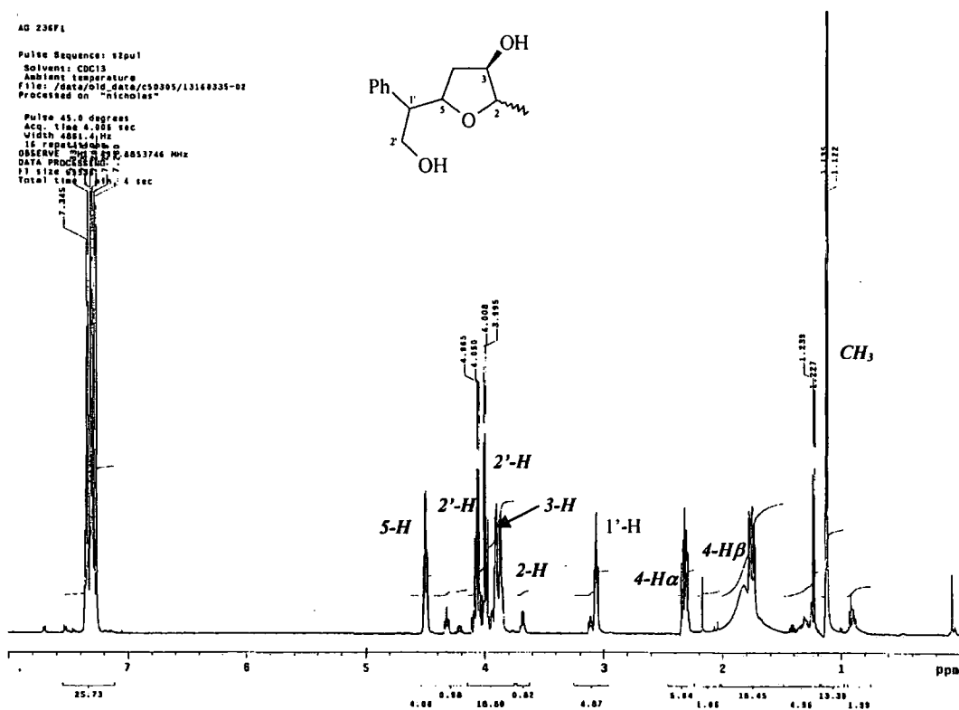
^1\text{H} NMR spectrum of 5-(2'-hydroxy-1'-phenyl-ethyl)-2-methyl-tetrahydrofuran-3-ol (68,69). (for comparison with the oxepane spectrum)
