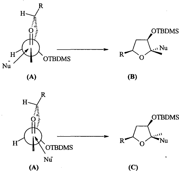
Scheme 4.44
