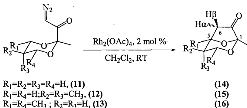
Scheme 2.18
