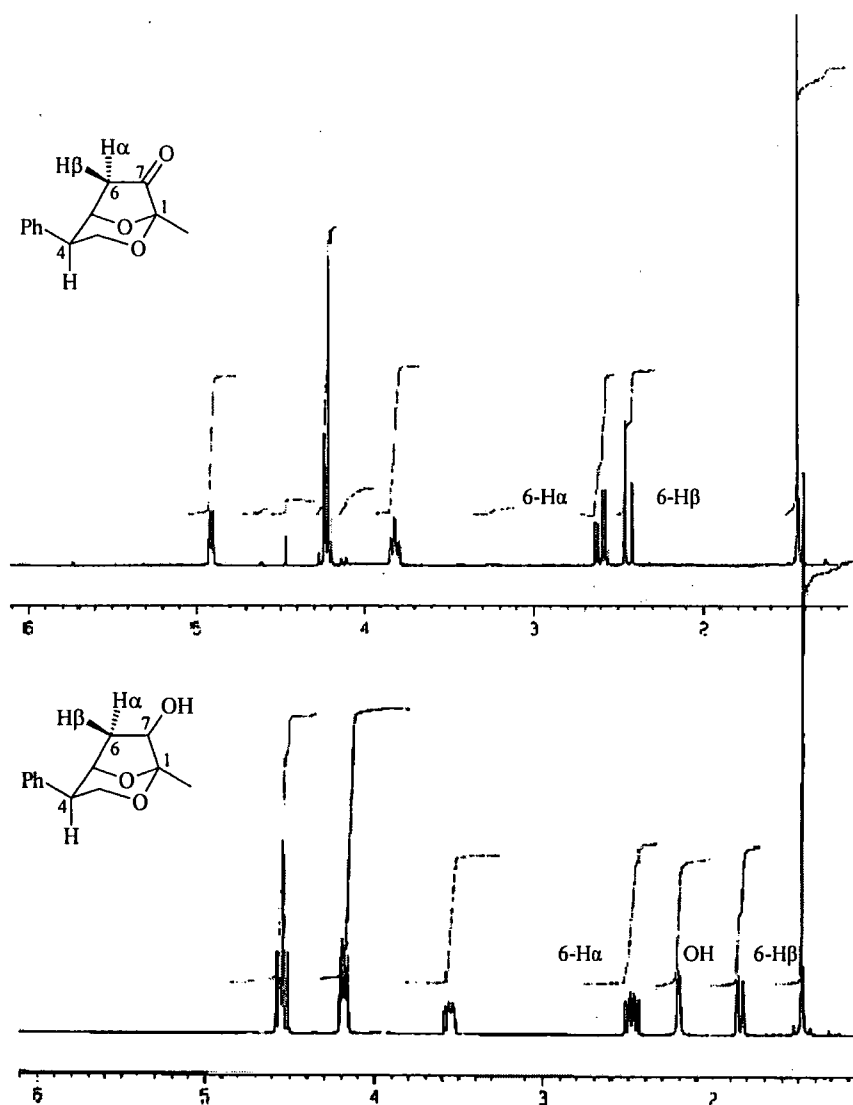
Scheme 4.25
