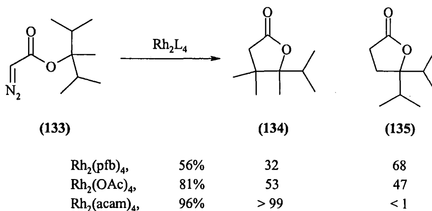
Scheme 1.73
