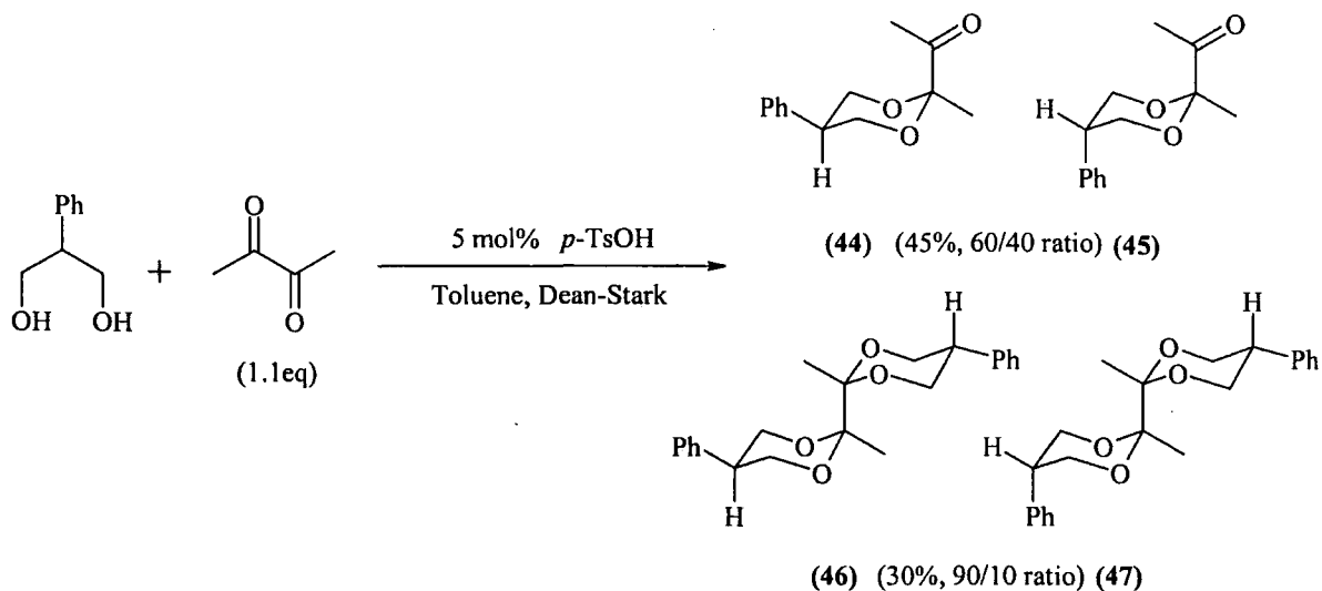
Scheme 3.28
