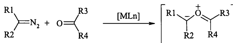
Scheme 1.31
