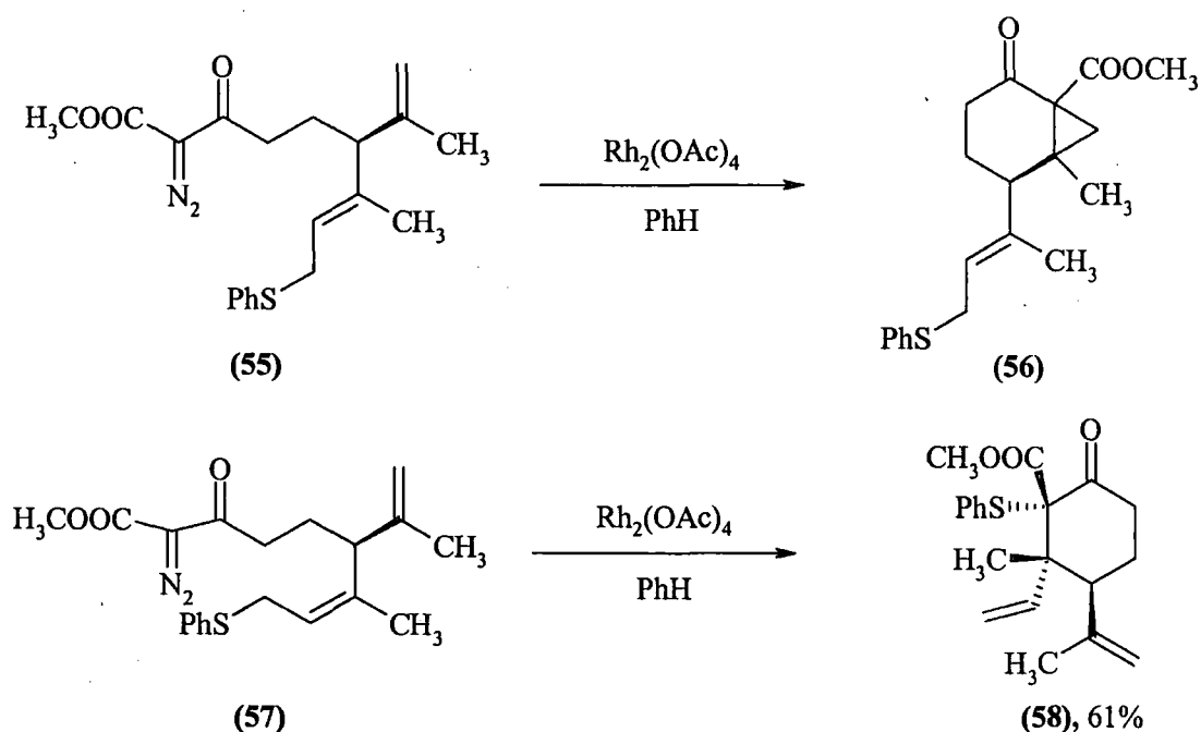
Scheme 1.35
