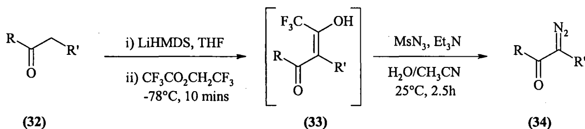
Scheme 1.15
