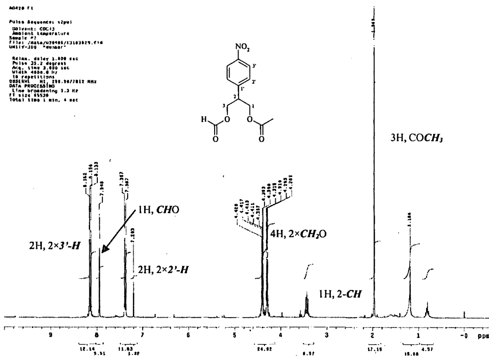
1 H NMR spectrum of 3-formyl-2-(4'-nitro)-propyl acetate (62)
