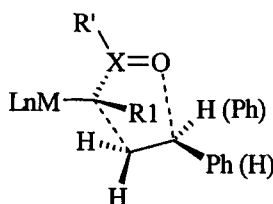
Scheme 1.25
