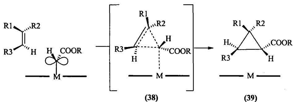
Scheme 1.21
