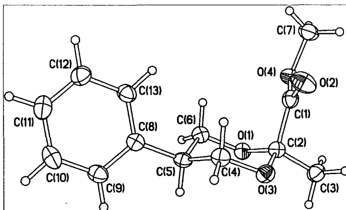
Scheme 3.17
