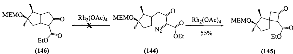
Scheme 1.78
