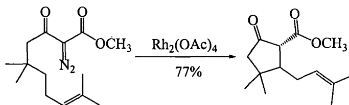
Scheme 1.83
