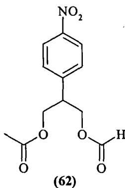
Scheme 3.36
