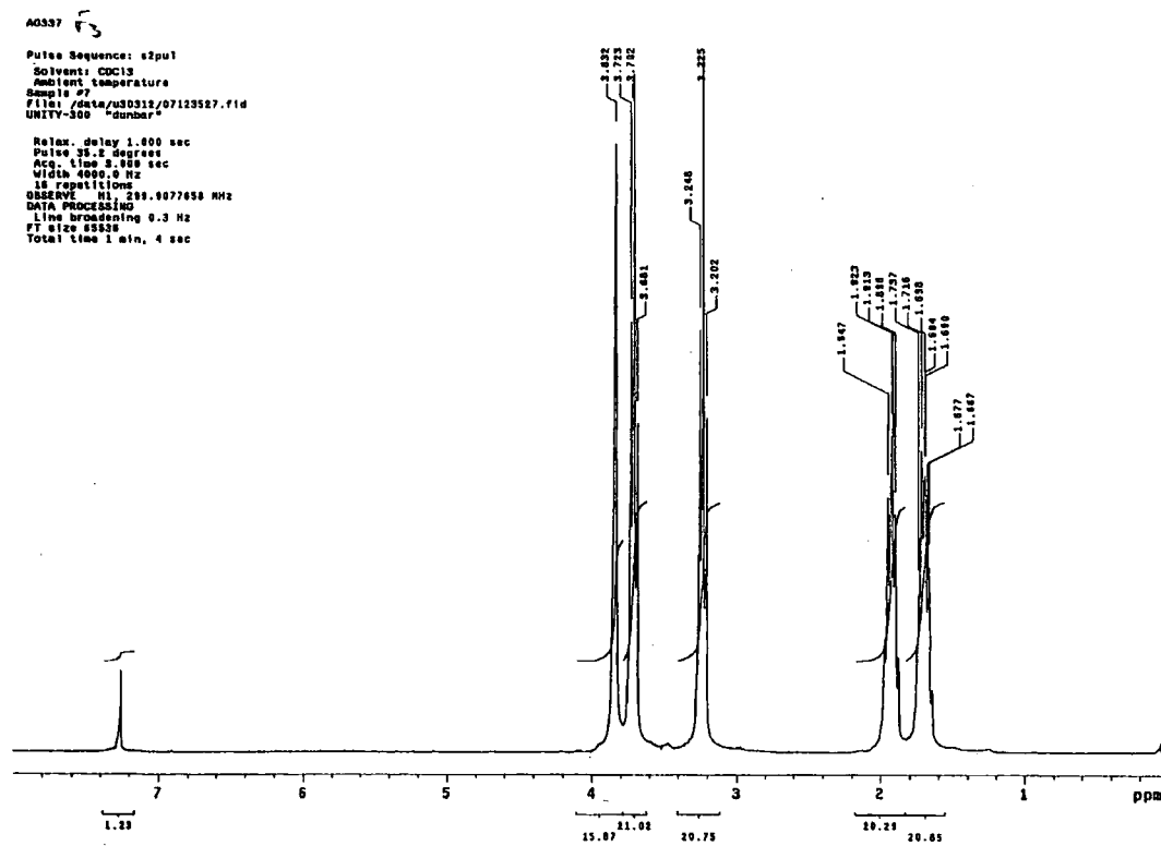
1 H spectrum of a by-product of the SmI 2 reaction.
