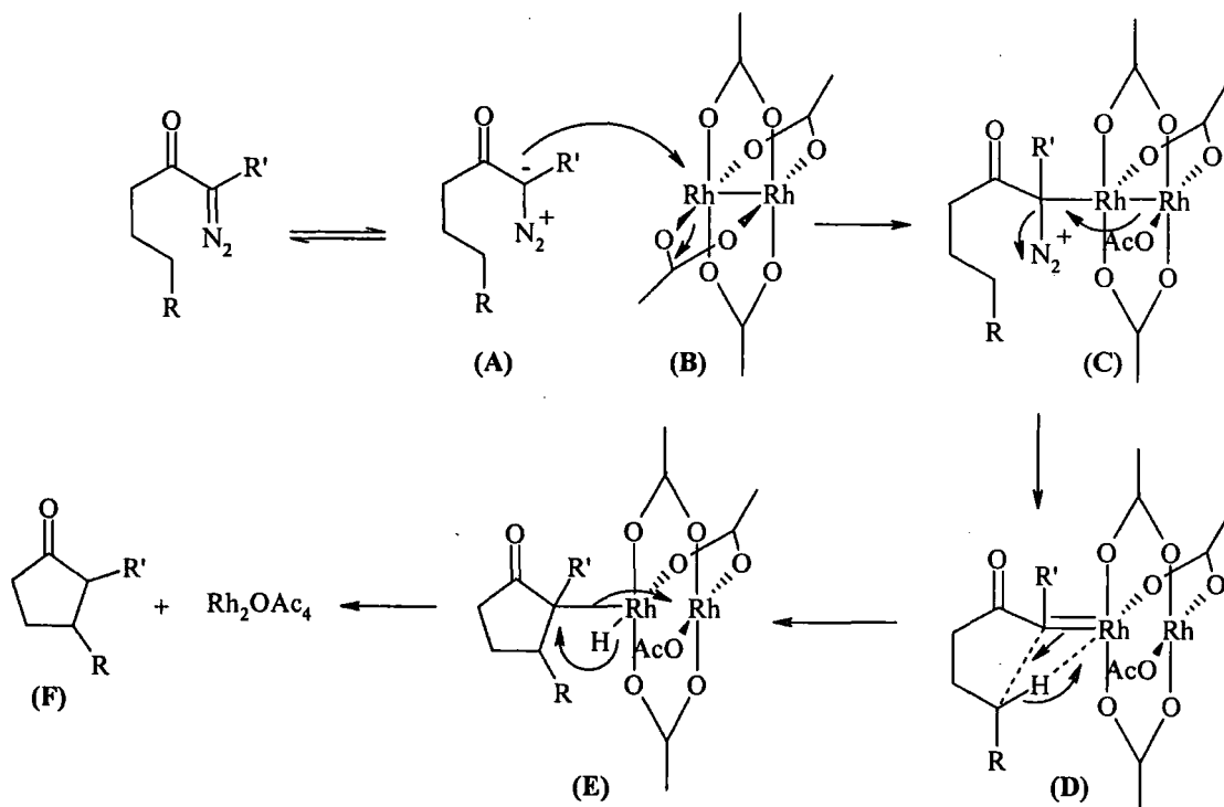
Scheme 1.76
