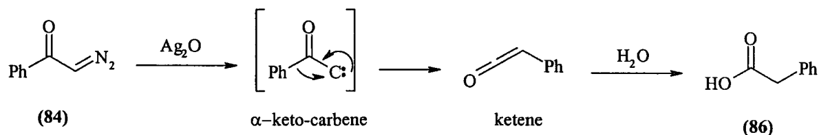
Scheme 1.47
