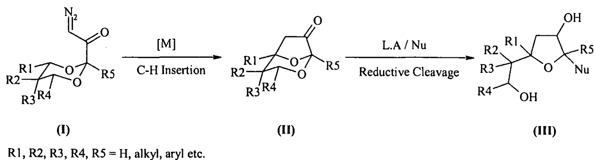
Scheme 1.2
