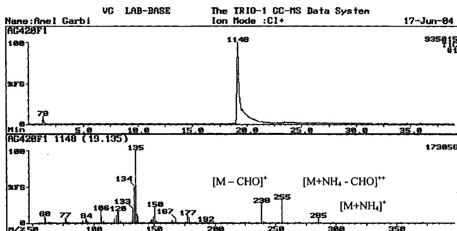
GC/MS spectrum of 3-formyl-2-(4'-nitro)-propyl acetate (62)
