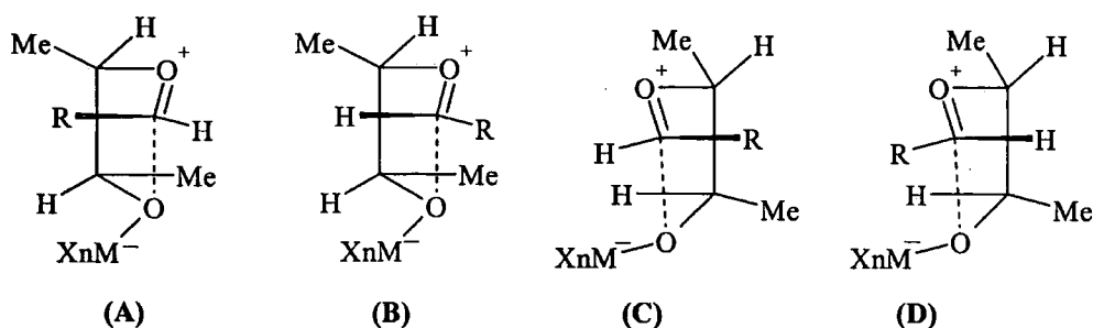
Scheme 4.7
