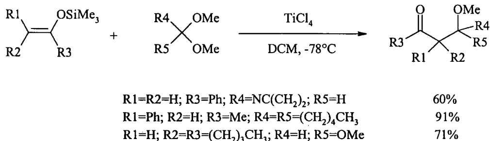
Scheme 4.2
