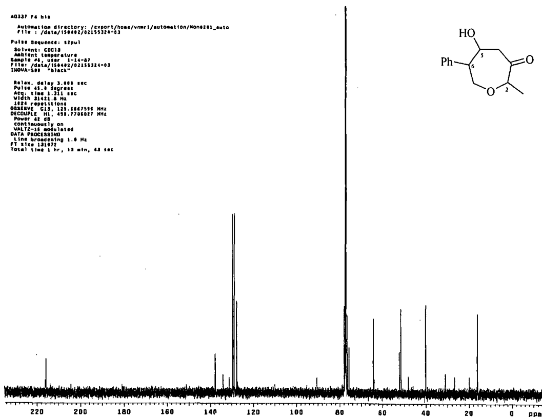
13 C NMR spectrum of 5-hydroxy-2-methyl-6-phenyl-oxepan-3-one.
