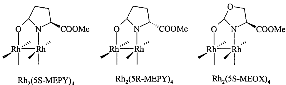
Scheme 1.91
