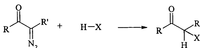
Scheme 1.53
