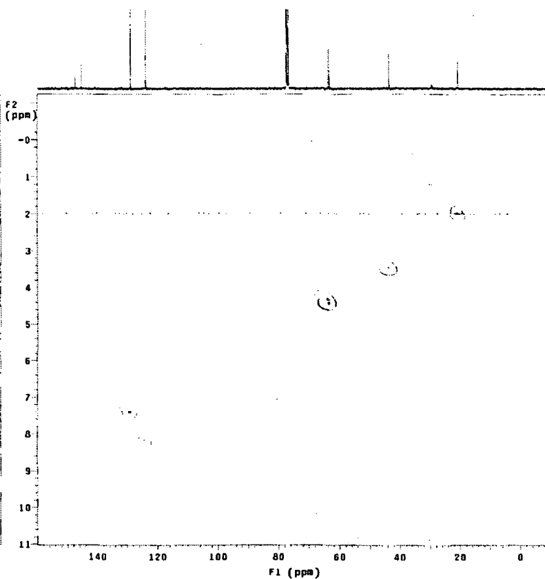
HSQC spectrum of 3-formyl-2-(4'-nitro)-propyl acetate (62)
