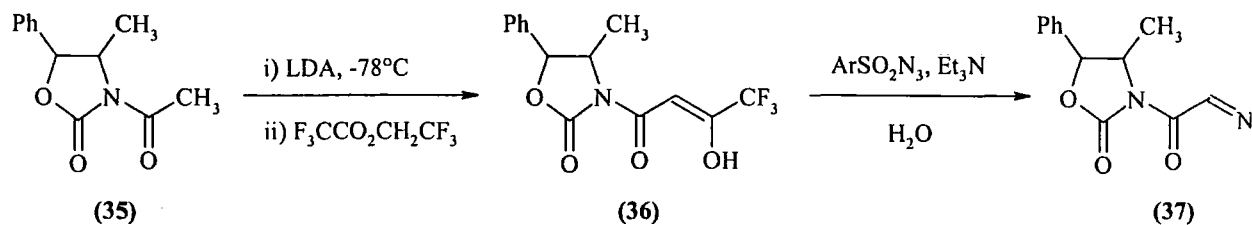
Scheme 1.16
