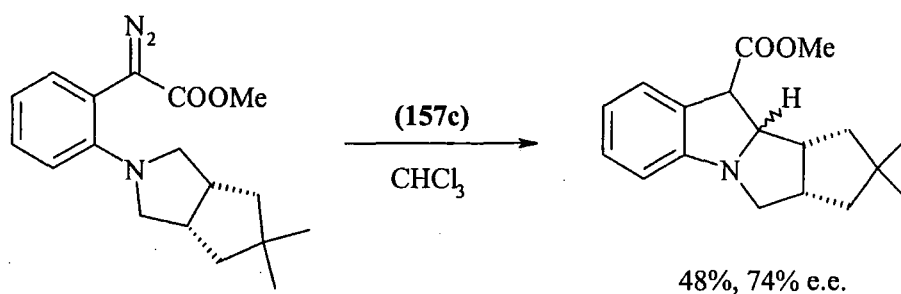
Scheme 1.89
