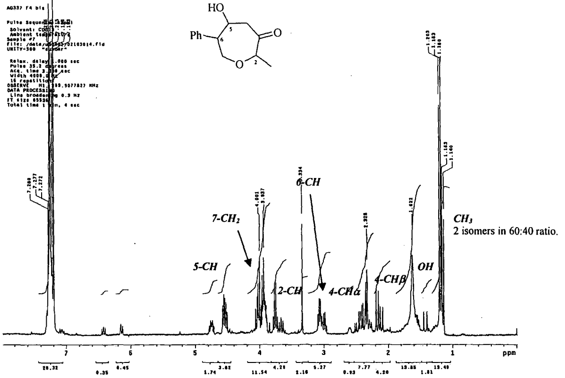
1 H NMR spectrum of 5-hydroxy-2-methyl-6-phenyl-oxepan-3-one. (Sm 2 reaction product)
