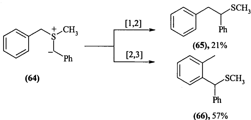
Scheme 1.39
