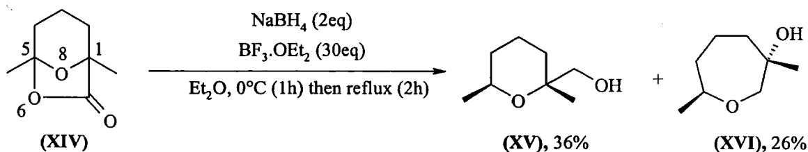
Scheme 4.19
