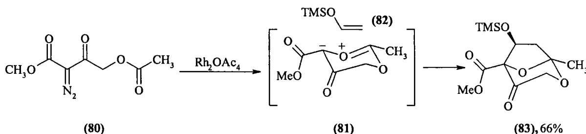
Scheme 1.45
