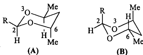
Scheme 4.10
