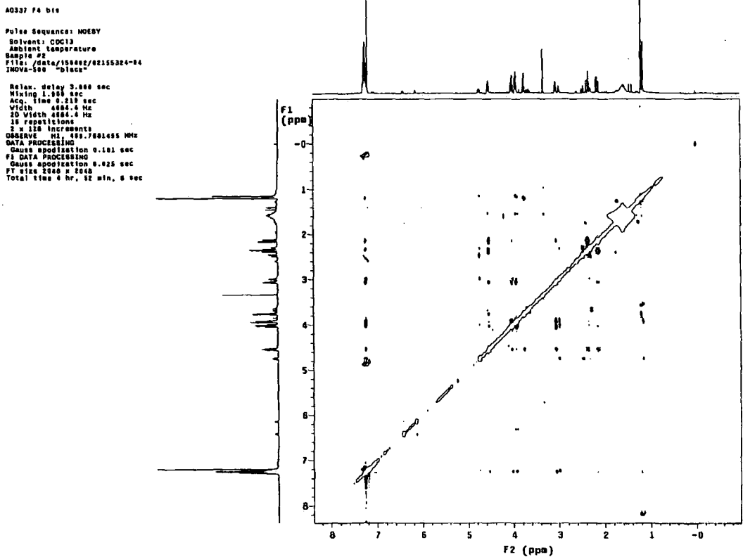
NOESY spectrum of 5-hydroxy-2-methyl-6-phenyl-oxepan-3-one.
