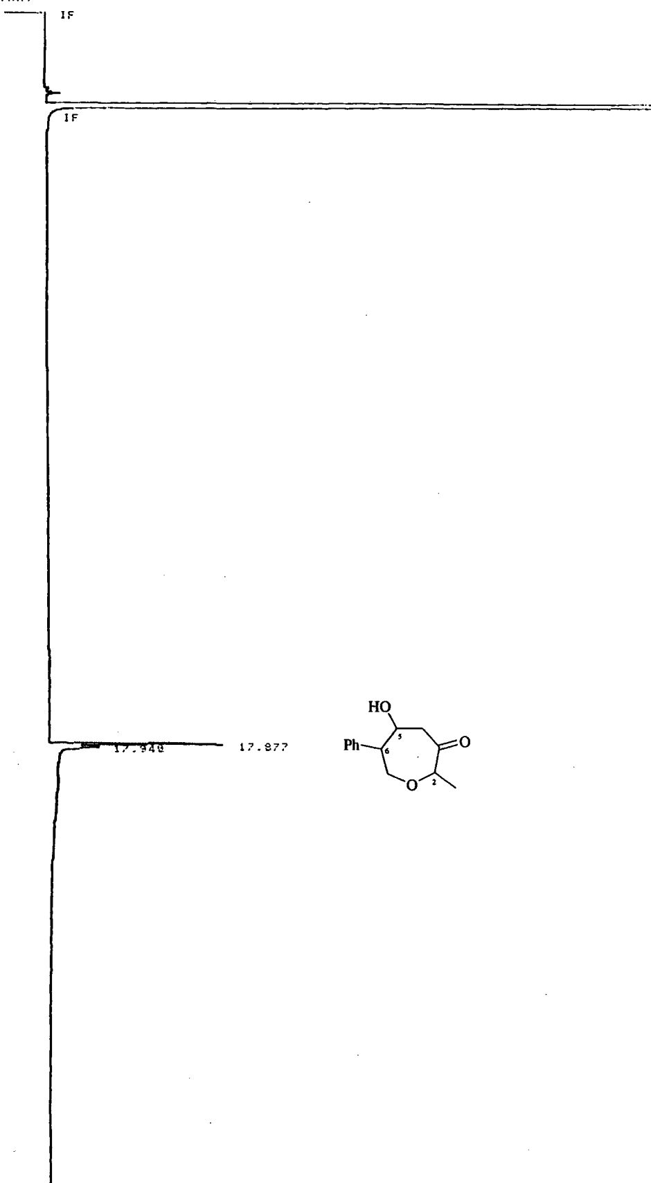
GC spectrum of 5-hydroxy-2-methyl-6-phenyl-oxepan-3-one (2 isomers).
