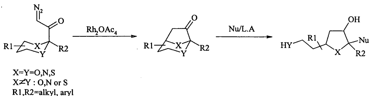
Scheme 5.1
