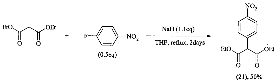
Scheme 3.7
