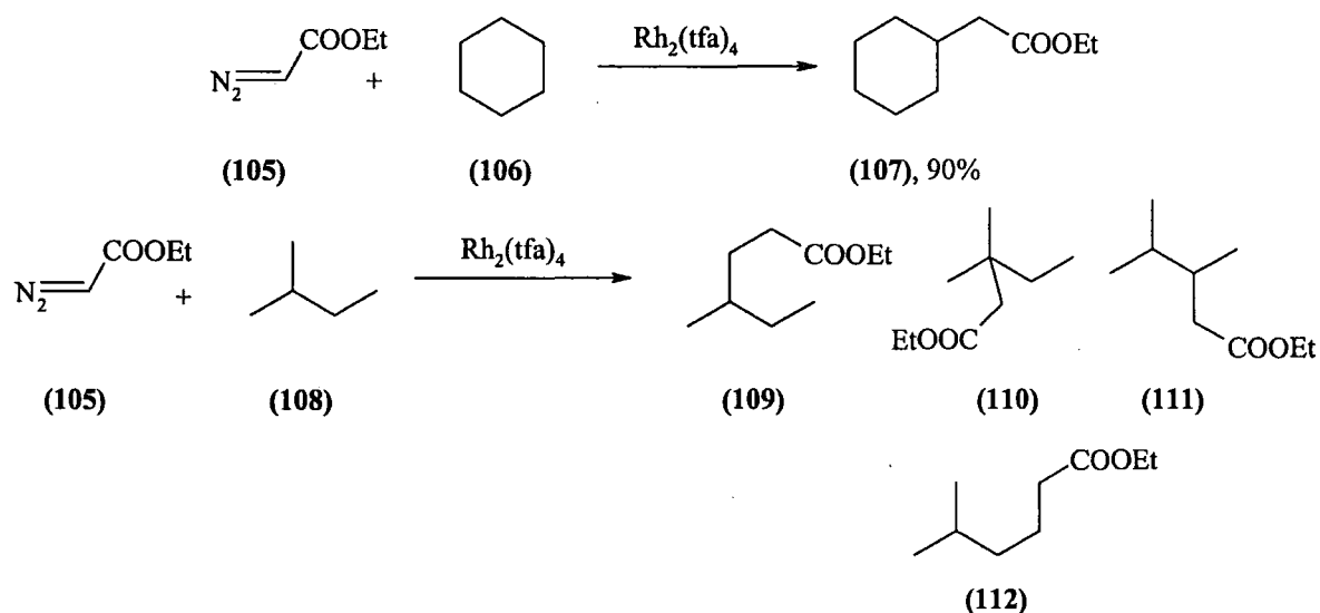
Scheme 1.57
