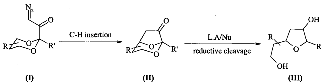
Scheme 1.93
