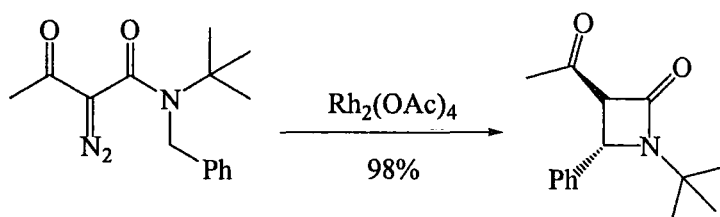
Scheme 1.81
