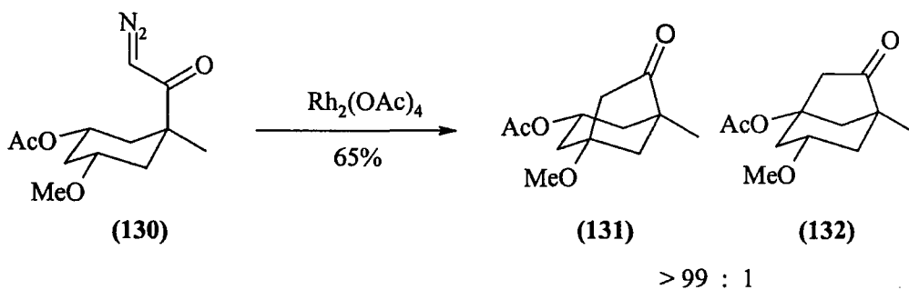
Scheme 1.71
