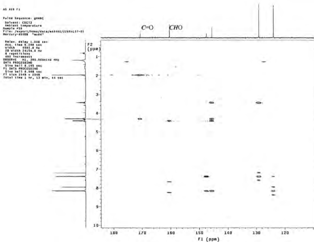
HMBC spectrum of 3-formyl-2-(4'-nitro)-propyl acetate ( 62 )
