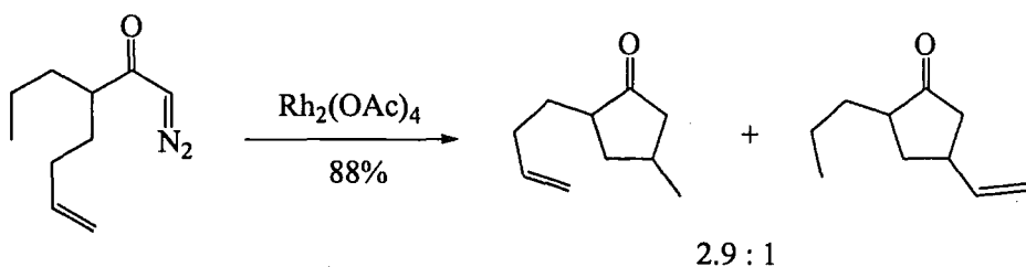
Scheme 1.68
