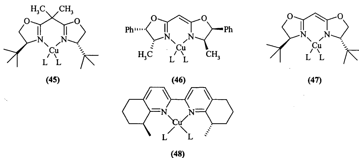
Scheme 1.26
