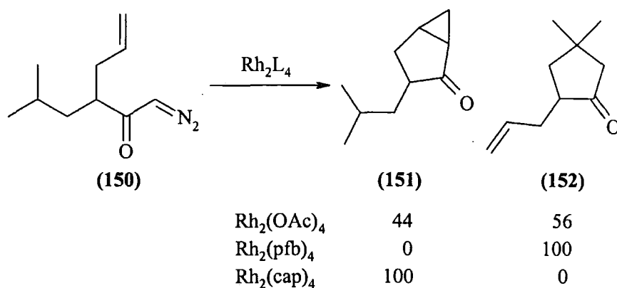
Scheme 1.85
