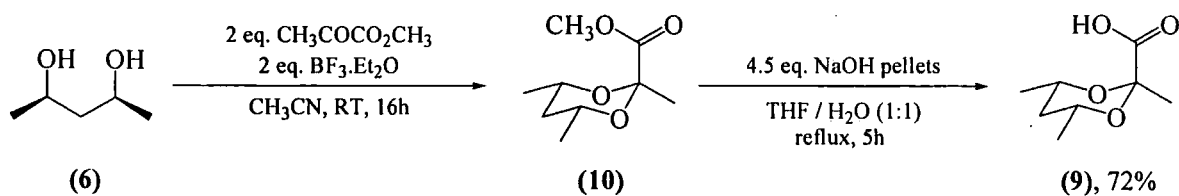
Scheme 2.10
