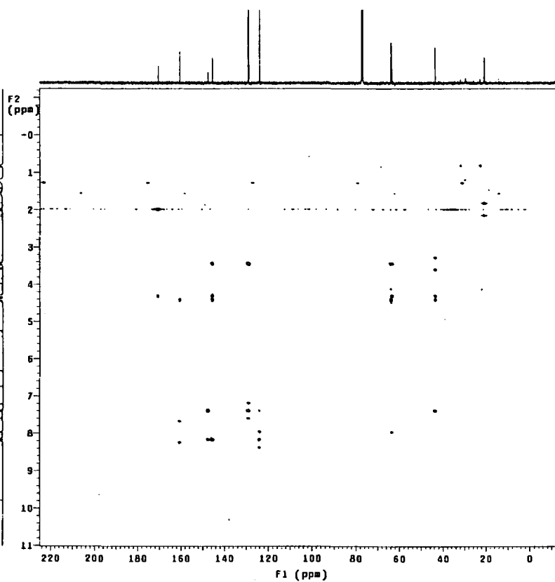
HMBC spectrum of 3-formyl-2-(4'-nitro)-propyl acetate (62)
