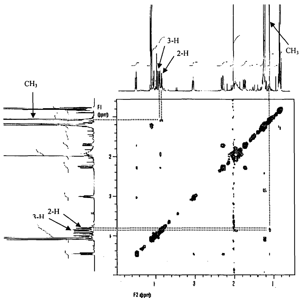
Scheme 4.40
