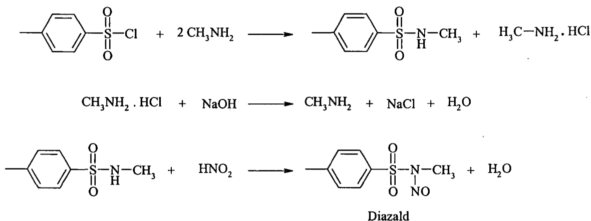
Scheme 3.23
