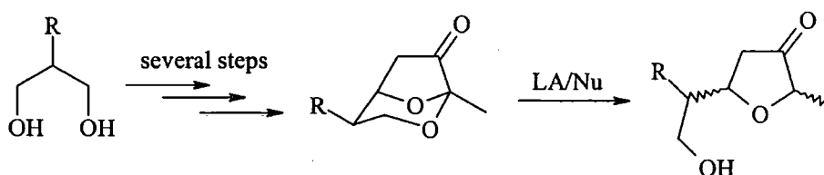
Scheme 4.1
