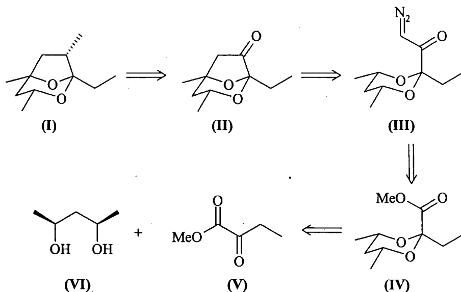
Scheme 2.20
