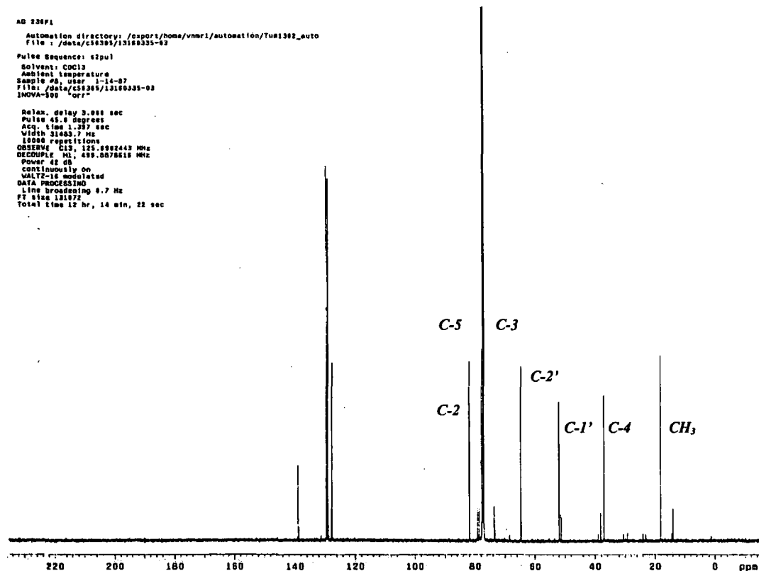
^{13}\text{C} NMR spectrum of 5-(2'-hydroxy-1'-phenyl-ethyl)-2-methyl-tetrahydrofuran-3-ol (68,69). (for comparison with the oxepane spectrum)
