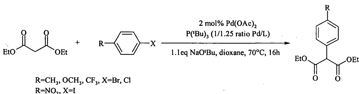
Scheme 3.5
