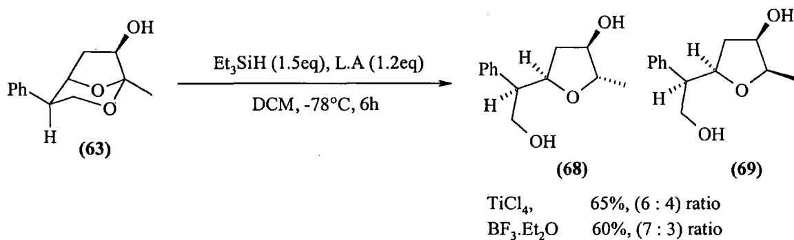
Scheme 4.39
