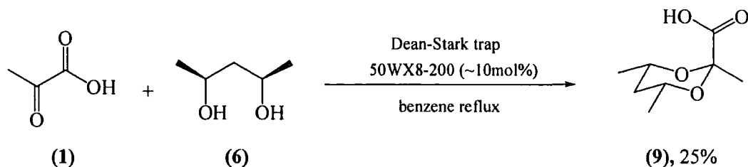
Scheme 2.7
