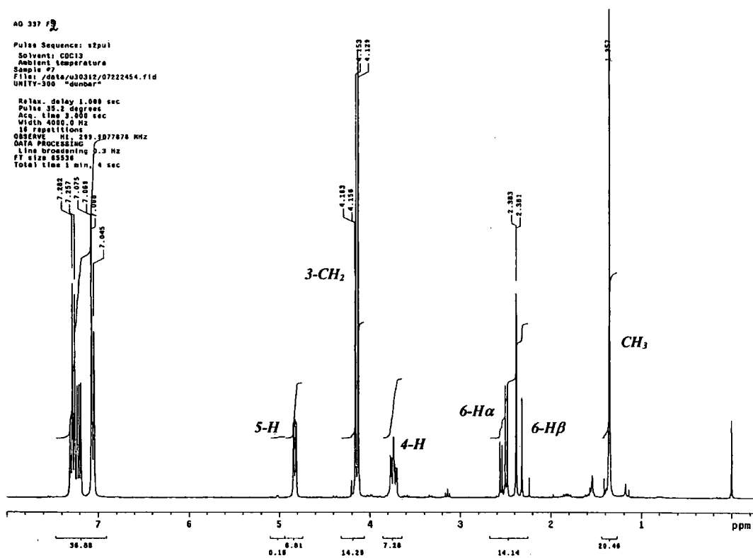
1 H NMR spectrum of 1-methyl-4-phenyl-2,8-dioxa-bicyclo[3.2.1]octan-7-one ( 56 ). (starting material recovered after reaction).
