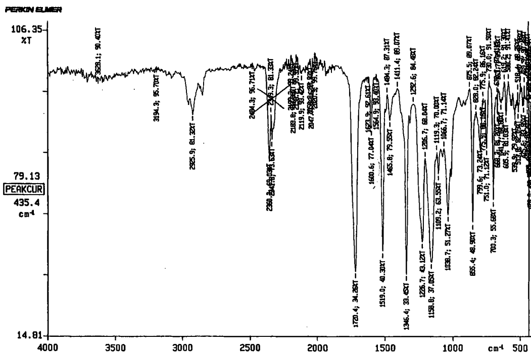
IR spectrum of 3-formyl-2-(4'-nitro)-propyl acetate (62)
