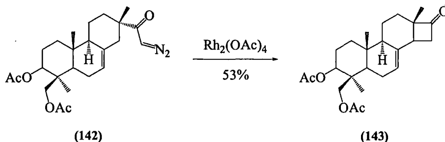
Scheme 1.77
