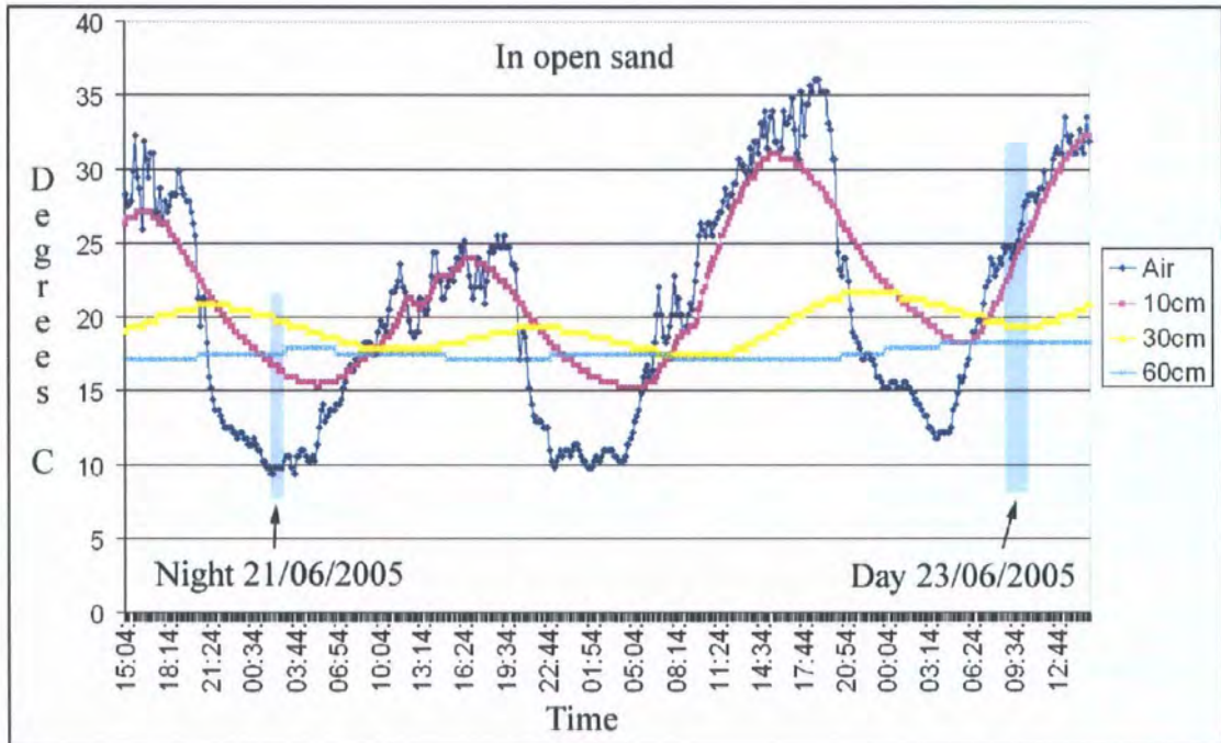
Figure 88 Temperature results (Hobo5) from 20/06/2005 to 23/06/2005
