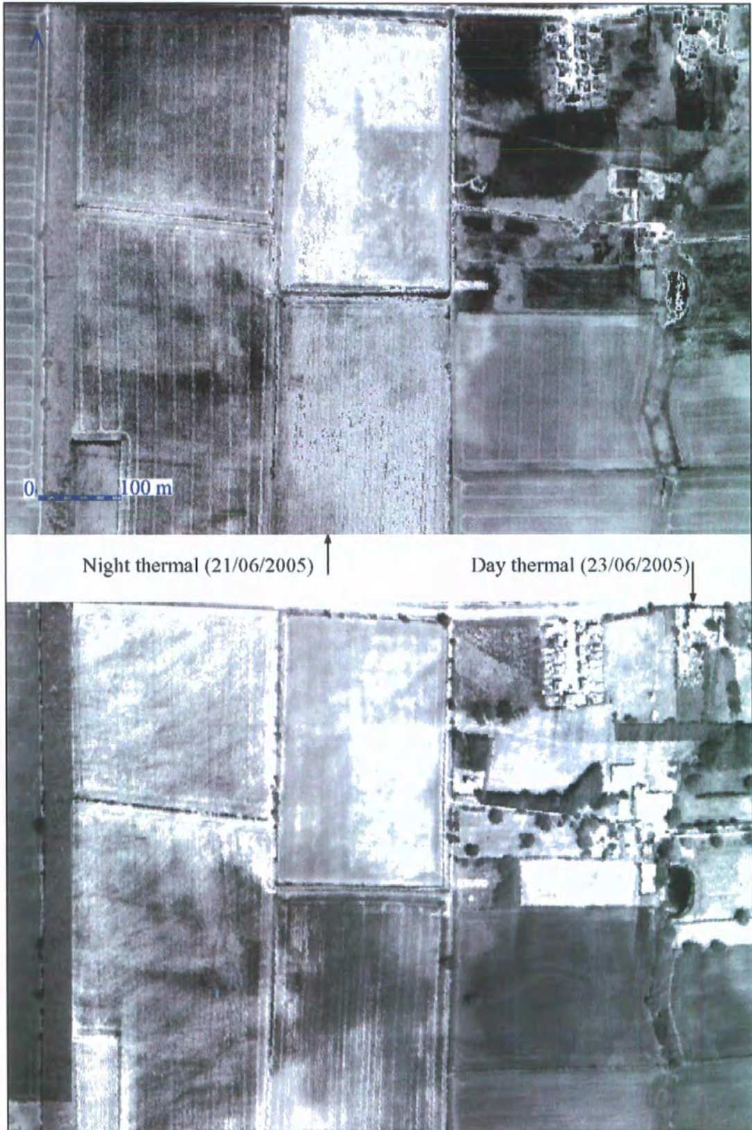
Figure 137 Thermal difference between night and day flights (AZ-16 ATM). Case study area 4 (south)
