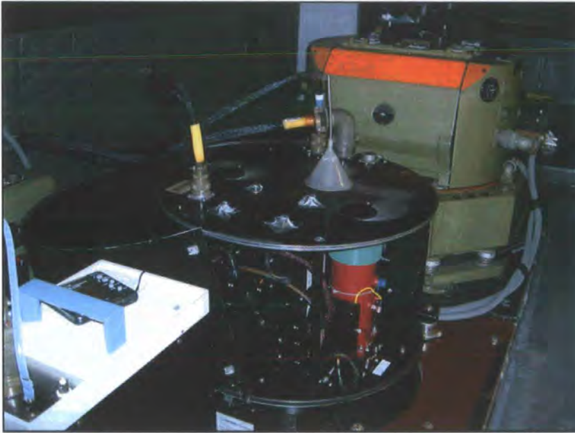
Figure 32 The internal workings of the AZ-16, with the CASI instrument in the foreground and the Wild RC10 in the background.
