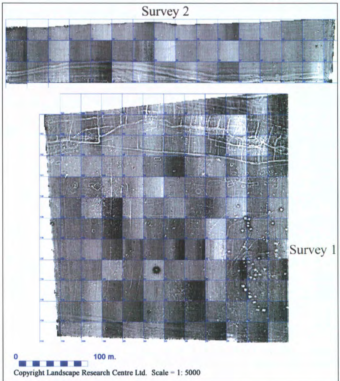
Figure 36 The raw gradiometer data from the two different surveyed areas carried out over Site 28
