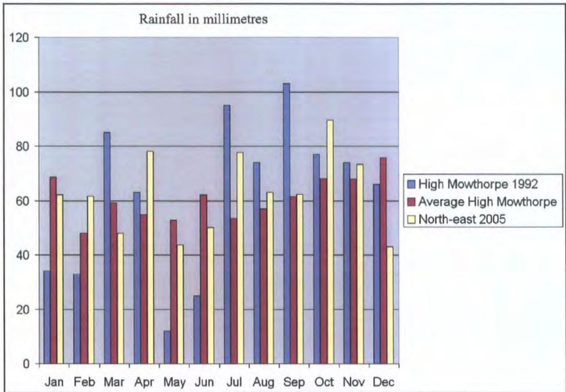
Figure 23 Rainfall per month in mm for 1992 and 2005 compared with the average rainfall from 1971 to 2001
