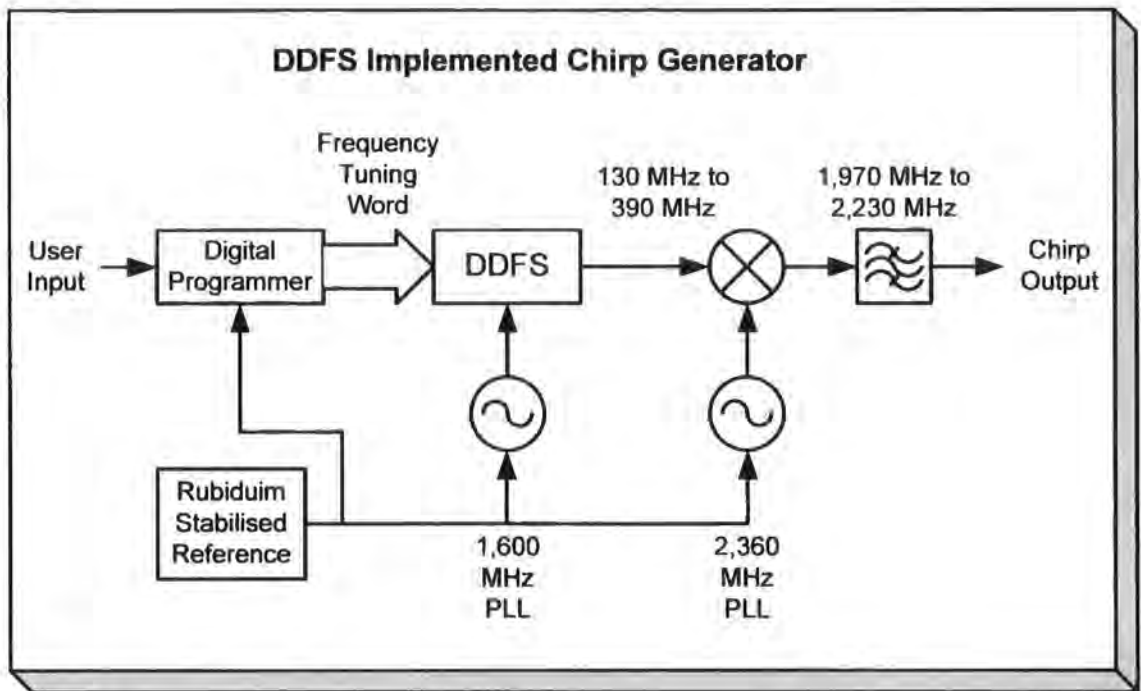
Figure 3.5 Chirp source and heterodyne up-converter
