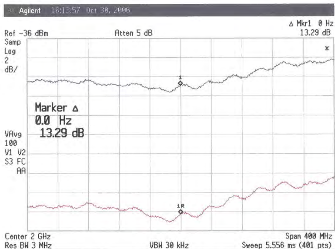
Figure 5.15 “y-factor” measurement of the 3.5 GHz down-converter
