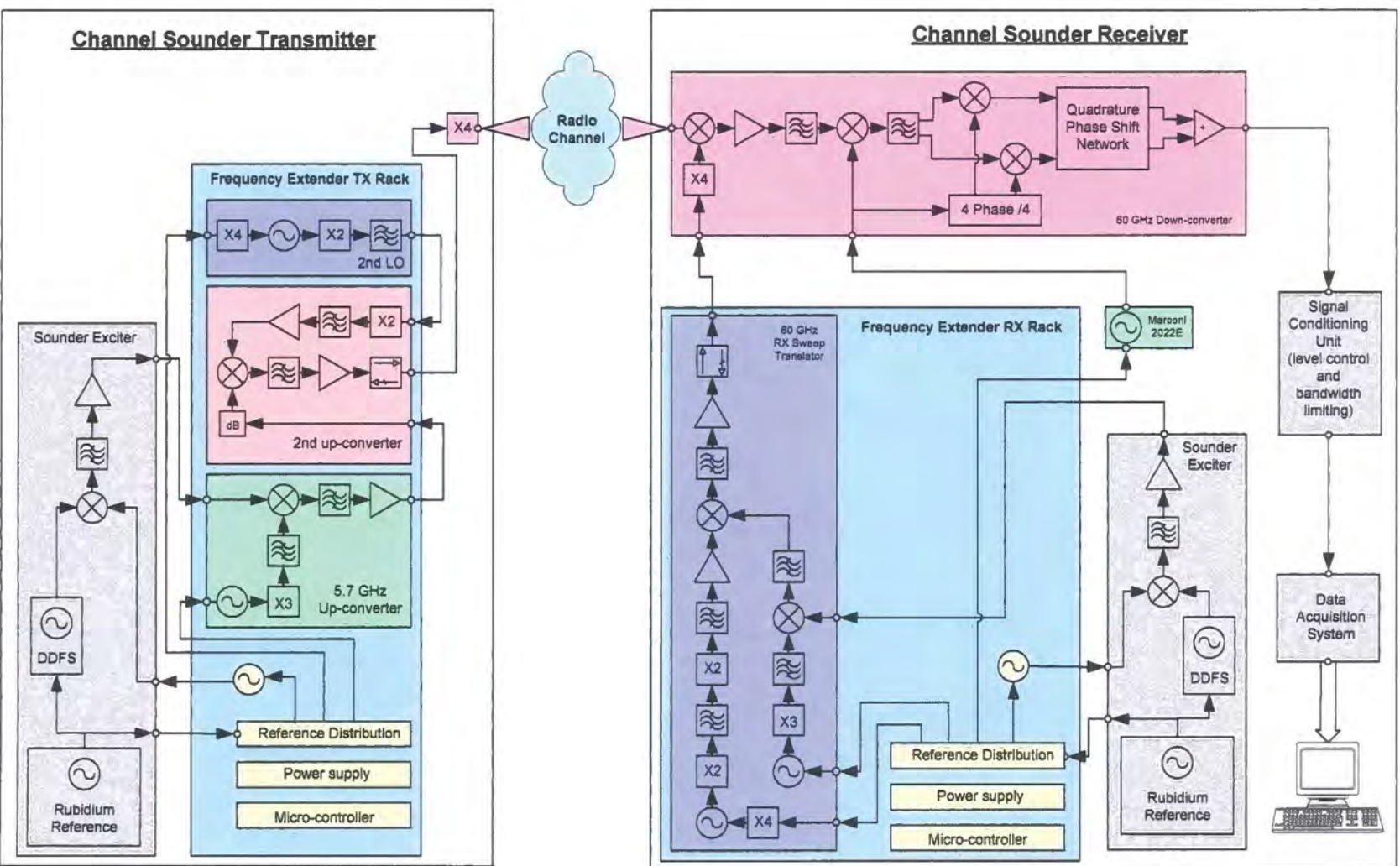
Figure 4.23 The 60 GHz channel sounder 4-38
