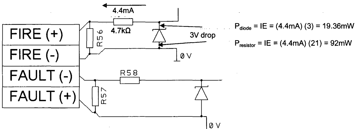
Figure 36 – Zener Inputs
