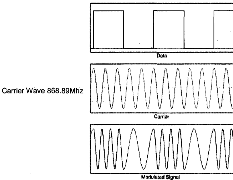
Figure 9 – FSK Modulation
