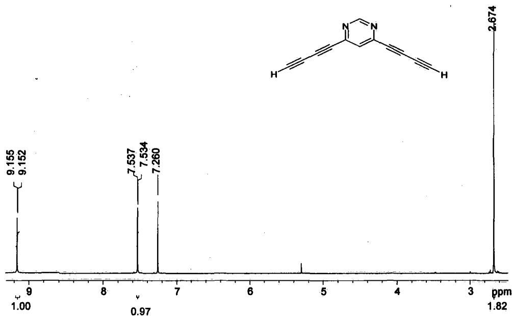
Fig III.1 ^1\text{H} NMR spectra of compound 214 in \text{CDCl}_3 at 400 MHz.
