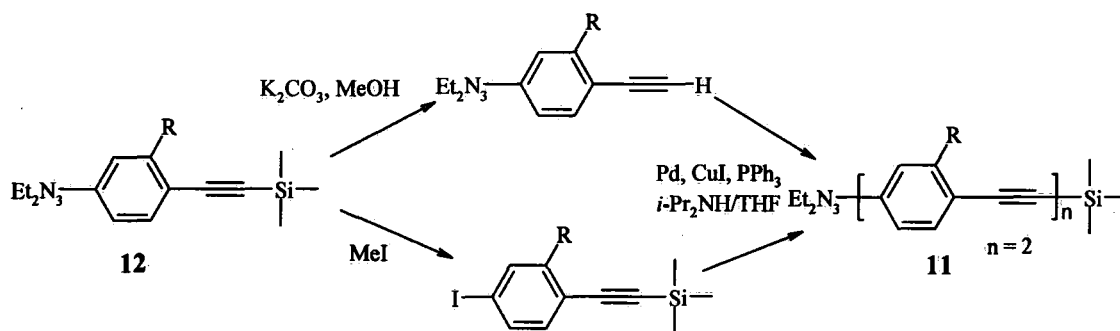
Scheme I.2 The iterative convergent/divergent approach.
