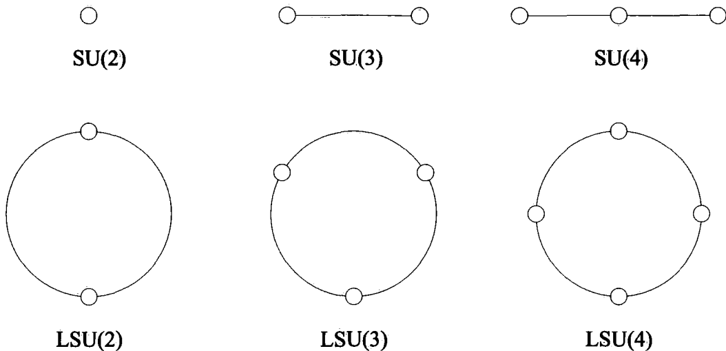
Figure 2.1: The Dynkin diagrams of various Lie groups and their loop groups
