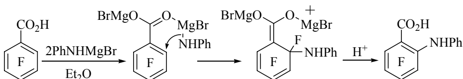
Scheme 6. 9 ortho substitution in pentafluorobenzoic acid
