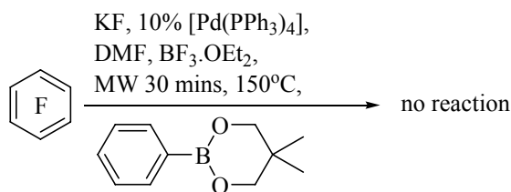
Scheme 47. Attempted C-F bond palladium activation with a Lewis Acid
