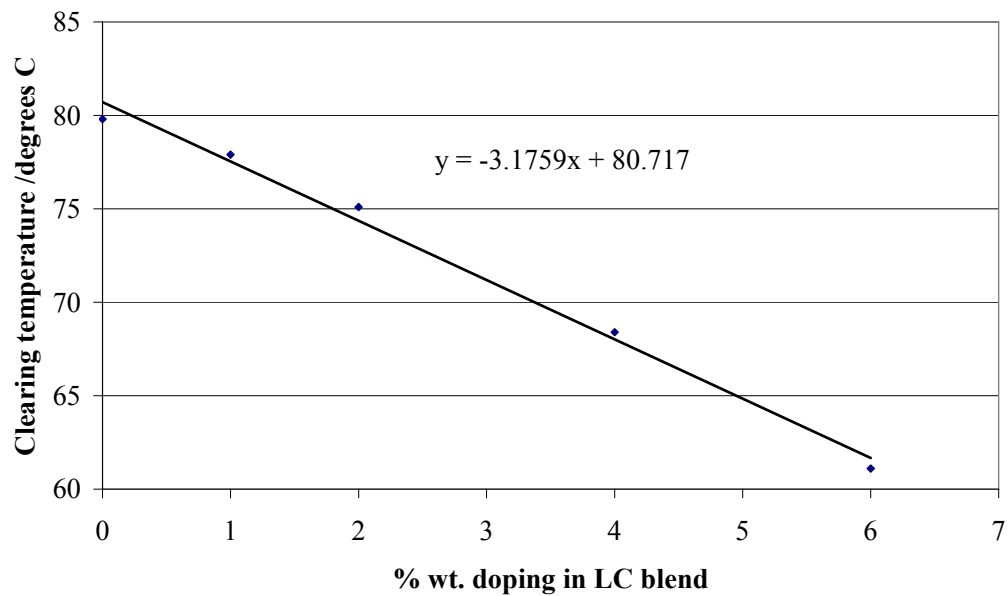
Graph 4. T_{NI} versus percentage doping of a dielectrically negative LC blend with 45 .
