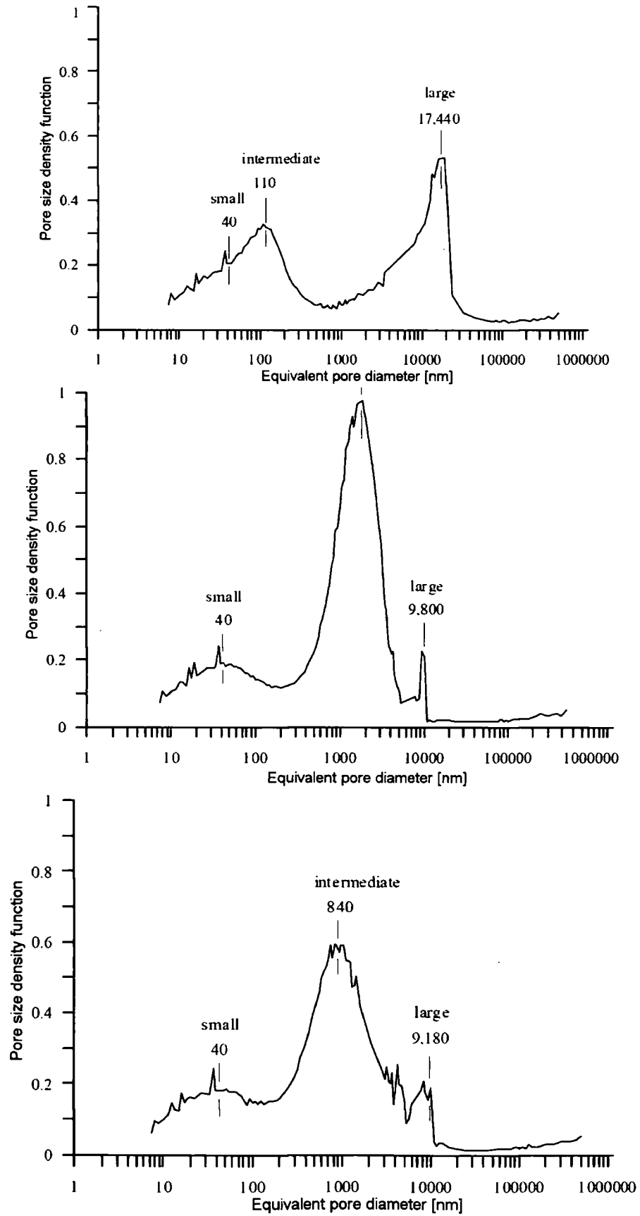
Figure 2.16. Fabric evolution during wetting: pore structure after compaction (top), after free swelling (middle) and after swelling under constant volume (bottom), after Monroy (2006).
