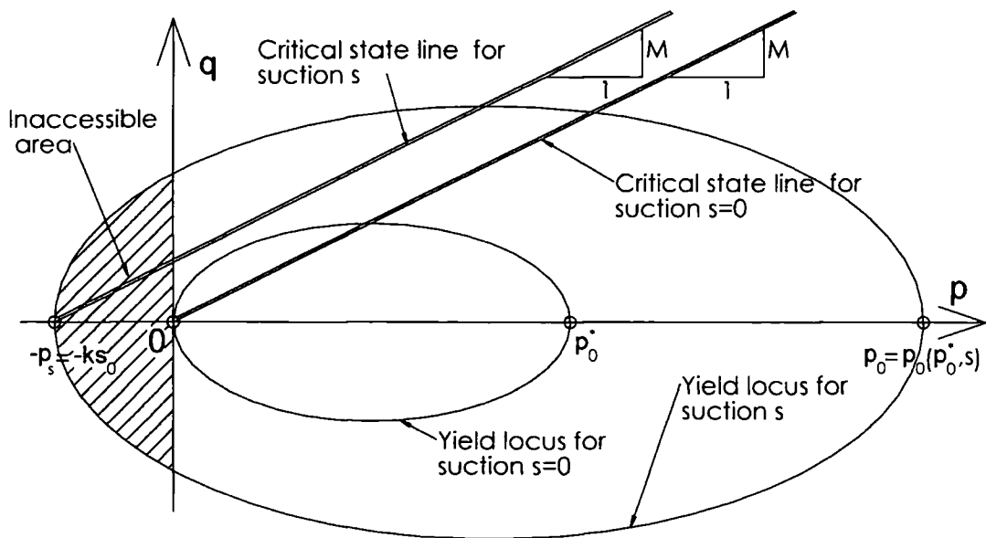
Figure 4.1. BBM yield locus. Note that the part of the yield locus left to the shear stress q axis is not accessible.
