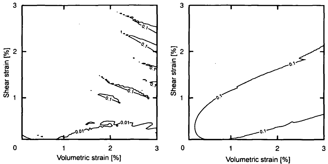
Figure 7.19. Percentage error in mean net stress integrated with explicit Modified Euler scheme (left) and advanced implicit algorithm (right). BBM parameters, strain increment, suction increment and initial stress state same as in Fig. 7.18. Data obtained by Solowski and Hofmann.
