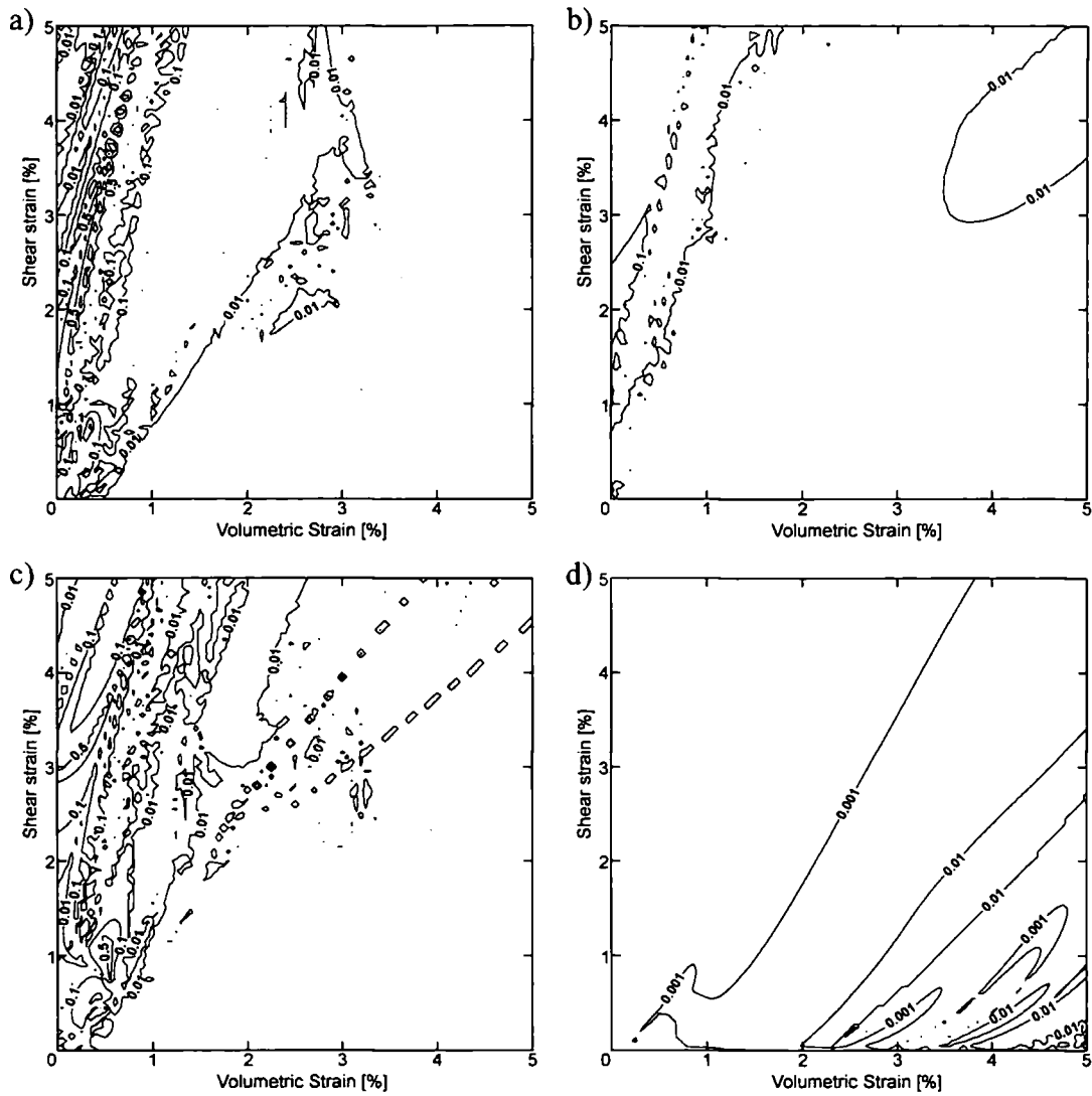
Figure 7.17. Error maps for EPUS error control. Percentage error in stresses integrated with: a) fourth order R-K method 4(3), b) England 5(4) c) Cash-Karp 5(4) and d) extrapolation method. In all cases the tolerance was set to 1%. Areas with error larger than 1% are greyed out.
