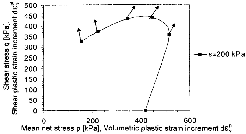
Figure 2.13. Plastic strain increment directions (after Estabargh and Javadi 2005).
