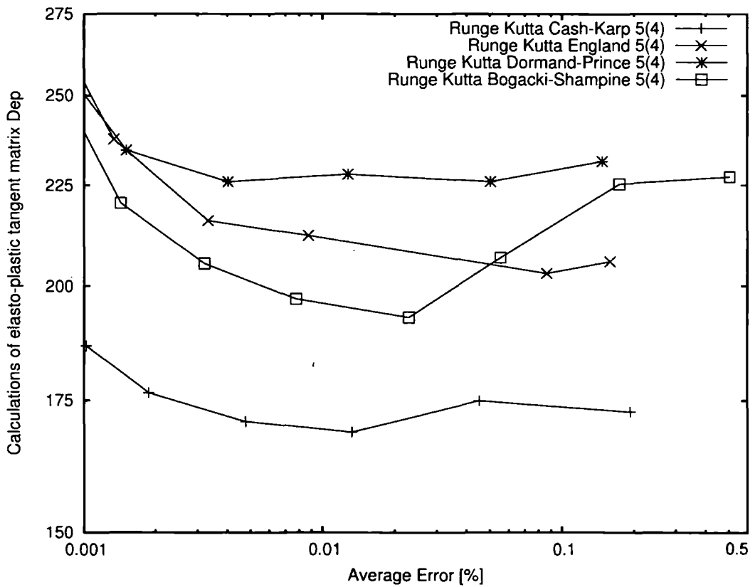
Figure 7.14. Comparison of efficiency for fifth order Runge-Kutta schemes with EPUS error control .
