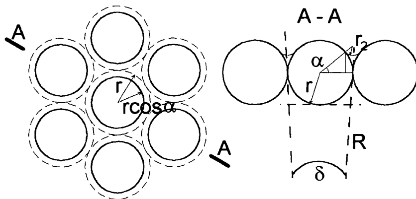
Figure 3.5. Fragment of surface and fragment of a cross-section of a spherical aggregate of radius R from Fig. 3.2 created from spherical grains of radius r .
