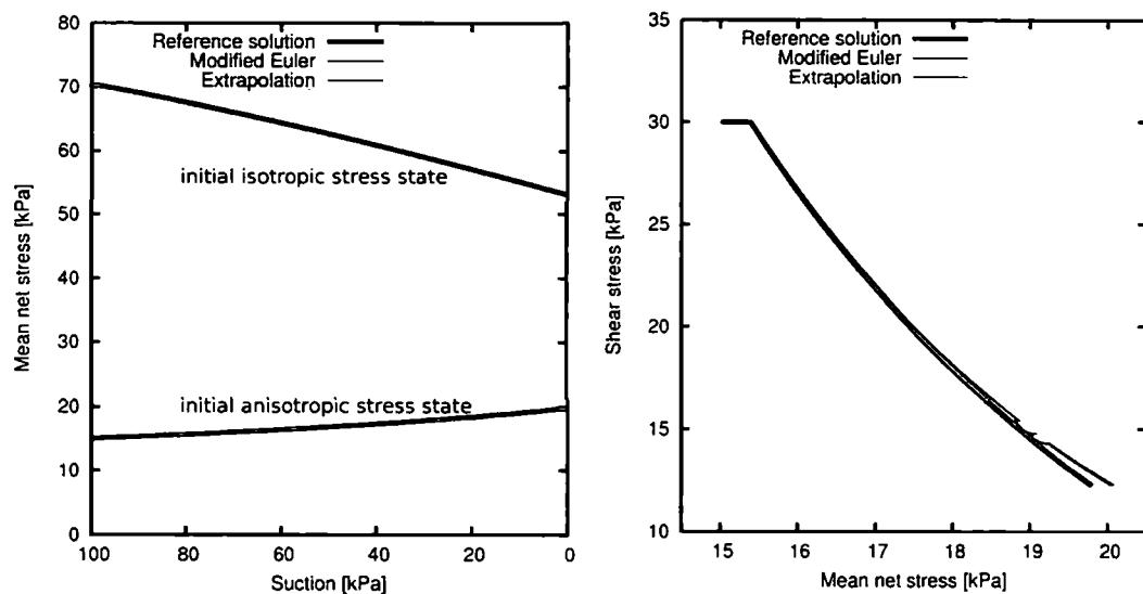
Figure 7.8. Isochoric wetting starting from both initial isotropic and anisotropic stress states: mean net stress versus suction (left) and shear stress versus mean net stress (right).
