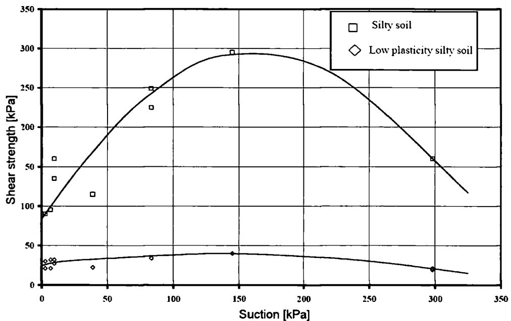
Figure 2.10. Shear strength of silty/ low plasticity silty soil (after Monroy 2005, data from Nishimura and Toyota 2002).
