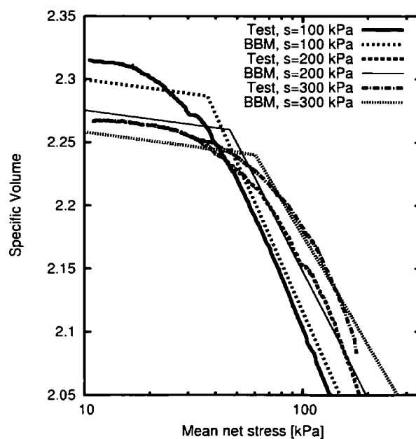
Figure 5.7. BBM approximation of experimental data. Data after Sharma (1998).
