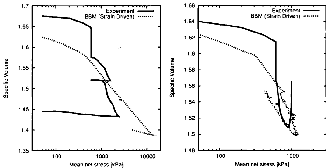
Figure 4.4. Simulation of an oedometric test EDO-1 (left), and shear test IWS-NC-02 (right). Only strain driven simulation is presented.
