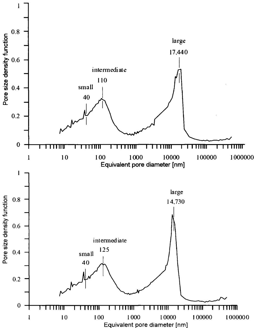
Figure 2.9. Pore size distribution at the initial state (top) and after mean net stress loading (bottom) at constant water content for compacted London Clay (after Monroy 2005).
