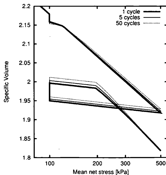
Figure 5.12. Random multi-cell enhanced BBM (RMC-BBM) with one, five and fifty wetting and drying cycles. The MC-BBM solution is equal to RMC-BBM with one cycle.
