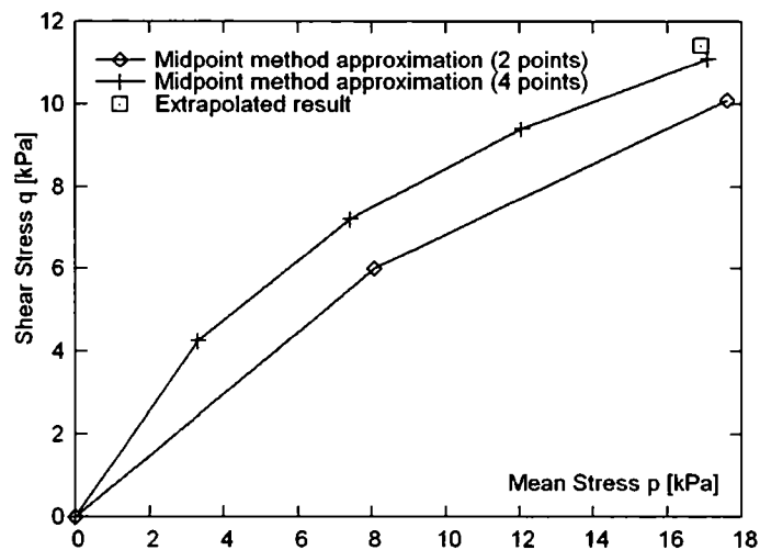
Figure 6.1. Extrapolation method: stress integrated with twice with constant subincrement size Midpoint method (with two and four subincrements) and the extrapolated result. Results obtained for error per step (EPS) error control.
