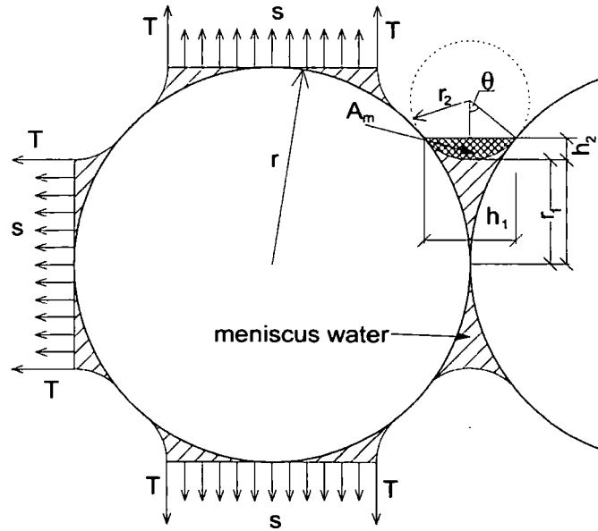
Figure 3.1. Forces acting on a soil grain in a simple cubic packing
