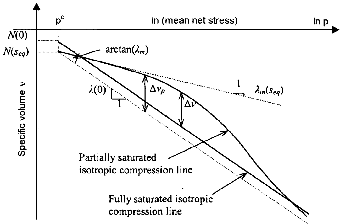
Figure 2.4. Schematic of isotropic compression line for fully saturated and partially saturated soil (after Georgiadis et al. 2005). The amount of collapse initially increases then reduces, in line with the results presented by Sun et al. (2007), see Fig. 2.5.
