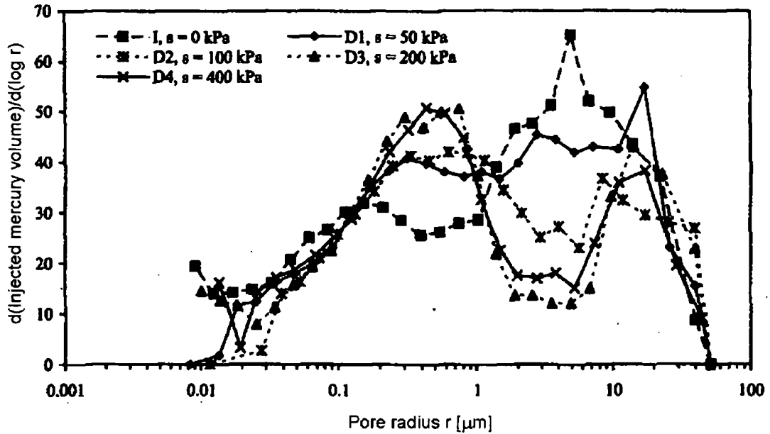
Figure 2.17. Fabric evolution during drying with suction increases from 0 up to 400 kPa (after Cuisinier and Laloui 2004).
