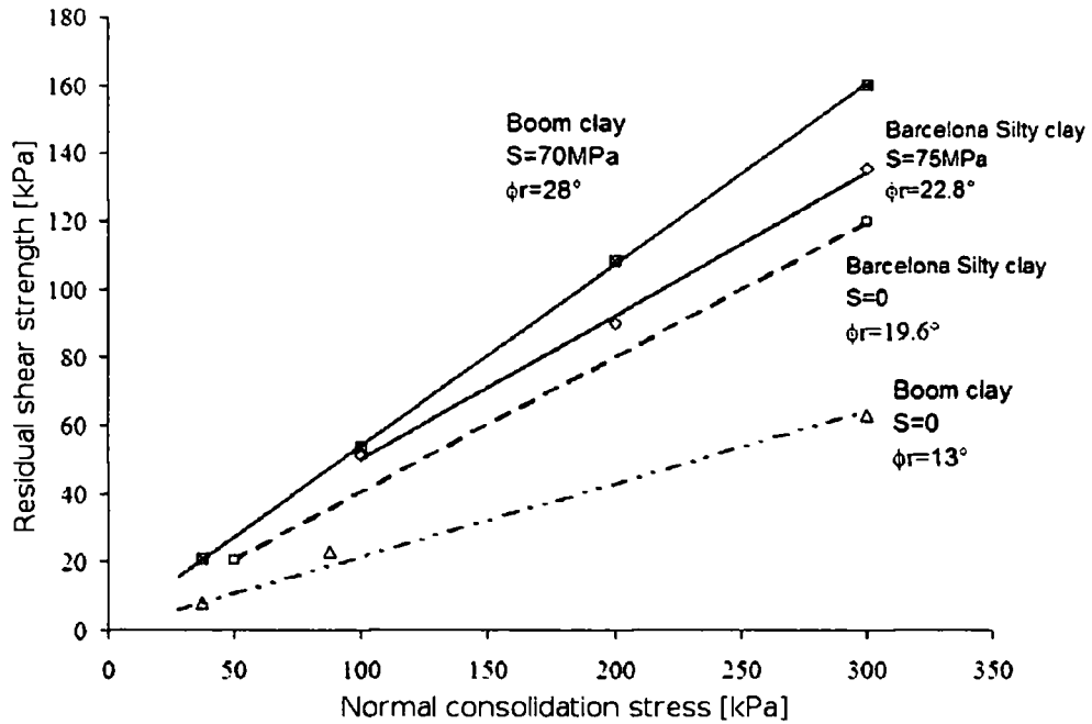
Figure 2.7. Residual shear resistance envelopes for saturated and unsaturated ( s=70\text{MPa} ) Boom clay and Barcelona silty clay (at s=75\text{MPa} , after Vaunat et al. 2007).
