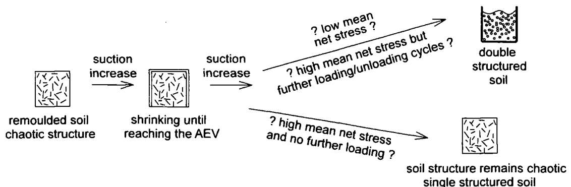
Figure 2.20. Hypothetical requirements for creation of double structured soil from remoulded state.
