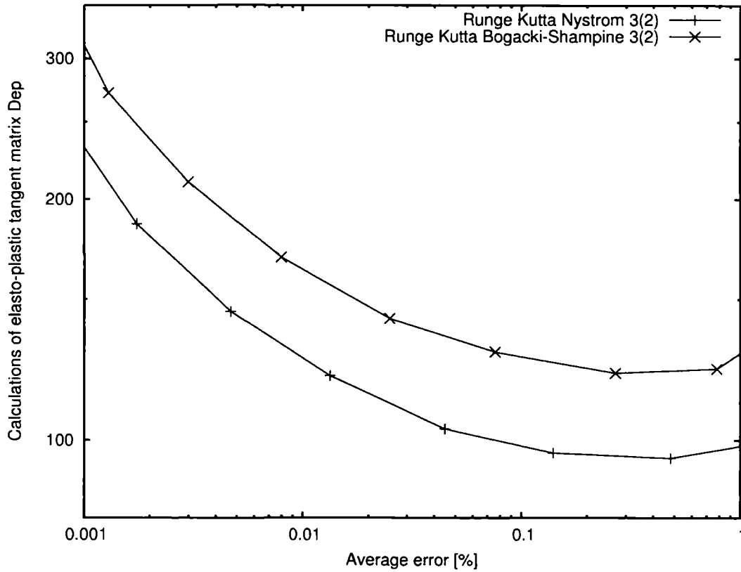
Figure 7.12. Comparison of efficiency for third order Runge-Kutta schemes with EPS control.
