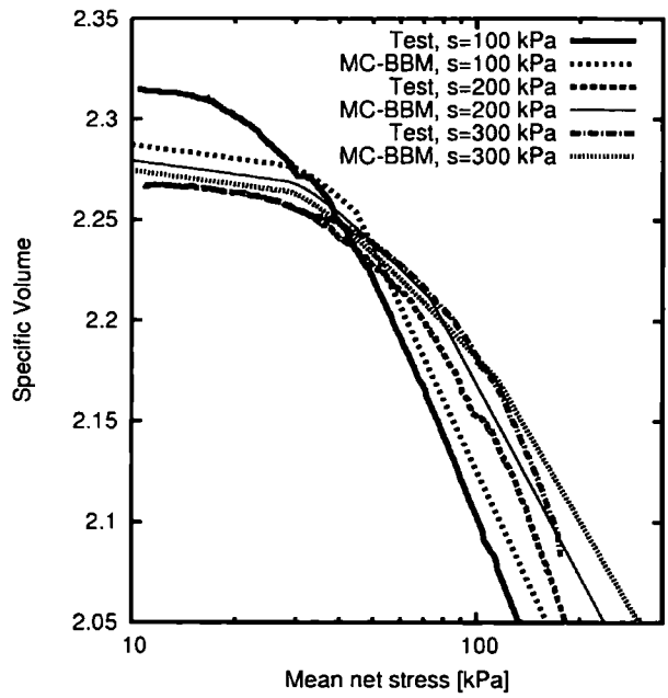
Figure 5.8. Multi-cell enhanced BBM (MC-BBM) approximation of experimental data. Data after Sharma (1998).
