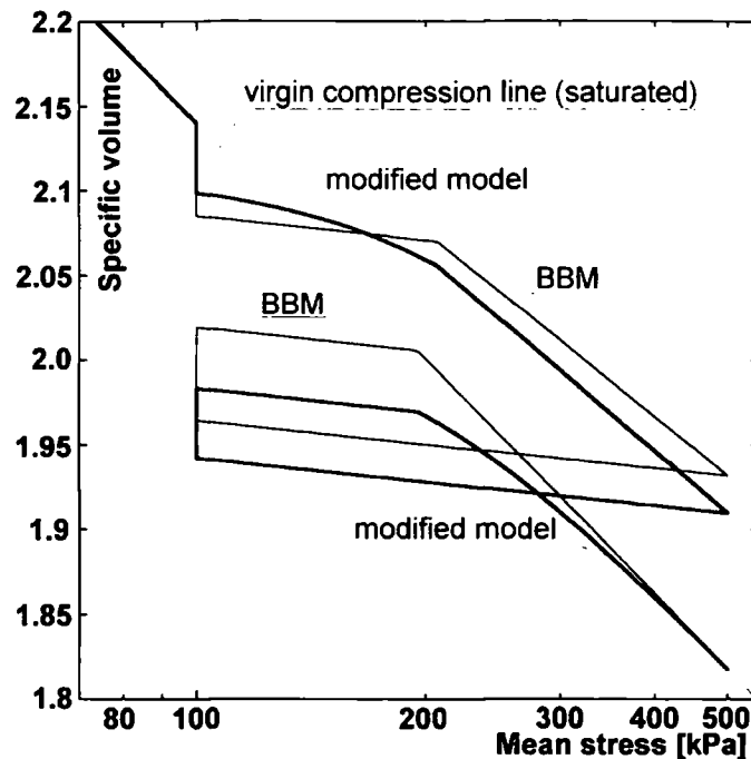
Fig. 5.6. Comparison of the modified BBM with the original formulation (for the same parameter set).
