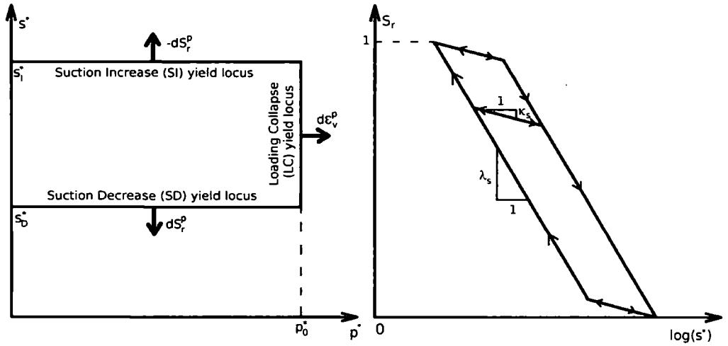
Figure 4.5. Yield locus and water retention behaviour of the Wheeler et al. (2003) model.
