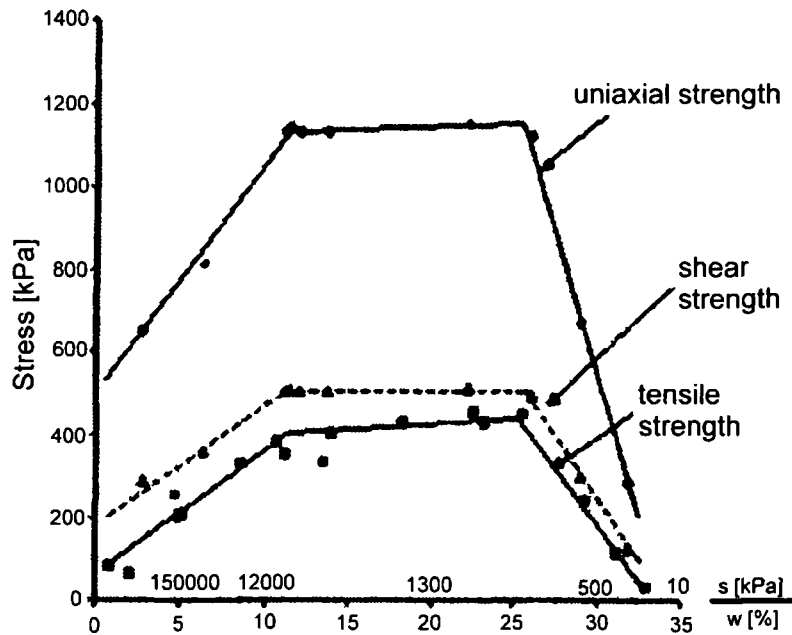
Figure 2.11. Shear strength and tensile strength of kaolinite clay with varying water content/suction. Suction values approximate (after Vesga and Vallejo 2006).
