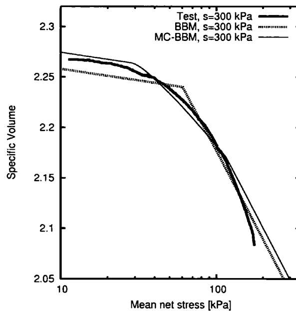
Figure 5.11. Multi-cell enhanced BBM (MC-BBM) and BBM approximation of experimental data. Data after Sharma (1998).
