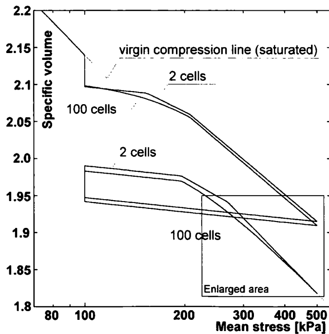
Figure 5.4. Influence of number of cells used in simulation: comparison between simulation with 2 and 100 cells
