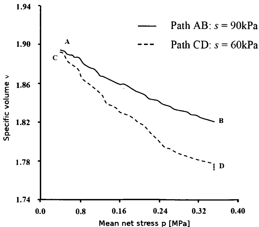
Figure 2.2. Virgin compression lines slopes for suction s=60 and s=90 kPa (after Alonso et al. 1990).
