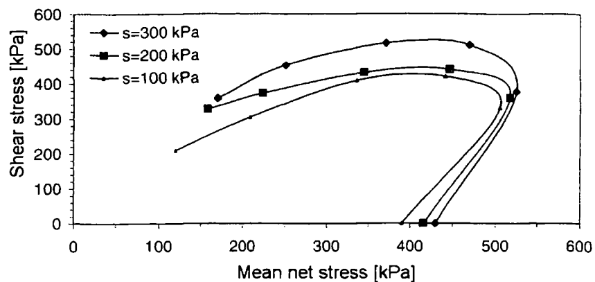
Figure 2.12. Yield locus shape for increasing suction (after Estabargh and Javadi 2005).
