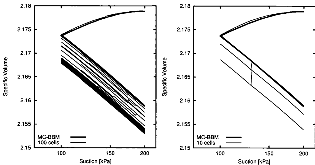
Figure 5.14. Random multi-cell enhanced BBM (RMC-BBM) modelling fifty wetting and drying cycles with 100 (left) and 10 (right) cells. The number of cells heavily influences the quality of model prediction (compare also Fig. 5.13 right). The MC-BBM solution is equal to RMC-BBM with one cycle – the difference in the figure is due to 1000 cells used in MC-BBM solution.
