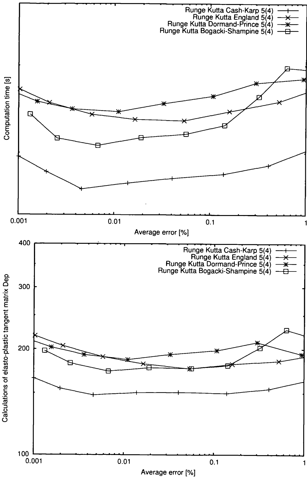
Figure 7.13. Comparison of efficiency for fifth order Runge-Kutta schemes with EPS error control.
