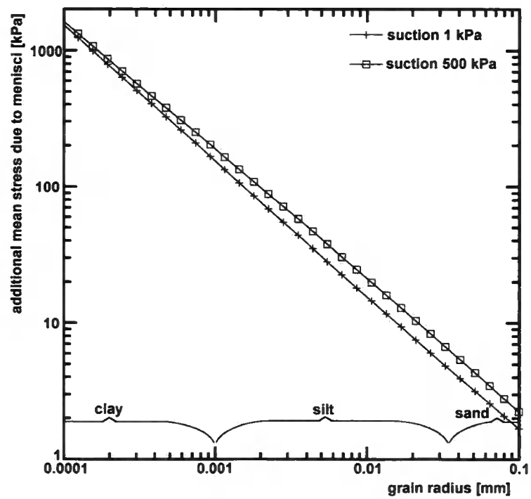
Figure 3.3. Mean net stress in menisci part of soil due to menisci forces. Simple cubic packing assumed
