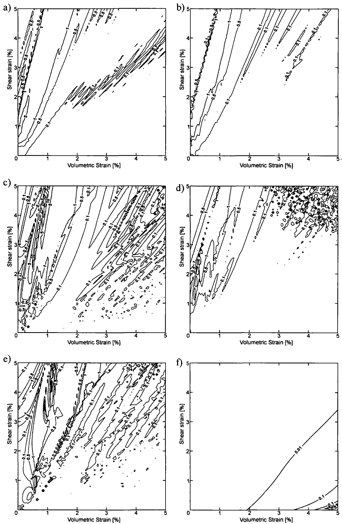
Figure 7.16. Error maps for EPS error control. Percentage error in stresses integrated with: a) Modified Euler 2(1), b) Nystrom 3(2) c) fourth order R-K method 4(3) d) England 5(4) e) Cash-Karp 5(4) f) extrapolation method. In all cases the tolerance was set to 1%. Areas with error larger than 1% are greyed out.
