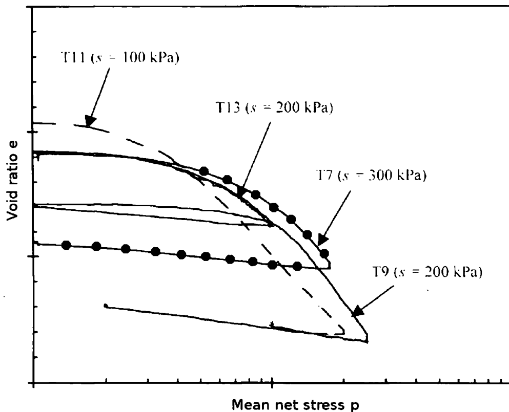
Figure 2.1. Increase in soil stiffness and resistance with suction increase under mean net stress loading (after Sharma 1998).
