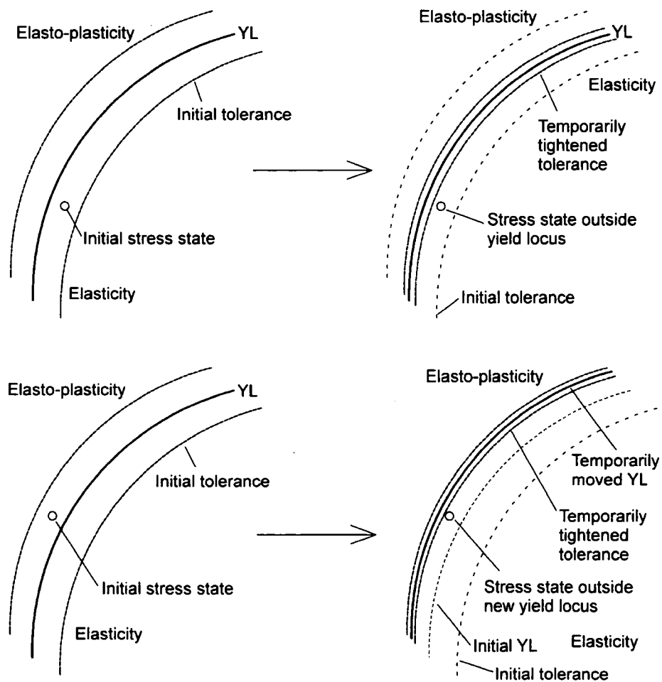
Figure 6.4. Graphical illustration of the modification of the yield tolerance during unloading-loading case for the Pegasus algorithm. Yield tolerance modified when the initial stress state lies on the elastic side of the yield locus (top). Yield tolerance modified and yield locus temporarily moved when the initial stress state lies on the elasto-plastic side of the yield locus (bottom).
