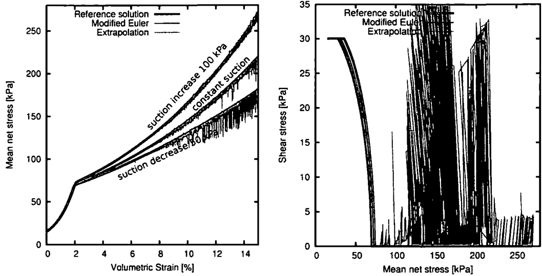
Figure 7.2. Isotropic loading at variable suction starting from an initial non-isotropic stress state with associated flow rule: mean net stress versus volumetric strain (left) and shear stress versus mean net stress (right).
