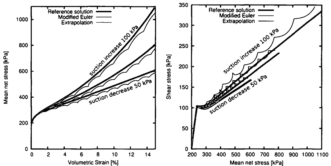
Figure 7.7. Oedometric loading at variable suction for slightly overconsolidated soil with non-associated flow rule: mean net stress versus volumetric strain (left) and shear stress versus mean net stress (right)
