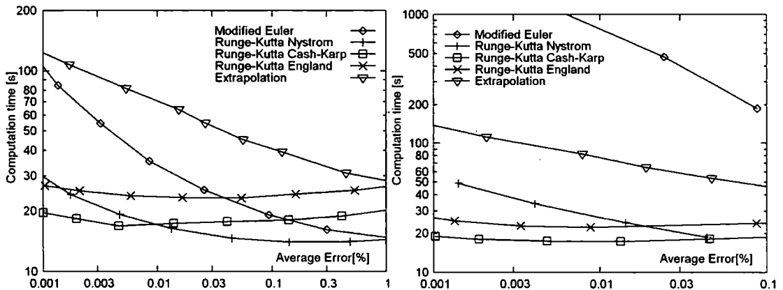
Figure 7.9. Computation times versus average error for best Runge-Kutta schemes and extrapolation method with EPS control (left) and EPUS error control (right).
