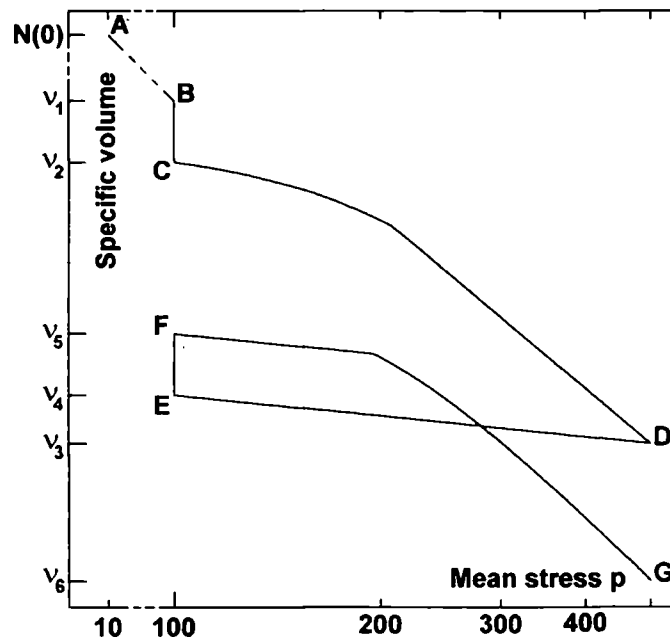
Figure 5.1. Stress path, as calculated in the example
