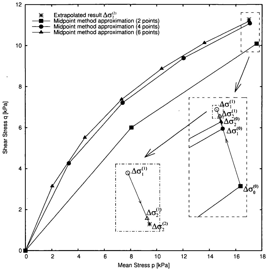
Figure 6.2. Extrapolation method: stress increments integrated with 2, 4 and 6 subincrements ( \Delta\sigma_0^{(0)} , \Delta\sigma_1^{(0)} and \Delta\sigma_2^{(0)} ) are extrapolated to obtain \Delta\sigma_1^{(1)} and \Delta\sigma_2^{(1)} . Those stress increments are used to obtain final, most accurate stress increment \Delta\sigma_2^{(2)} .
