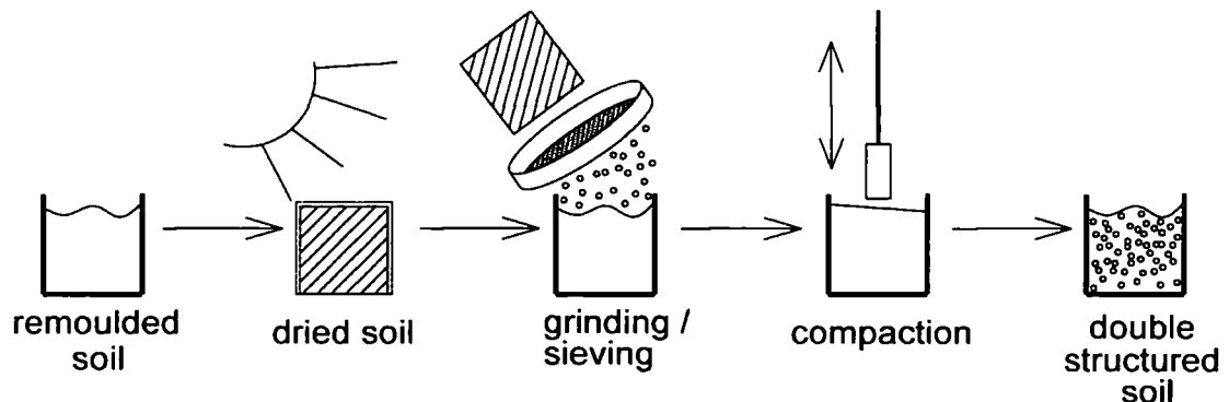
Figure 2.14. Typical sample preparation for unsaturated soil testing resulting in double structured soil.
