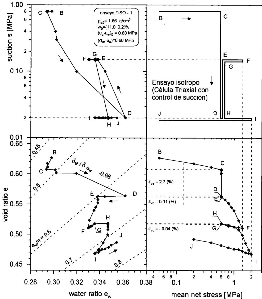
Figure 2.6. Mean net stress loading of a compacted sample with changes in suction (after Barrera 2002).
