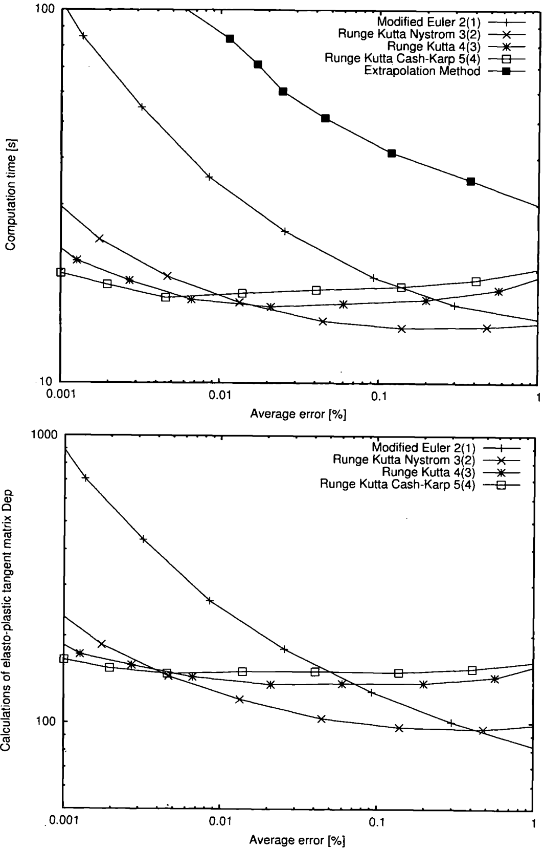
Figure 7.10. Comparison of efficiency for best Runge-Kutta schemes of order two, three, four and five and extrapolation method when coupled with EPS error control.
