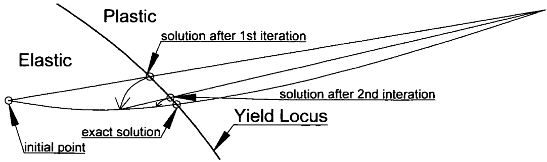
Figure 6.3. Graphical illustration of the first two iterations of Pegasus algorithm
