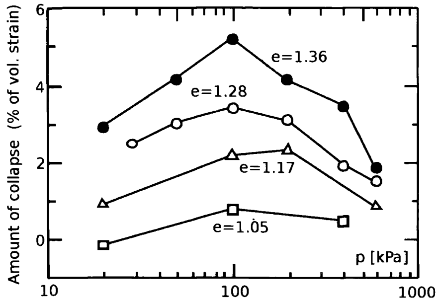
Figure 2.5. Amount of collapse for compacted soil samples to different initial void ratio. The relative amount of collapse decreases in high mean net stresses (after Sun et al. 2007b).
