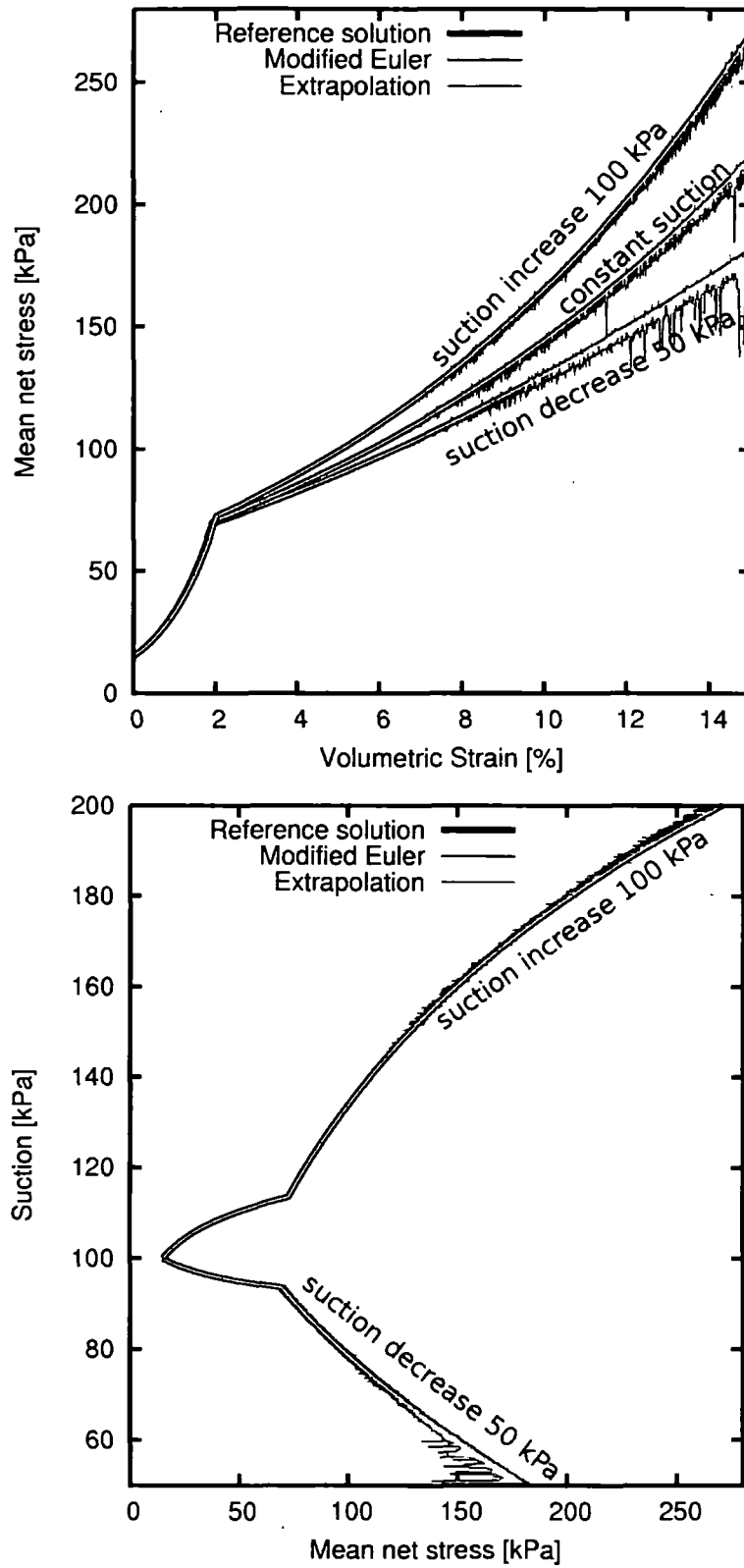
Figure 7.1. Isotropic loading at variable suction starting from an initial isotropic stress state: mean net stress versus volumetric strain (top) and suction versus mean net stress (bottom)
