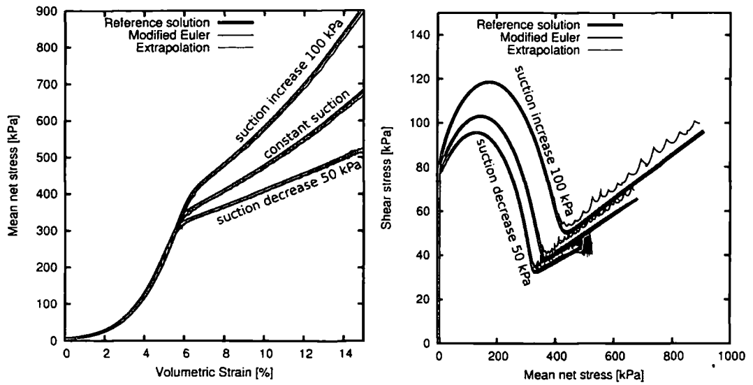
Figure 7.4. Oedometric loading at variable suction for heavily overconsolidated soil with associated flow rule: mean net stress versus volumetric strain (left) and shear stress versus mean net stress (right)
