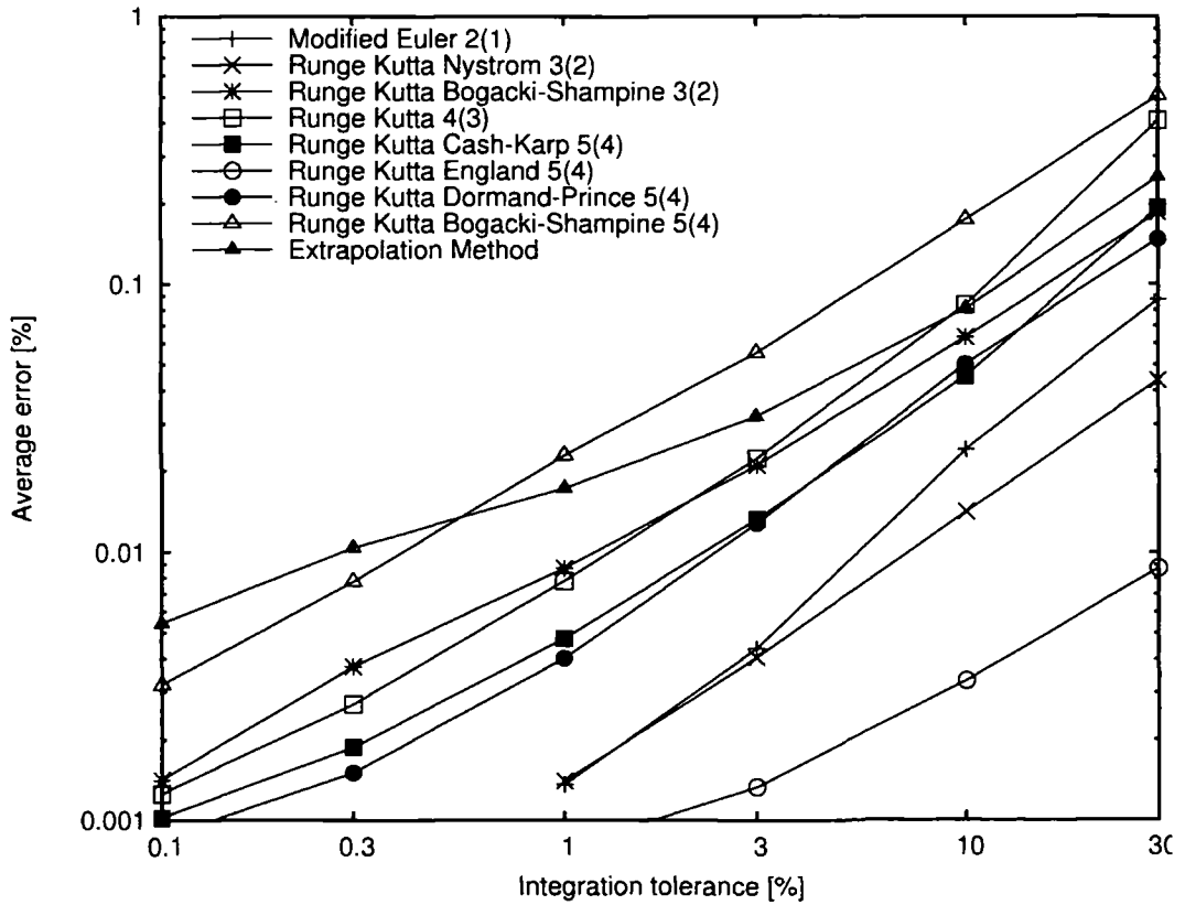
Figure 7.15. Average error vs tolerance for Runge-Kutta methods and extrapolation method with EPS error control method (top) or EPUS error control method (bottom).
