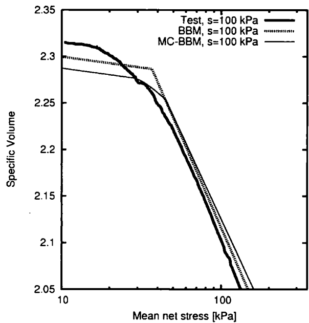
Figure 5.9. Multi-cell enhanced BBM (MC-BBM) and BBM approximation of experimental data. Data after Sharma (1998).
