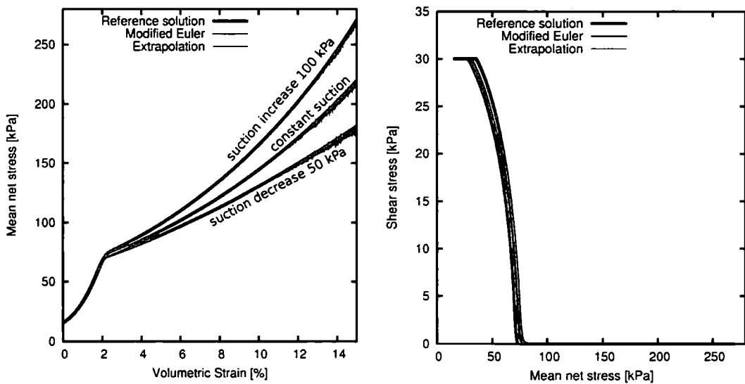
Figure 7.3. Isotropic loading at variable suction starting from an initial non-isotropic stress state with non-associated flow rule: mean net stress versus volumetric strain (left) and shear stress versus mean net stress (right).
