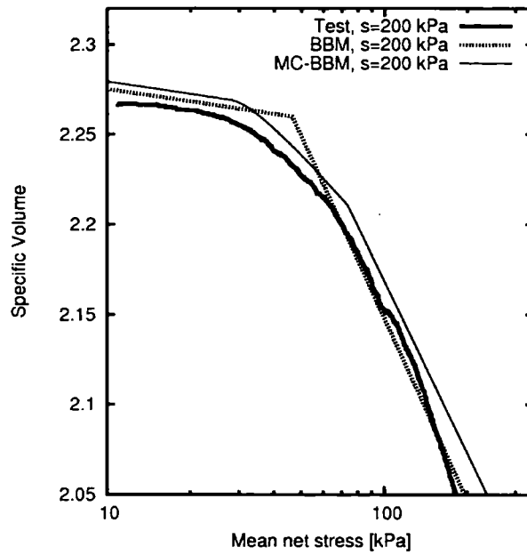
Figure 5.10. Multi-cell enhanced BBM (MC-BBM) and BBM approximation of experimental data. Data after Sharma (1998).
