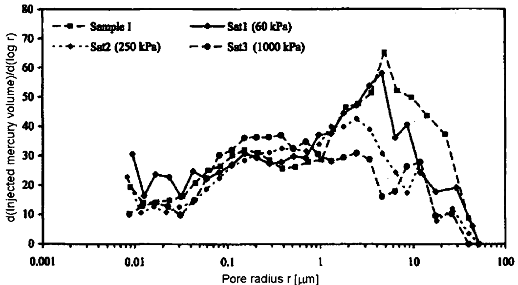
Figure 2.15. Evolution of soil fabric under mechanical loading in saturated state. Values in brackets indicate maximum mean stress applied (after Cuisinier and Laloui 2004)
