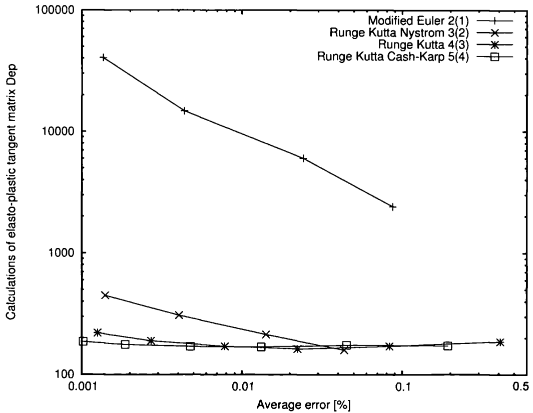
Figure 7.11. Comparison of efficiency for best Runge-Kutta schemes of order two, three, four and five and extrapolation method when coupled with EPUS error control.
