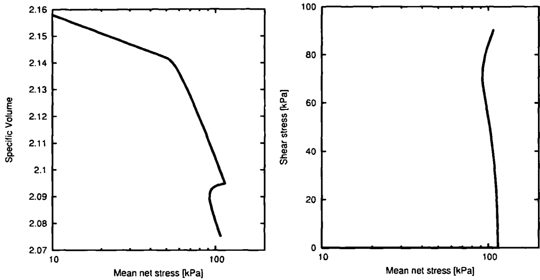
Figure 6.5. Stress integration: initial increment of 3% volumetric strain (as in isotropic loading) followed by 1% of \epsilon_{11} increment (as in oedometric loading). Evolution of mean net stress versus specific volume (left) and mean net stress versus shear stress (right).
