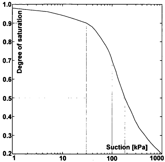
Figure 5.2. Water retention curve
