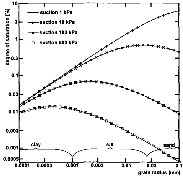
Figure 3.4. Degree of saturation due to menisci. Simple cubic packing assumed
