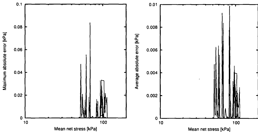
Figure 6.6. Error in integration shown in Fig. 6.5 (left) due to multi-cell enhancement. Maximum error among all stress components in all cells (measured against averaged stress over all the cells, left) and average error of non-zero stress components (measured against averaged stress over all the cells, right).
