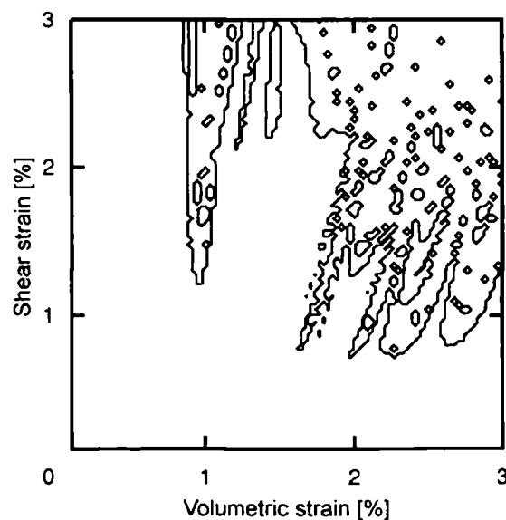
Figure 7.18. Shaded areas of the map indicate non – convergence of the general implicit algorithm. Tests were done for BBM with parameters for Lower Cromer till (Alonso 1990). The initial stress state was p=500 kPa q=0 , initial suction 800 kPa and suction increment -300 kPa, constant for each strain increment (volumetric and shear strain increment were as indicated on the axes). Data obtained by Solowski and Hofmann.
