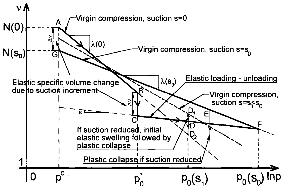
Figure 4.2. Behaviour of soil on isotropic stress paths, as predicted by the BBM.
