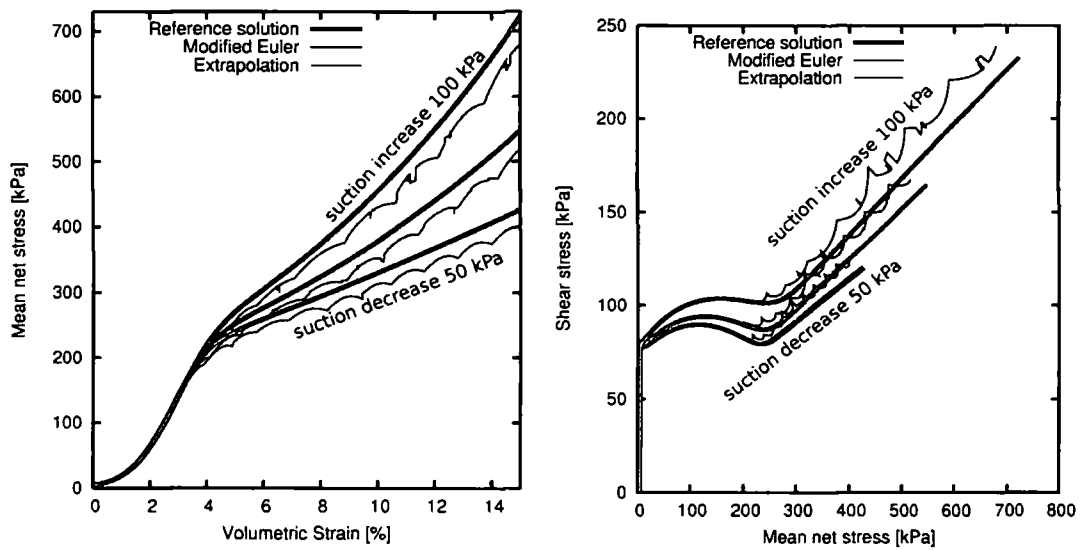
Figure 7.5. Oedometric loading at variable suction for heavily overconsolidated soil with non-associated flow rule: mean net stress versus volumetric strain (left) and shear stress versus mean net stress (right)
