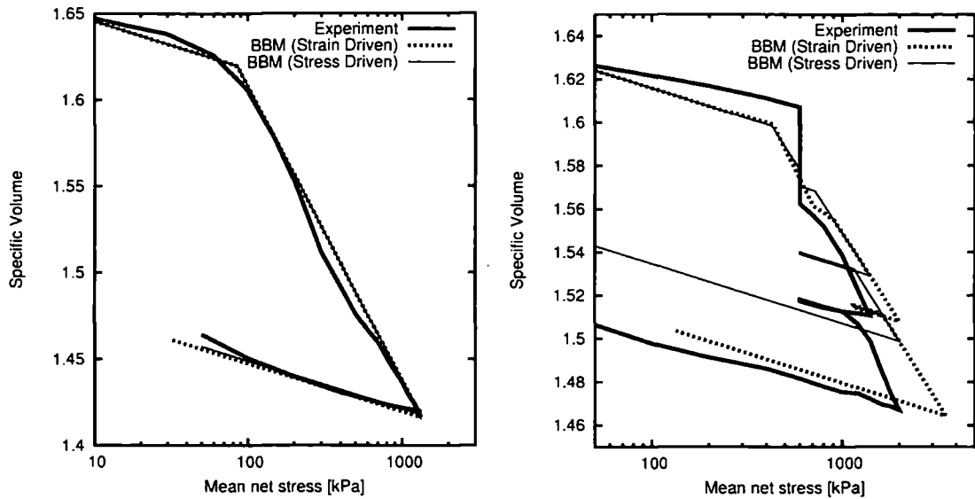
Figure 4.3. Comparison for the saturated SAT-1 (left) and unsaturated TISO-1 (right) isotropic tests. In the figure laboratory data and predictions of the BBM (both strain and stress driven) are given.
