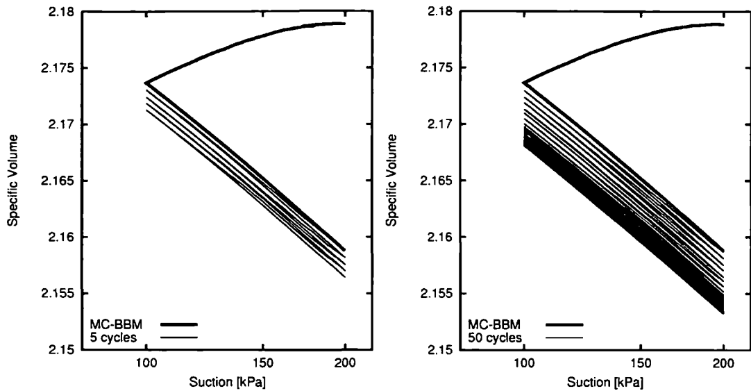
Figure 5.13. Random multi-cell enhanced BBM (RMC-BBM) with five (left) and fifty (right) wetting and drying cycles. The MC-BBM solution is equal to RMC-BBM with one cycle.
