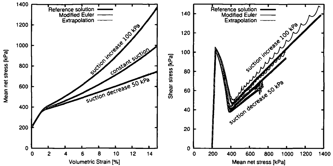
Figure 7.6. Oedometric loading at variable suction for slightly overconsolidated soil with associated flow rule: mean net stress versus volumetric strain (left) and shear stress versus mean net stress (right)
