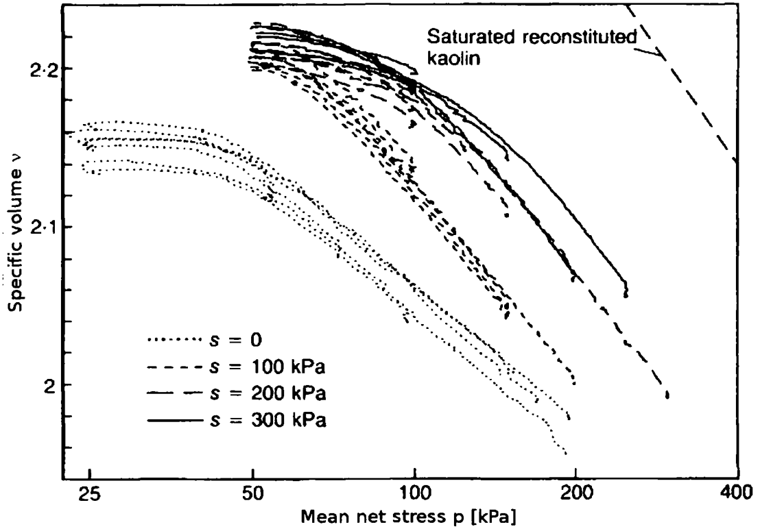
Figure 2.3. Isotropic compression tests for suctions 0, 100, 200 and 300 kPa (after Wheeler and Sivakumar 1995). Note that virgin compression lines corresponding to the reconstituted saturated kaolin and kaolin with non-zero suction have very similar slopes.
