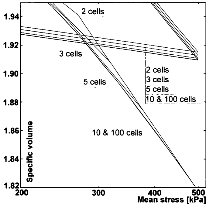
Figure 5.5. Influence of number of cells used in simulation – enlarged detail from Figure 5.4. Comparison between simulations using 2, 3, 5, 10 and 100 cells.
