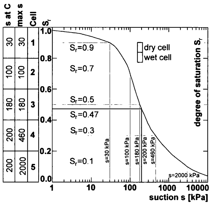
Figure 5.3. Illustration of suction distribution within cells after drying to s=200 kPa (Fig. 5.1, point C). A cell is assumed to be dry when its S_r < 0.5 .
