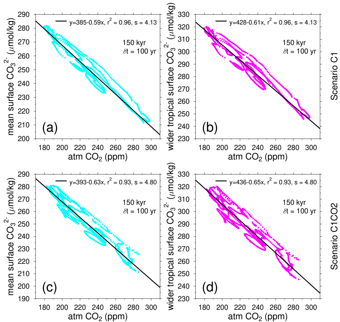
Figure S6. Scatter plots between atmospheric CO 2 and surface ocean CO 3 2- (a,c: global mean; b,d: wider tropics only) in scenarios (a,b) C1 and (c,d) C1CO2 for the last 150 kyr of the simulations. The root-mean-square-error is depicted by s .
