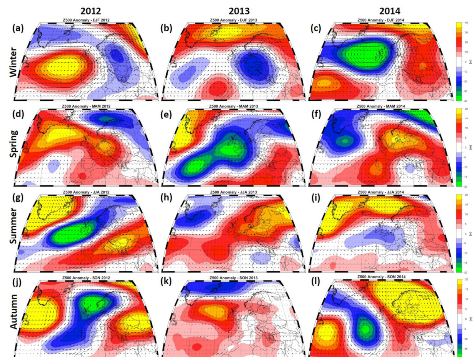
Figure 8. The seasonal geopotential height at 500 mb (Z500) anomalies over the period of January 2012 to December 2014. The anomalies are computed relative to the climatological period 1971–2000. Units: m.
