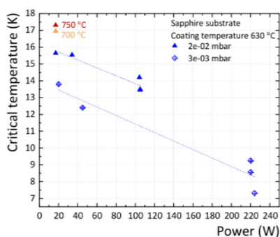
Figure 4: Dependence of the critical temperature of the Nb 3 Sn films on the cathode power. The films on sapphire substrate show trends with cathode power, coating pressure and coating temperature.
