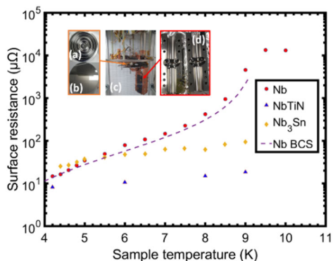
Figure 9: An example of surface resistance as a function of temperature for a planar Nb/Cu and NbTiN/Cu samples. Inset: (a) the choke cavity, (b) Nb/Cu planar sample, (c) RF facility, (d) a split cavity.
