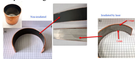
Figure 7: Samples formed from cylindrical Copper tube with Nb film: (a) non-irradiated; (b) irradiated in Ar chamber by ns laser radiation.
