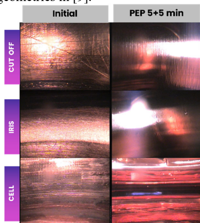
Figure 2: Internal surface inspection of a Cu 6 GHz cavity before (on the left) and after (on the right) PEP treatment.
