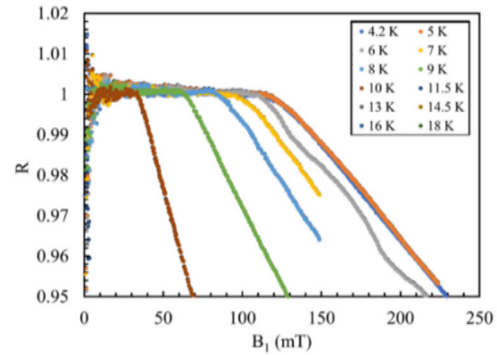
Figure 8: An example of parameter R(B_1, T_s) for Nb 3 Sn.
