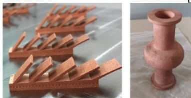
Figure 1: On the left Cu AM printability test of overhang surfaces. On the right the first Cu 6 GHz AM prototype.
