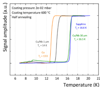
Figure 5: Superconducting transition curves of samples deposited at 600 °C. The Nb 3 Sn coated onto a thick Nb barrier layer shows same T c as sapphire substrate ones.
