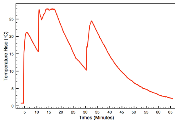
Figure 3. Hot Water Outlet Pipe Temperature Rise
