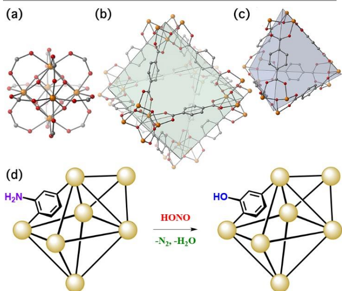
Fig. 1 (a) The \text{Zr}_6\text{O}_4(\text{OH})_4^{12+} node of UiO-66 coordinated to 12 carboxylate anions. (b) The octahedral pore of UiO-66. (c) The tetrahedral pore of UiO-66. (d) Schematic
