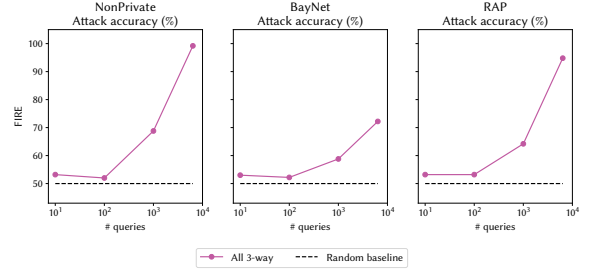
Figure 15: Comparison of attack accuracy of \text{Adv}_{recon} when uses varying number of queries for synthetic data size, m = 10^6
