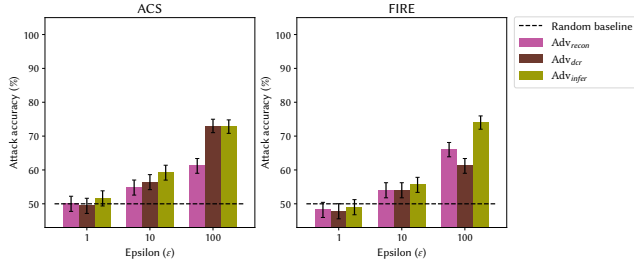
Figure 7: Attack accuracy of \text{Adv}_{\text{recon}} , \text{Adv}_{\text{dcr}} and \text{Adv}_{\text{infer}} as a function of privacy parameter \epsilon for PrivBayes synthetic data of size m = 10^6
