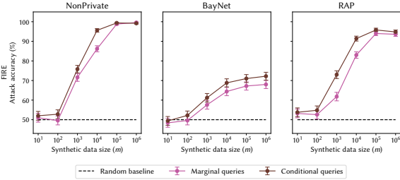
Figure 14: Comparison of attack accuracy of \text{Adv}_{recon} when using conditional queries compared to marginal queries.
