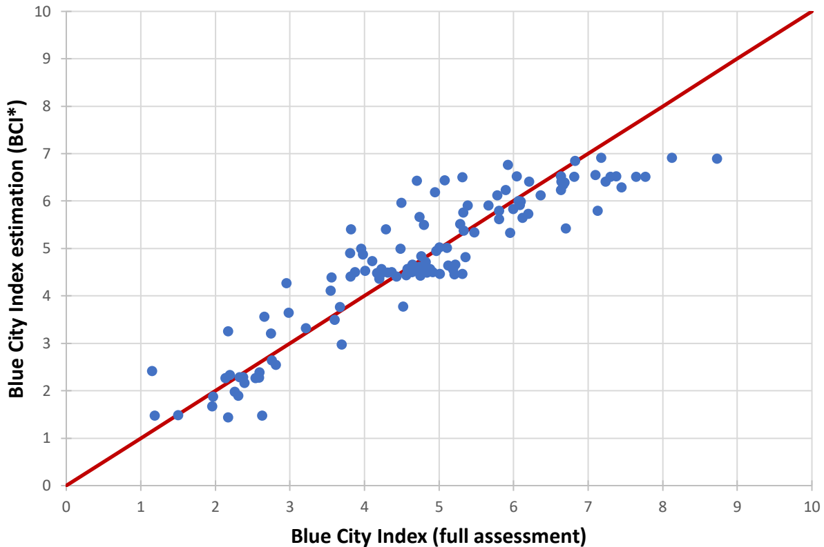
Fig. 3. Three-variable BCI* estimation model based on CBF and TPF, as provided in equation 1: BCI^* = 4.25 - 0.396*TPF21 [Government\ effectiveness] + 0.195*CBF4 [Secondary\ WWT] + 0.111*CBF8 [Energy\ recovery] . The plot shows the estimated BCI*s against the fully assessed BCIs for the combined 48 CBF and TPF indicators. The solid red line represent a full correspondence of the estimated BCI* and the actual BCI ( Y=X ; slope = 1). The applicability domain of the estimation model covers the BCI range of 1 to 6.5 as for BCI values > 6.5 a departure from linearity can be observed.
